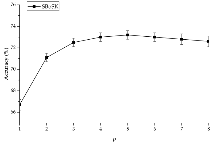
Figure 3.18: Classification accuracy w.r.t. different maximum considered subpath lengths P . SBoSK is computed on the Strasbourg Spot-4 image with D = 4096 .
