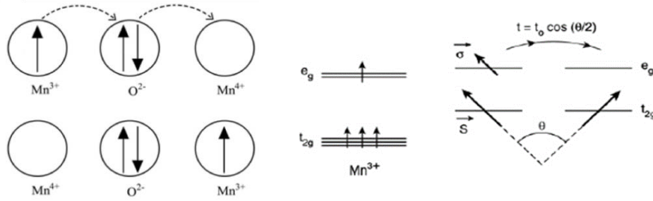
Figure 2.6: Transfer of electron from Mn 3+ to Mn 4+ via O – 2p orbital, and angle dependent transfer of e g electron between ‘i’ and ‘j’ sites, respectively [25].
