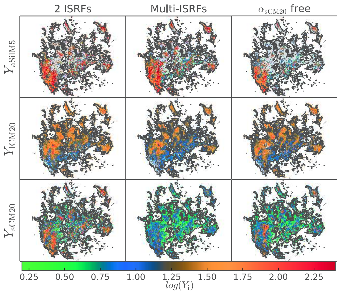
Figure 7.2: Parameter maps in the LMC from THEMIS fits of Y_{aSiM5} , Y_{1CM20} , and Y_{sCM20} (first, second, and third rows, respectively) for the two-ISRF, multi-ISRF, and \alpha_{sCM20} free (first, second, and third column) models.
