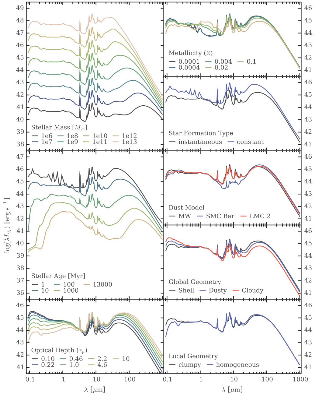
Figure 11.3: A few spectra from DIRTY, representing the variations in each parameter space.
