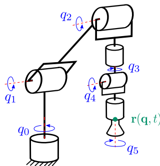
Figure 1.23: Robot joints \mathbf{q} for a 6-DOF robot, and the pose \mathbf{r} of the end-effector.
