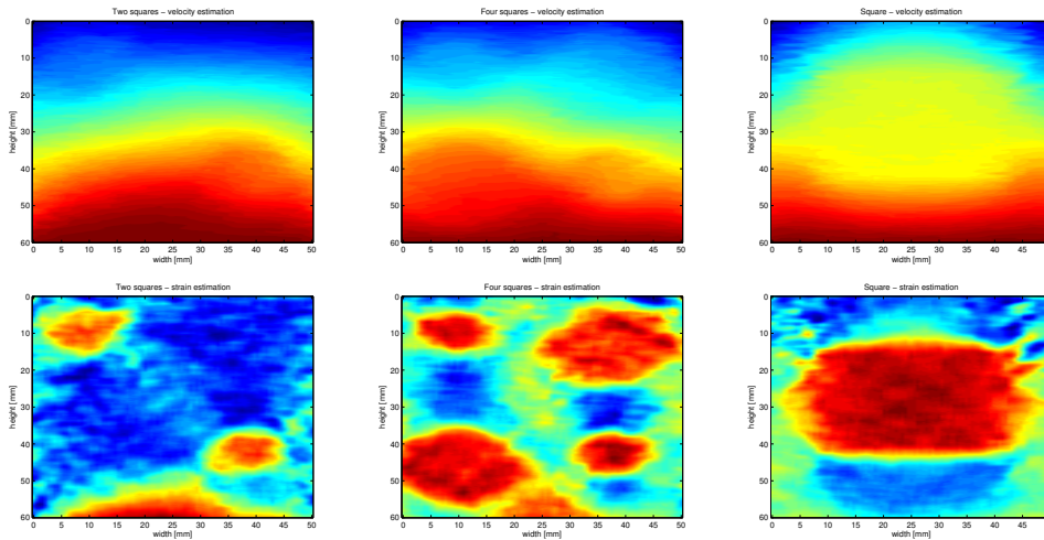
Figure 2.18: Results using simulation data from FEM+FIELD II.
