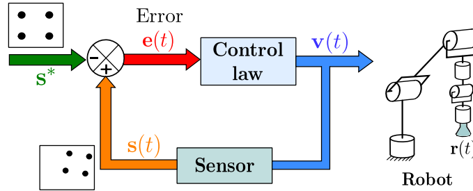
Figure 1.21: Visual servoing closed-loop.
