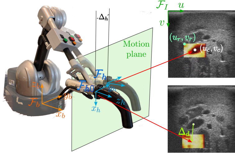
Figure 4.10: Handler displacement into the ultrasound image.
