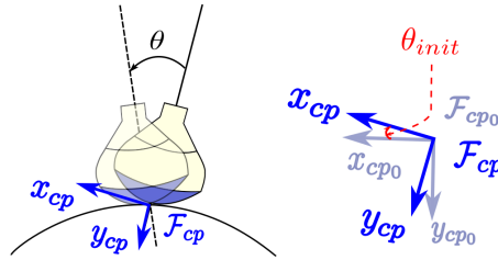
Figure 2.26: Probe orientation.
