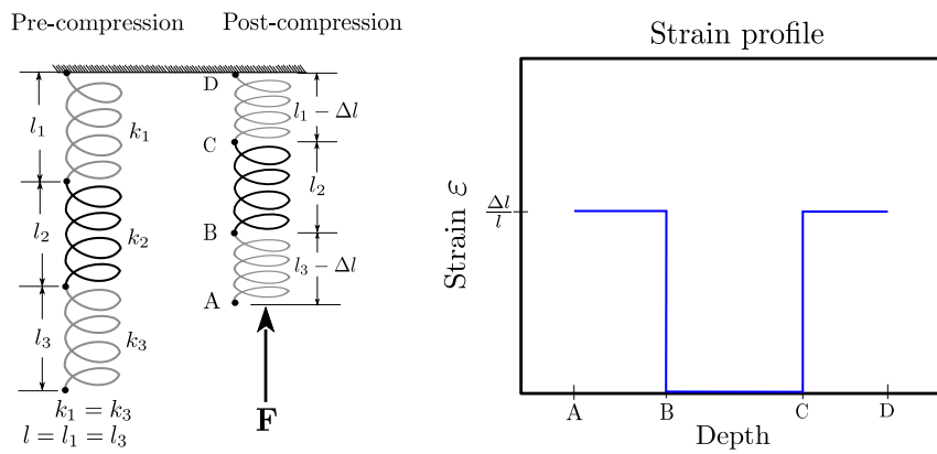
Figure 1.11: Strain profile for three consecutive springs. Springs 1 and 3 have the same length l and stiffness value k in the pre-compression state.
