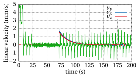
(c) Linear velocities
