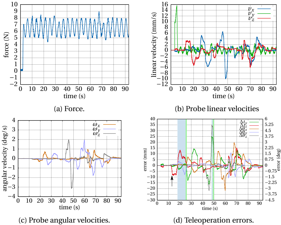
Figure 4.17: Measured force, velocities and errors in the teleoperation system.
