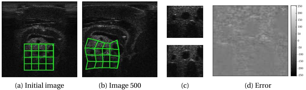
Figure 3.6: Example of the performance in dense FFD tracking. (a) initial image ( i = 0 ) of an image sequence (green rectangle is the region to be tracked). (b) last image ( i = 500 ) in the sequence. (c) template image from (a) at top and warped image from (b) at bottom. (d) error image computed from \hat{\mathbf{I}}_c(w(\mathbf{x}, \mathbf{p})) - \mathbf{I}_t(\mathbf{x}) .
