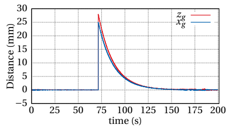
(b) Centering error e_t
