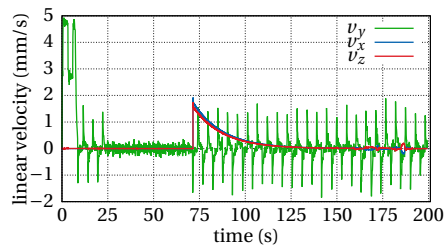
(c) Linear velocities
