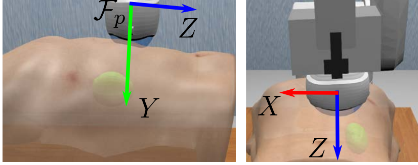
Figure 2.24: Axes for the frame \mathcal{F}_p (frame of the ultrasound probe). Lateral and top views of the probe in contact with a virtual human torso are shown in left and right images, respectively. A target, in green, is placed inside of the torso to relate the two views.
