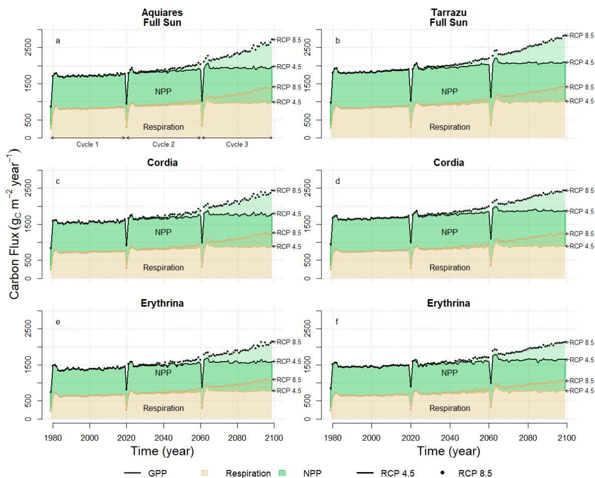
352 353 Figure 25. Climate change impacts on GPP and cumulated respiration and NPP according to Representative Concentration 354 Pathways (RCP 4.5 and RCP 8.5); location (left: Aquiares, right: Tarrazu) and current reference management: coffee grown 355 in monoculture (a,b) or in agroforestry systems under Cordia alliodora (c,d) or Erythrina poeppigiana (e,f).
