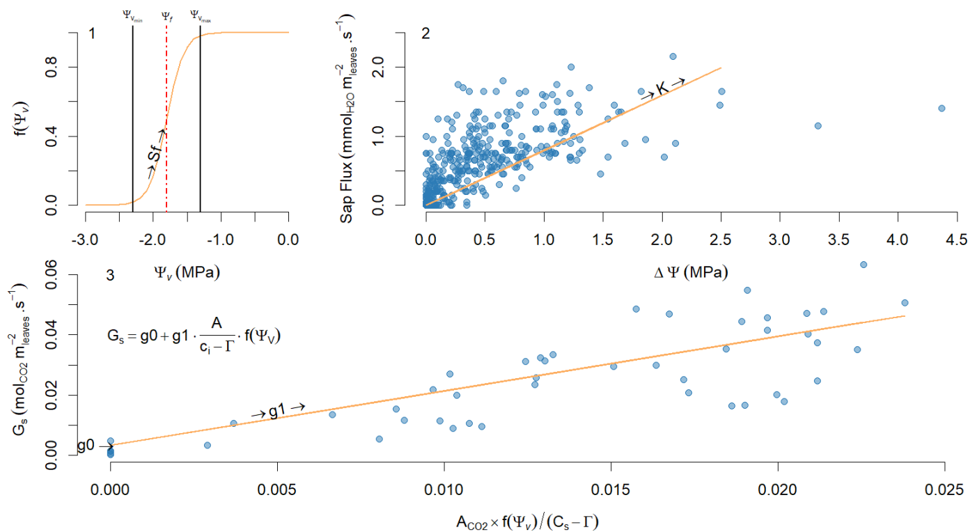
Figure A1. Tuzet et al. (2003) conductance model parameterization using 6 Coffea sprouts sap fluxes and leaf water potential. (1) Sf and \Psi_f parameters fit using data \Psi_{min} and \Psi_{max} data from (Dauzat et al., 2001) ; (2) Root-to-leaf plant conductivity ( K ) and (3) G_0 and G_1 parameters fitting.
