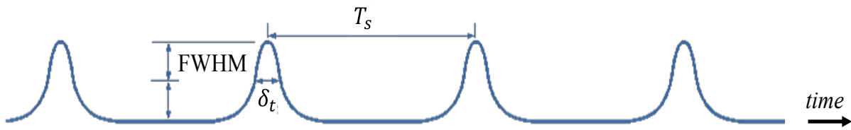
Figure 1.11: Pulse train of period T_s formed by pulses of width \delta_t measured at FWHM.
