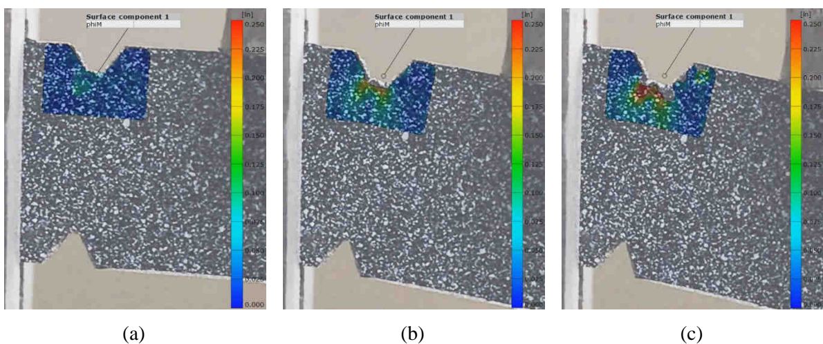
Figure 89 - Digital Image Correlation on tensile tests of epoxy resin (a) beginning of the test, (b) during the test and (c) at the failure initiation
