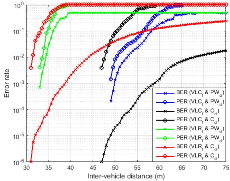
FIGURE 4.26: BER and PER evolution against the inter-vehicle distance by steps of 50 cm and combination of ‘VLC filtering’ (VLC f ) or ‘VLR filtering’ (VLR f ) with pulse width decoding (PW d ) or clock decoding (C d ).
