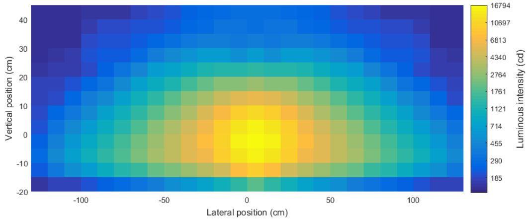
FIGURE 2.17: Spatial distribution of the luminous intensity of a headlamp driven by a current of 600 mA, when projected on a vertical plane at 4.5 m. The point of origin is the point of maximum luminous intensity 50 L.
