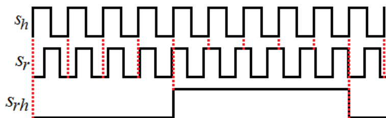
FIGURE 3.17: Heterodyning of a signal s_r by undersampling with a non-synchronized clock s_h when r = 10 .
