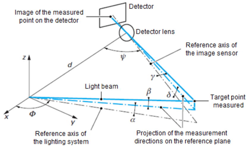
FIGURE 3.1: Working principles of triangulation, with \alpha , \beta and \Phi the angles of emission, \delta , \gamma and \psi the angles of incidence and d the distance between the emitter and the receiver [126].
