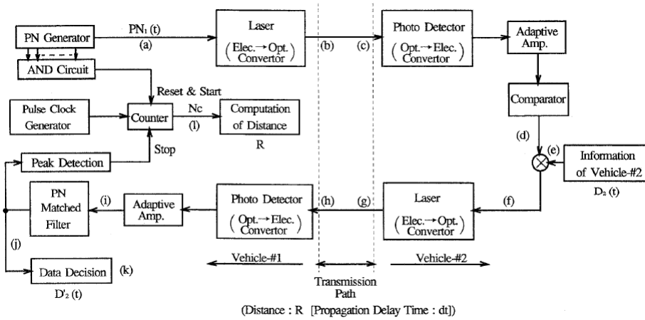
FIGURE 2.25: Block diagram of the boomerang system [110].
