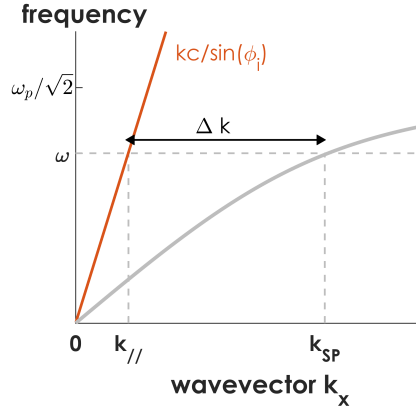
Figure 1.4: Matching the wavevector of the external EM wave and the SP requires to compensate \Delta k .
