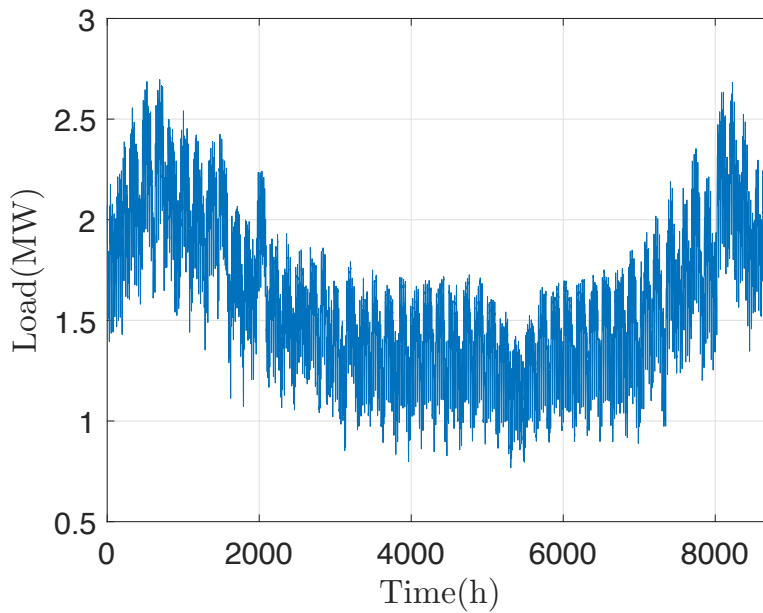
FIGURE 2.3: Ouessant approximated load variations for the year 2014.
