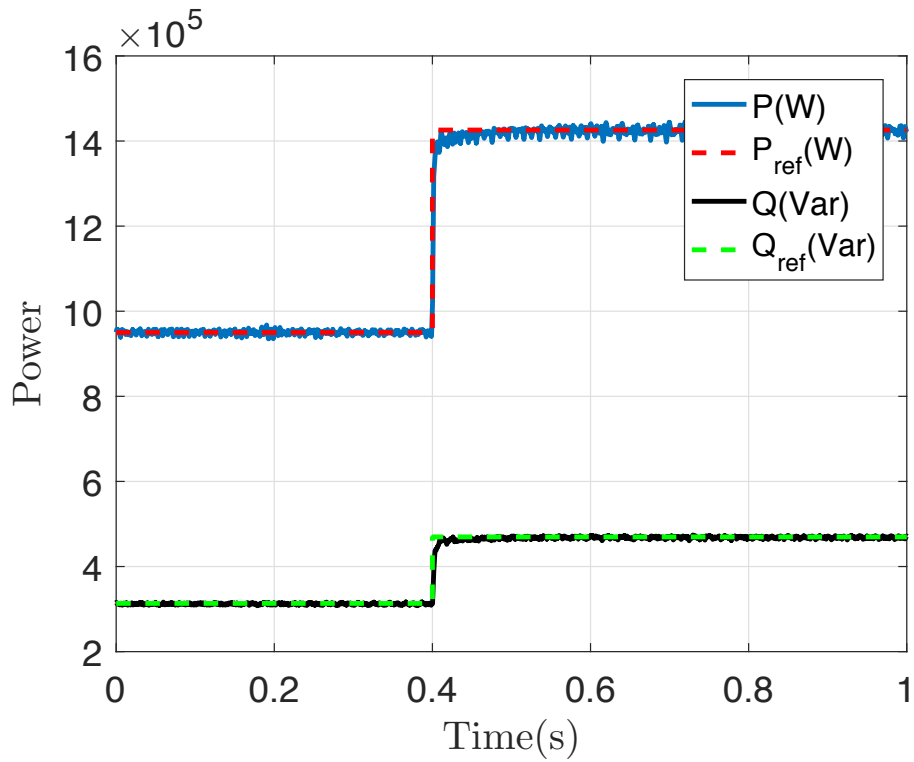
FIGURE 4.25: Power variations for the VSG control case.
