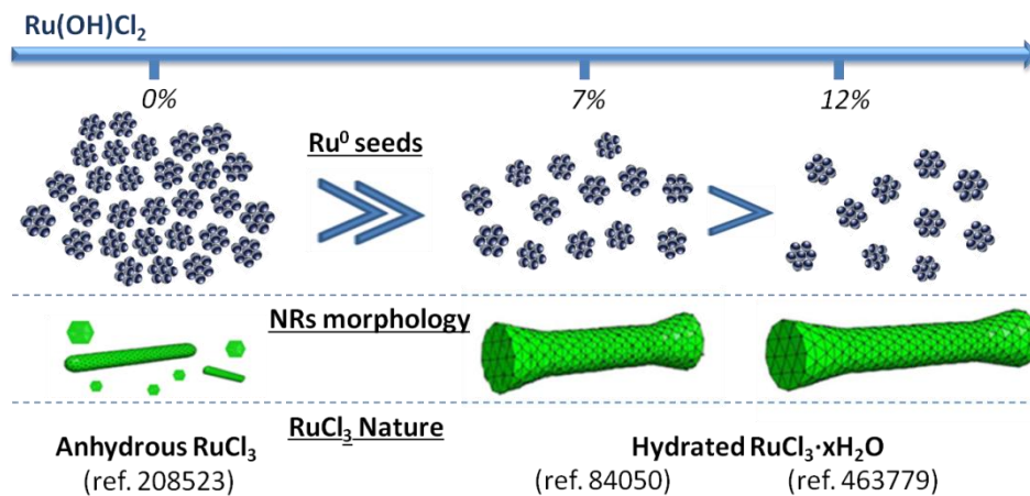
Figure II- 36 Suggested effect of the \text{Ru}(\text{OH})\text{Cl}_2 content on the \text{Ru}^0 nucleation rate and the nanorods' morphology.
