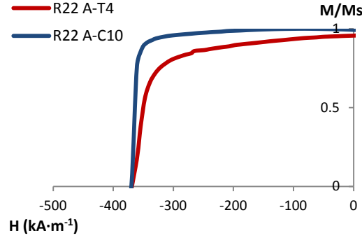
Figure III- 19 Second quadrant of the M(H) loops of the nanorod assemblies R_{22}A_{T4} and R_{22}A_{C1} .
