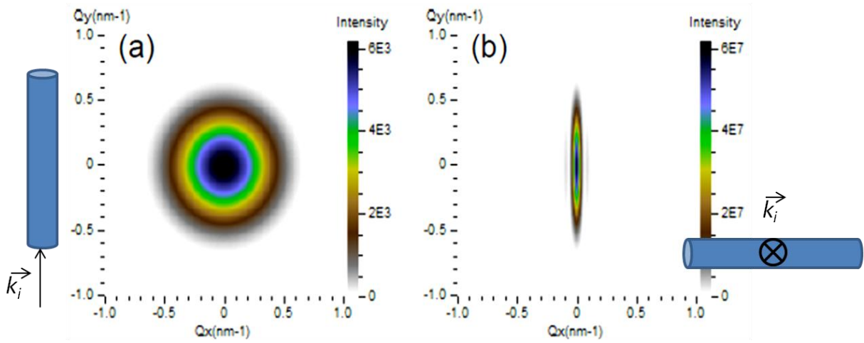
Figure IV- 2 Simulations of the factor V_p^2P(q) performed via the spectraprocessor software for a nanowire with d_m= 10 \text{ nm} and L_m= 100 \text{ nm} depending on its orientation to the incident beam (a) the rod long axis and \vec{k}_i are parallel to z ; (b) the rod long axis is in the (x,y) plane and parallel to x while \vec{k}_i is along z [6].
