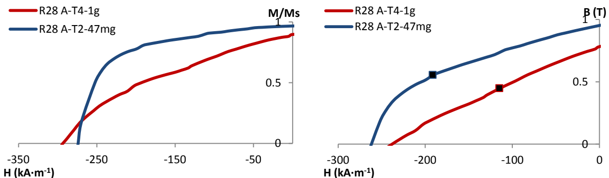
Figure III- 13 M(H) loop (left) and second quadrant of the corresponding B(H) loops (right) of the assemblies R_{28}A_{T4-1\text{g}} and R_{28}A_{T2-47\text{mg}} .
