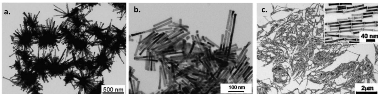
Figure II- 10 TEM images of Co particles obtained by reducing the following cobalt carboxylates: a) sea-urchin like particles from cobalt acetate; b) nanorods with L_m= 133 nm and D_m= 13 nm from cobalt caprate(C9) and c) nanorods with L_m= 99 nm and D_m= 15 nm from cobalt laurate (C12) [18].
