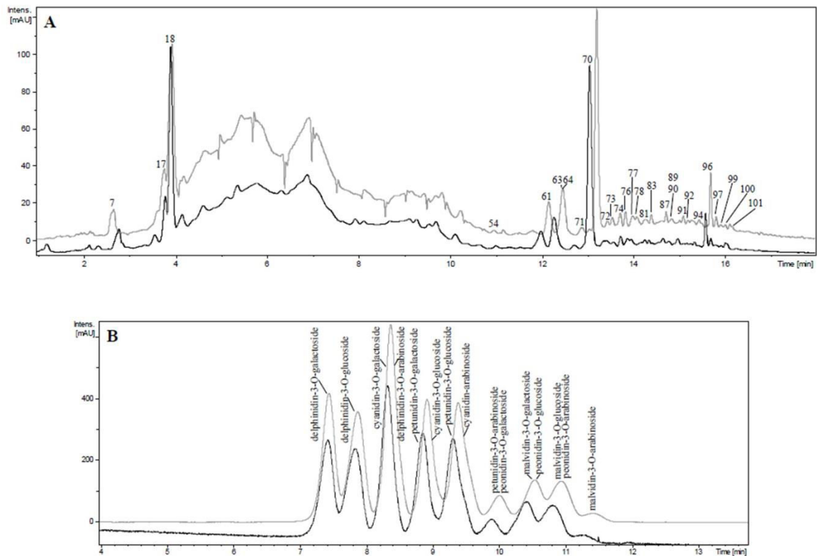
Fig. 4. Chromatographic profile at 280 nm (A) and at 520 nm (B) of aqueous (black) and ethanolic (grey) fruit extracts.
