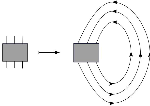
Figure 1.6 – The closure operation.
