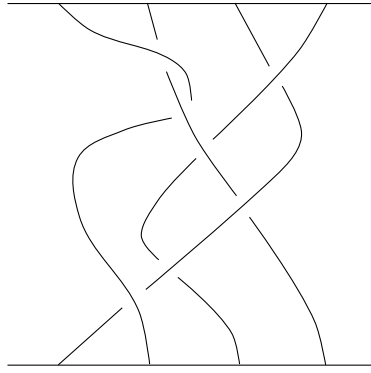
Figure 1.4 – Braid \sigma_1\sigma_3^{-1}\sigma_1\sigma_2\sigma_3^{-1}\sigma_2^{-1}\sigma_1 .
