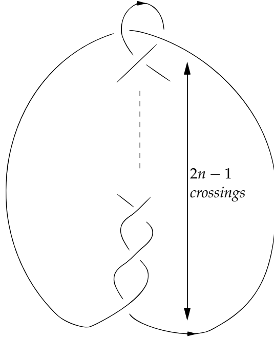
Figure 4.5 – Twist knot K_n .
