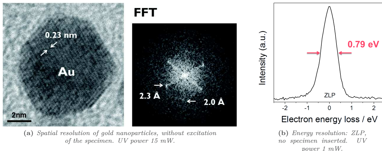
Figure 4.5: Resolution tests of the photoelectron beam in stroboscopic operation mode. The UV laser was operated at a repetition rate of 2 MHz.
