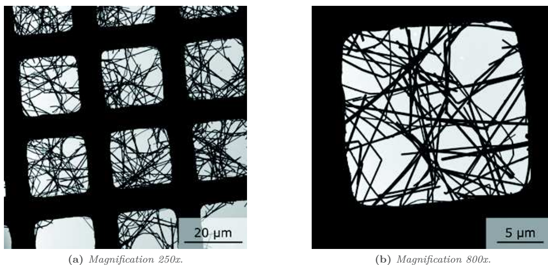
Figure 4.6: TEM images of the PINEM test sample containing silver needles deposited on a copper grid.
