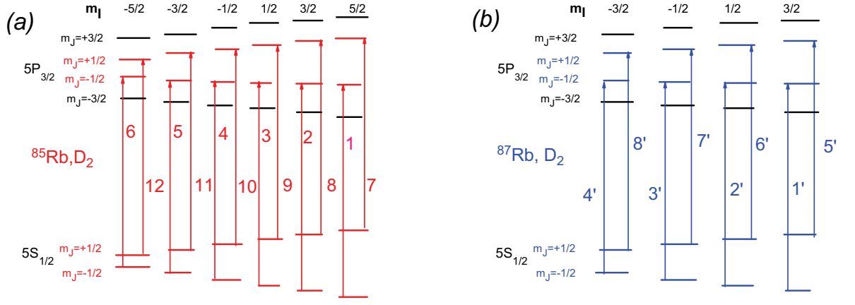
(a) The diagram of ^{85}\text{Rb} transitions. According to the selection rules for the case of -polarized radiation \Delta m_J = 0 and \Delta m_I = 0 , there are 12 transitions (labeled as 1-12)
