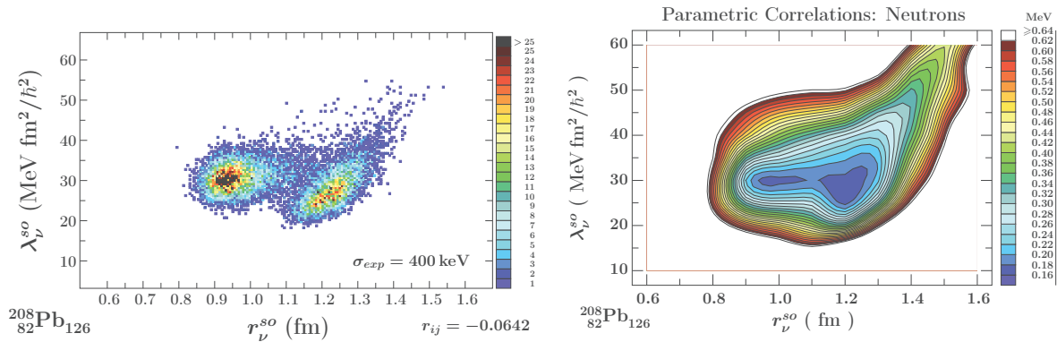
Figure 4.35 – Parametric correlation between spin-orbit radius and spin-orbit strength for the neutrons. Left panel shows realistic Monte Carlo simulations with the colour scale indicating the concentration of data points. Right panel: Projection of the r.m.s.-deviations onto the two dimensional plane with the colour scale representing the r.m.s.-values.
