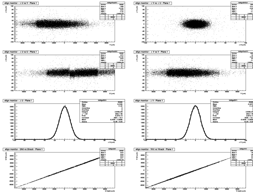
Figure 3.5: Alignment monitoring plots for a DUT (MIMOSA-28) using SALAT modules as references. The misalignment is due to the SALAT system.
