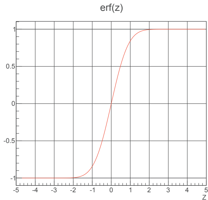
Figure 4.7: Error Function
