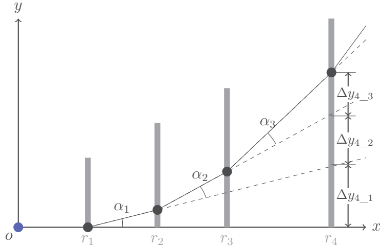
Figure 4.1: Multiple scattering in several layers of a detector
