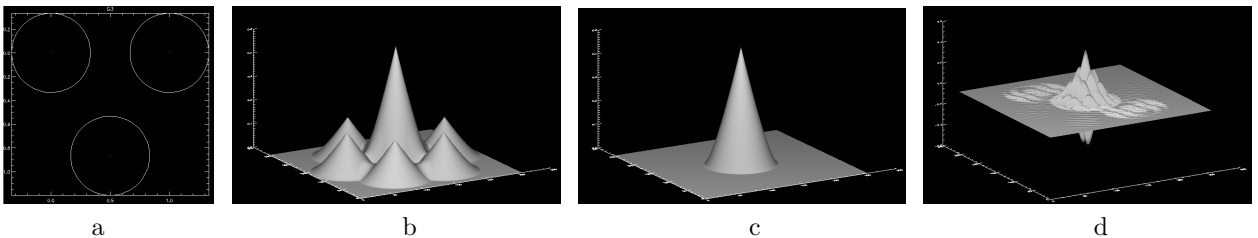
Figure 1. a. Goly 3 pupil configuration ; b. Goly 3 coherent OTF (aligned) ; c. Goly 3 incoherent OTF (aligned) ; d. Goly 3 coherent OTF (large differential tip/tilts between sub-apertures).
