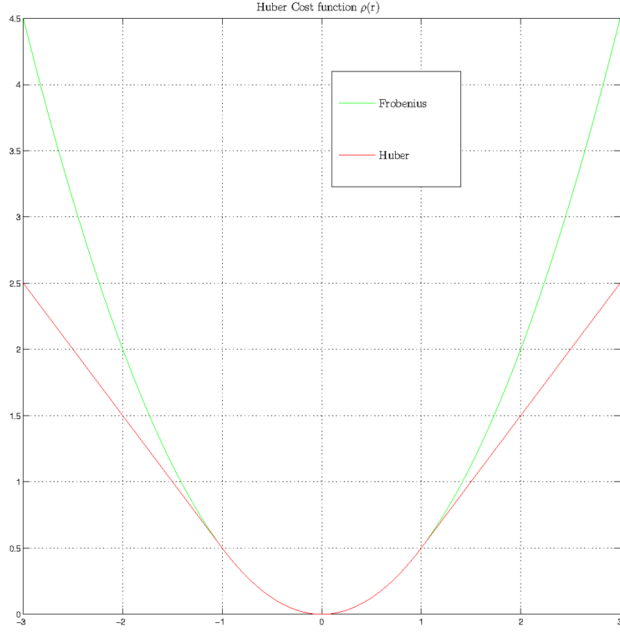
Figure 4.3 – The Huber Cost Function
