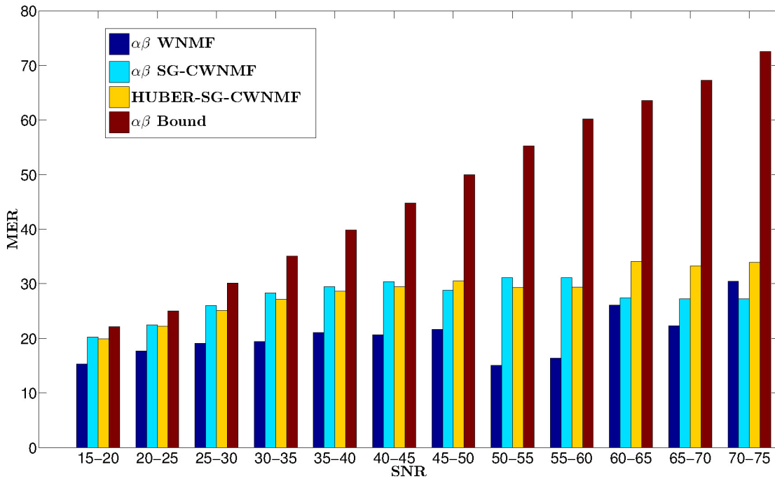
Figure 6.12 – MER versus input SNR . The case with 10 outliers
