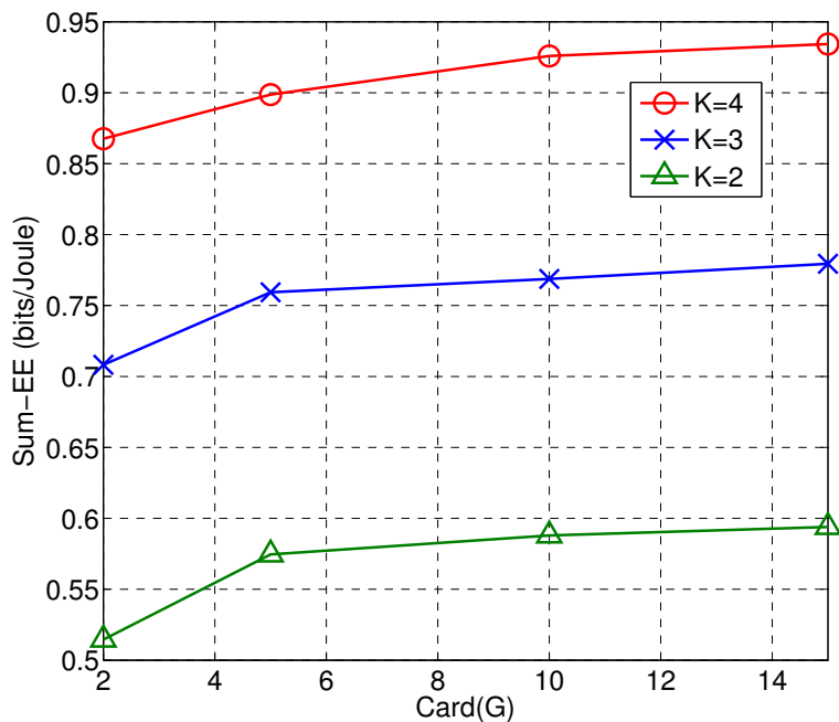
FIGURE 4.8 – The complexity of the algorithm depends highly on the cardinality of G .
