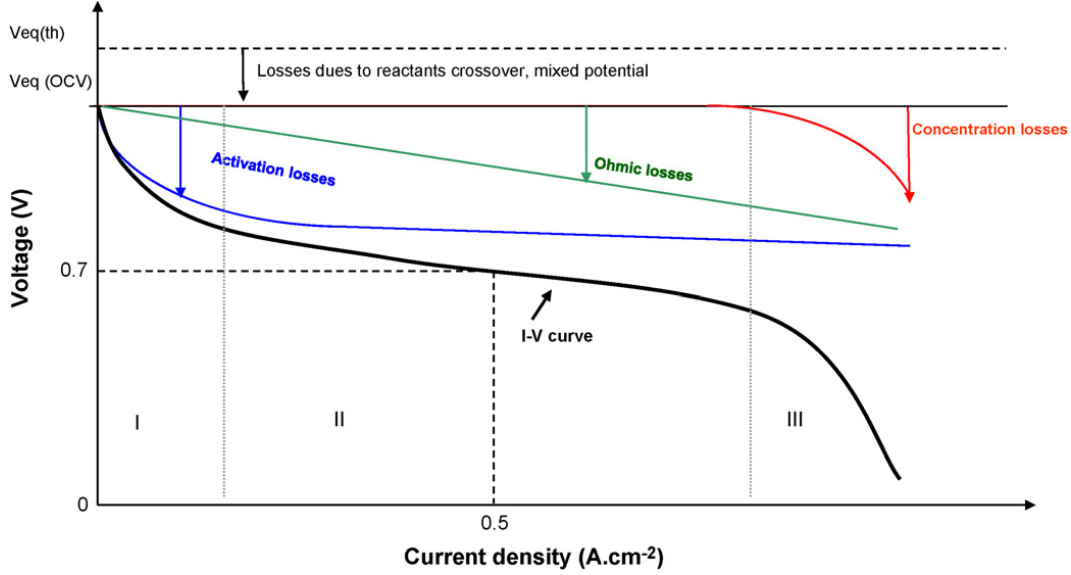
Figure 1.6: Typical polarization curve of PEMFC [24].
