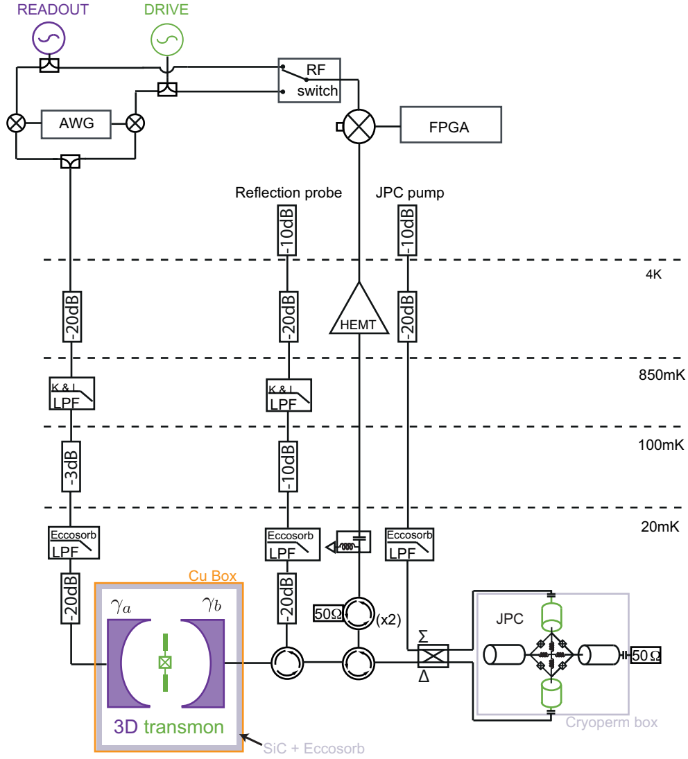
Figure 65: Full schematic of the wiring for the weak value experiment described in Chap. 4.
