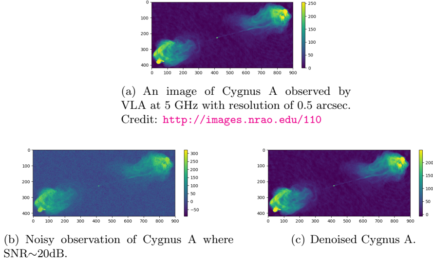
Figure 2.10: Example of sparse denoising: The noisy image is decomposed in starlet wavelet space with four scales and the standard deviation \sigma of the noise is estimated at the finest starlet scale by MAD (all the scales are normalized by the factor of \ell_2 norm of atoms). Then the hard-thresholding operation with threshold 3\sigma is applied on the starlet coefficients (except coefficients of the coarse scale). The final denoised image is reconstructed from the modified starlet coefficients.
