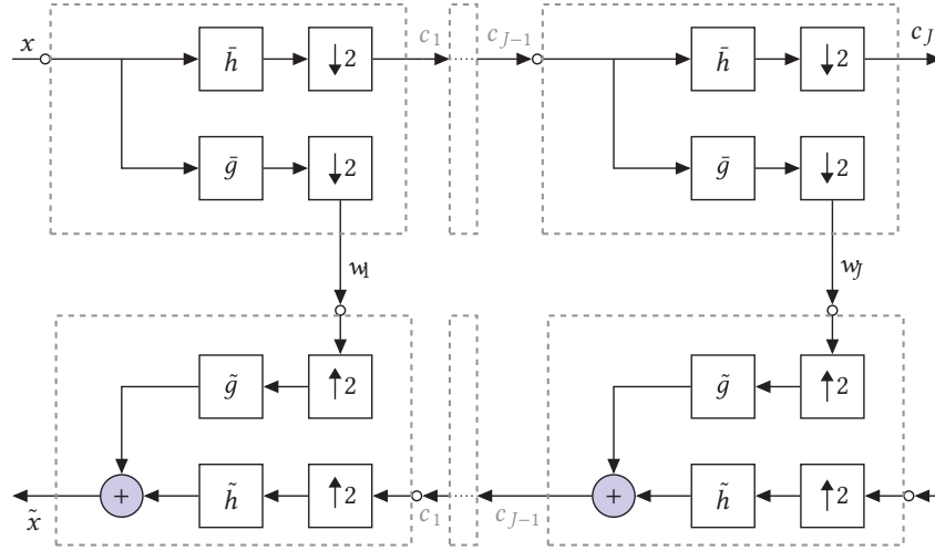
Figure 2.4: Fast pyramidal algorithm for a (bi-)orthogonal wavelet transform. The top represents the scheme of fast decomposition of an input signal x using a pair of filter (h, g) , while the bottom represents the scheme of fast reconstruction using a dual pair of filter (\tilde{h}, \tilde{g})
