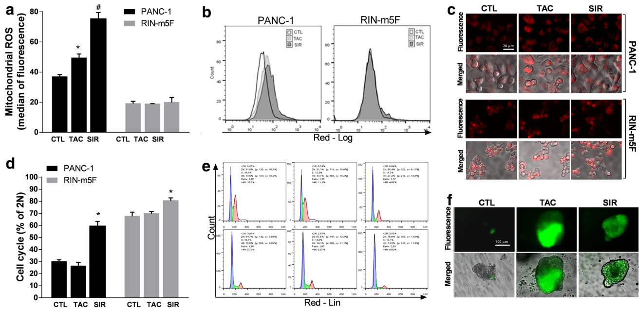
Fig. 4 TAC and SIR impact cell cycle and promote a senescence-like phenotype. a MFI of unfixed cells labeled with MitoSOX™ fluorescent dye assessed by flow cytometry, and b the related histograms. c ROS accumulation after treatment with 100 nM TAC or SIR during 24 h was confirmed by fluorescence microscopy using the MitoSOX™ probe. * p < 0.01 versus untreated cells (CTL), # p < 0.01 versus TAC, n = 3 . d Proportion of cells in G0/1 phase (2 N) after labeling by propidium iodide and red fluorescence acquisition by flow cytometry, following TAC and SIR treatment as above; * p < 0.01 versus untreated (CTL), n = 3 . e Representative histograms of cell populations with diploid DNA in G0/1 (2 N, blue), S (green) and G2
