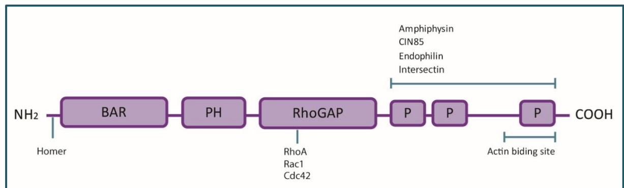
Fig13: Schematic representation of Oligophrenin-1. OPHN1 is a Rho family GTPase activating protein (Rho-GAP) that contains a N-terminal BAR domain, which senses and binds curved membranes and a Pleckstrin Homology (PH) domain, which binds phosphatidylinositol lipids. The catalytic GAP domain inhibits RhoA, Rac1, and Cdc42 in vitro. The C-terminal part, OPHN1 contains an actin-binding site and three Proline-rich sites permitting the interaction with SH3 domain containing proteins including amphiphysinI and II, CIN85, endophilinA1and B2, Homer1 and intersectin1.
