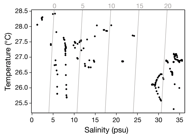
Fig. 6. Temperature–salinity diagram for the 10 individual green turtles Chelonia mydas fitted with a CTD-SRDL tag in 2014. Grey lines and numbers: isopycnal lines and values
