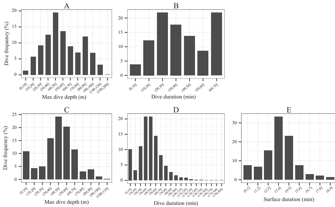
Fig. 4. Histograms of the diving variables recorded by the Argos-linked Fastloc GPS tags (A and B) and the CTD-SRD L tags (C, D and E). Maximum dive depth (A and C, m), dive duration (B and D, min), and post-dive surface interval (E, min) for all individuals.
