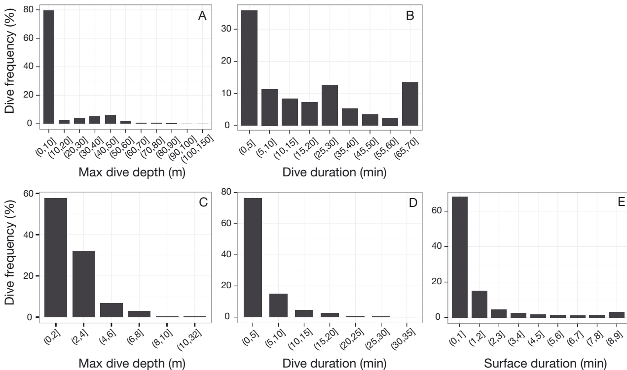
Fig. 3. Diving variables recorded by the (A,B) Argos-Fastloc GPS tags and (C–E) CTD-SRD tags showing maximum dive depth (A,C), dive duration (B,D), and post-dive surface interval (E) for all individual green turtles Chelonia mydas . The bins differ from those described in the 'Materials and methods' section as they were combined for a better visual representation
