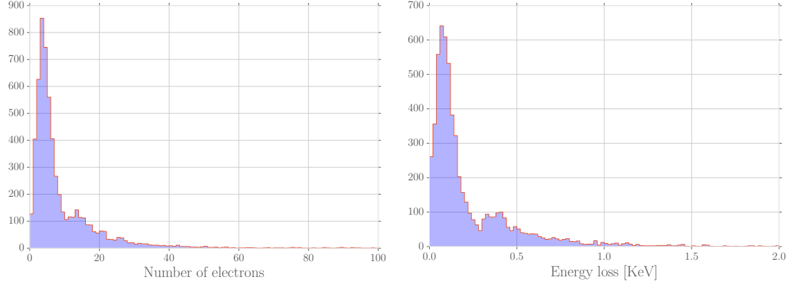
(a) Argon
