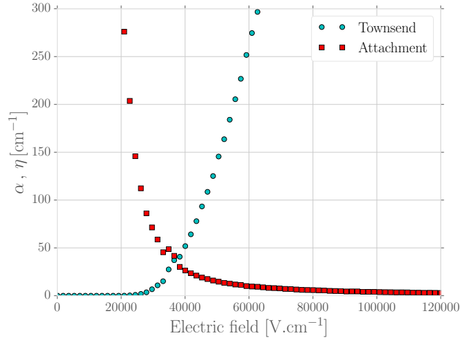
(b) \text{C}_2\text{H}_2\text{F}_4/\text{i-C}_4\text{H}_{10}/\text{SF}_6 96.7%/3%/0.3%
