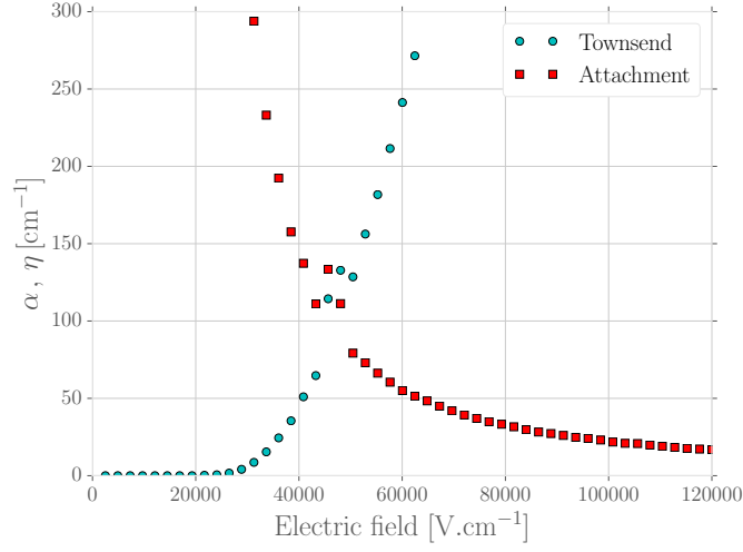
(a) \text{C}_2\text{H}_2\text{F}_4/\text{CO}_2/\text{SF}_6 93%/5%/2%
