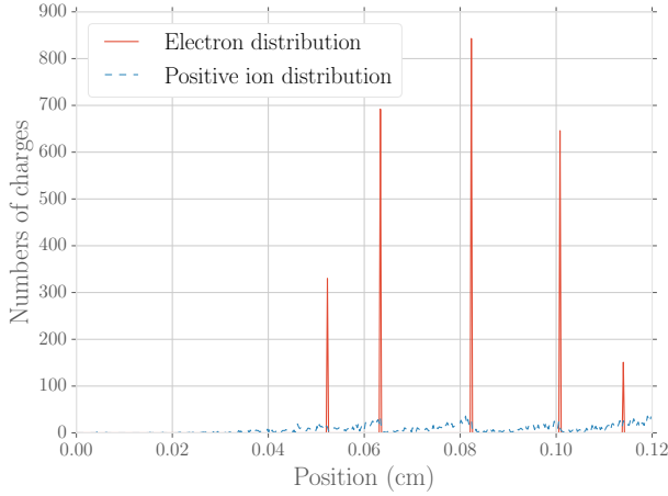
(a) n_e = 2662
