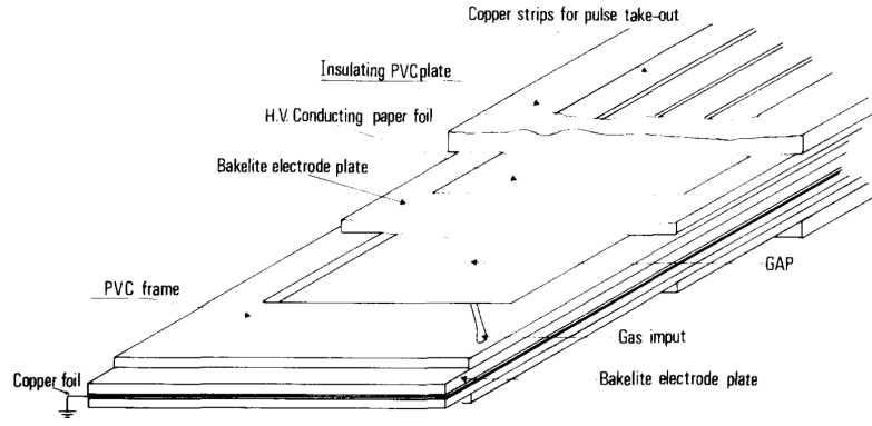
Figure 1.12: Sketch of the first RPC prototype. (From [92])
