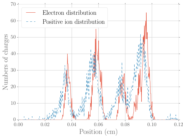
(c) n_e = 3828
