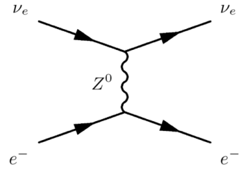
(b) Feynman diagram of neutral neutrino-electron scattering.
