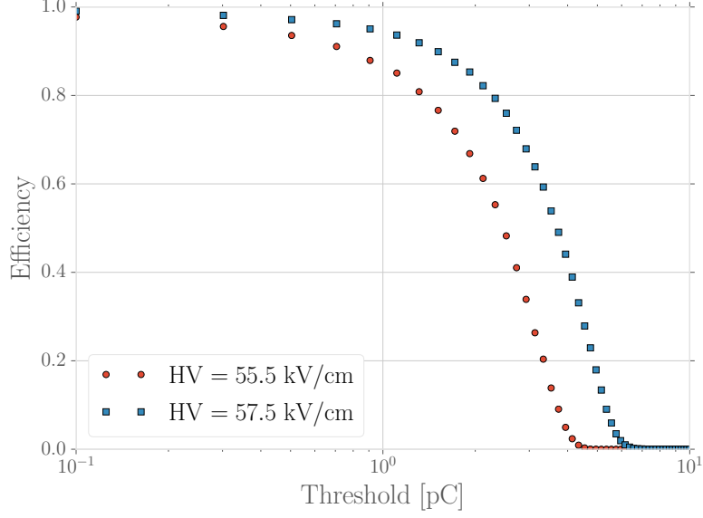
Figure 6.4: Efficiency as a function of the detection threshold. We used the CALICE RPC geometry and gas, with an applied electric field of 55.5 and 57.5 kV cm -1
