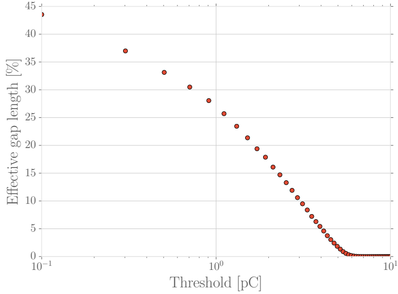
Figure 6.5: Effective gap length. We used the CALICE geometry, with an electric field of 57.5 kV cm -1 and 5 GeV/c muons.
