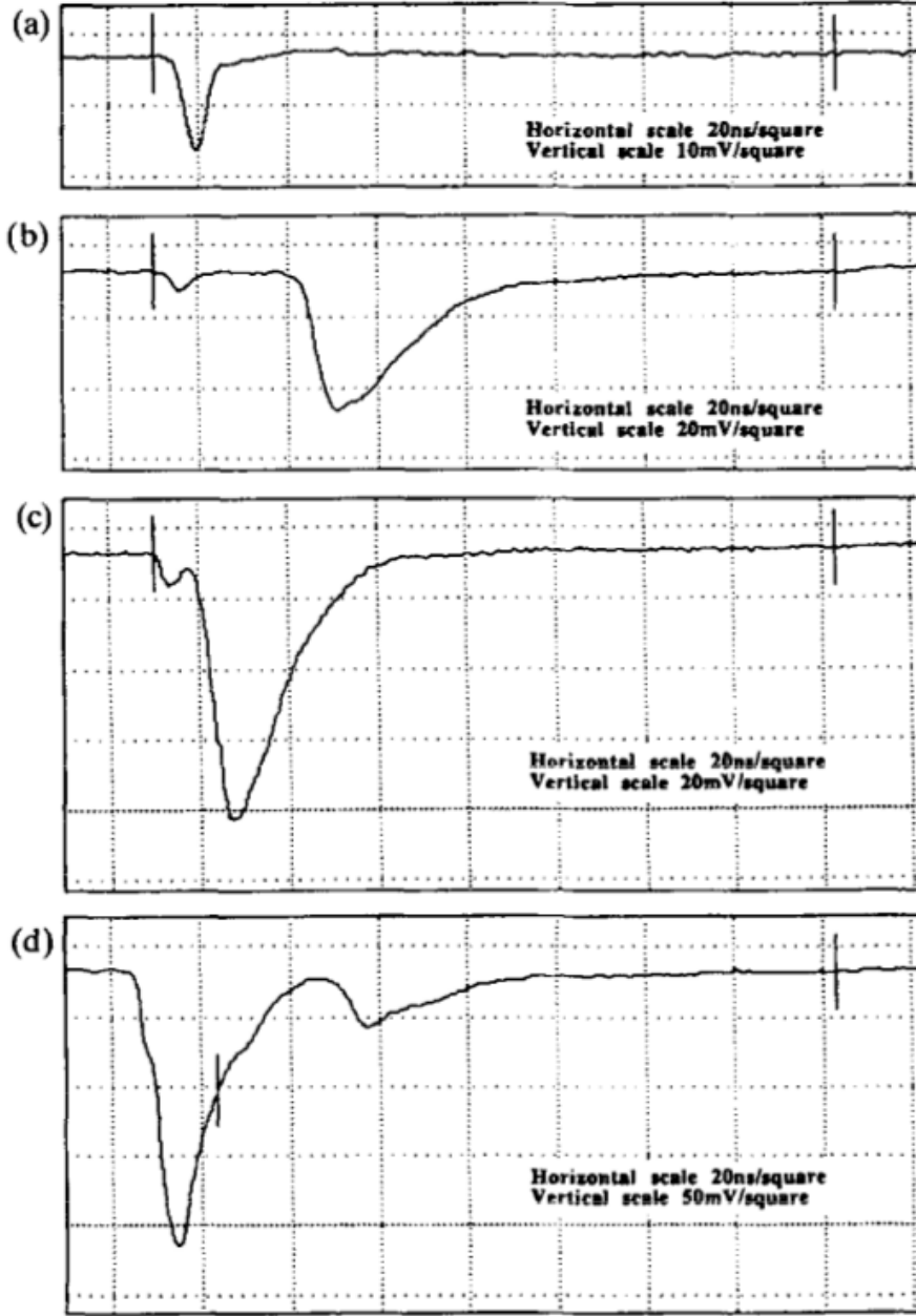
Figure 3.18: Signal from an 2 mm-wide RPC at different operating voltage, operated with \text{C}_2\text{H}_2\text{F}_4 . (a) 9.4 kV, typical avalanche signal. (b) 9.6 kV a streamer appears after a time delay of 38 ns. (c) 10.2 kV The delay becomes shorter. (d) 11.4 kV the avalanche and streamer merged and becomes indistinguishable, also a second streamer signal is present. (From [22])
