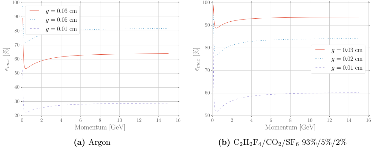
Figure 6.1: The maximum efficiency (eq.6.3) as a function of the muon momentum, for different gap widths, in pure Argon and in the CALICE sDHCAL mixture.
