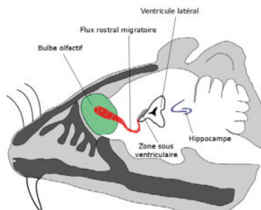
Figure 3. Neurogenèse adulte.
