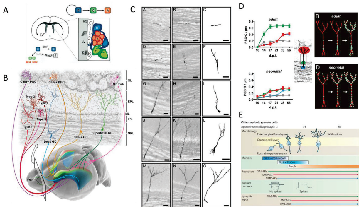
Figure 6: Adult-born interneurons
