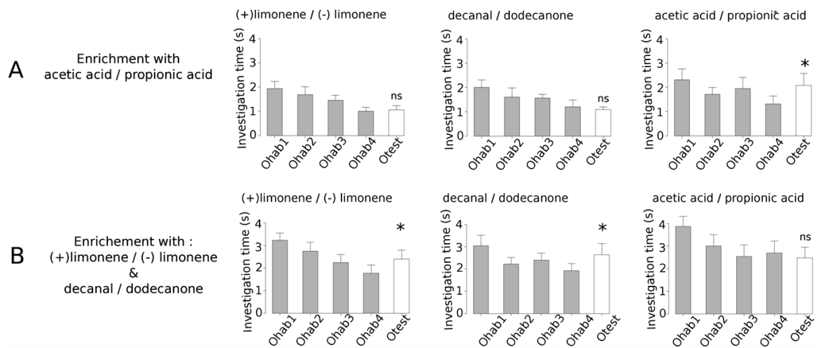
Figure 8: Discrimination tests.
