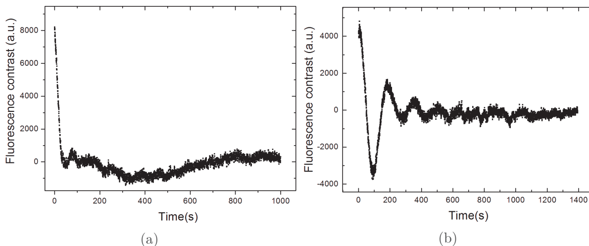
Figure 5.14: Intensity contrast as a function of time for a lamellar mesophase \Phi_m = 10 wt. % and C_p = 2 wt. %. With fringe spacing i = 19.8\ \mu\text{m} (a) and i = 39.6\ \mu\text{m} (b).
