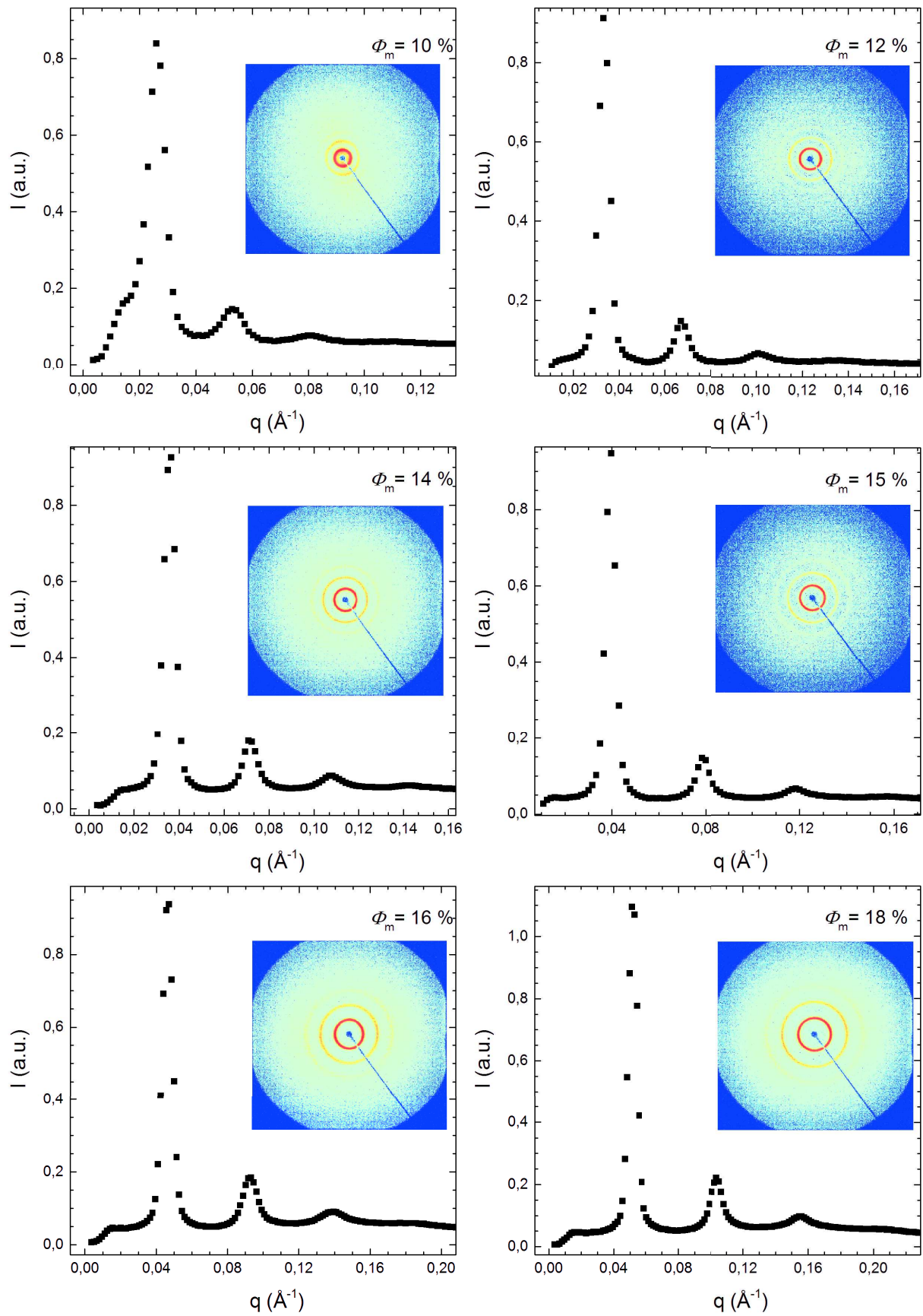
Figure A.7: The intensity scattered by the mesophases along the dilution line at constant polymer amount ( C_p = 5 \text{ wt. \%} ).
