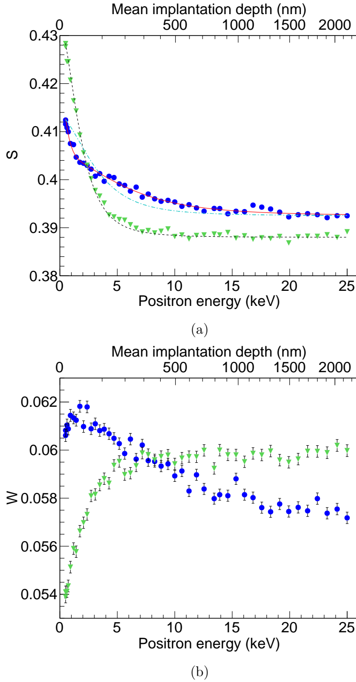
Figure 7.8: (a) S parameter as a function of the beam energy for the ( \bullet ) epitaxial layer and the ( \blacktriangledown ) substrate. The curves were fitted using VEPFIT [134] resulting in a diffusion length of L_{\text{eff}} = 6.6 \pm 0.3 nm for the first epitaxial layer, while for the second layer the diffusion length is L_{\text{eff}} = 250 \pm 10 nm (—). The substrate diffusion length is L_{\text{eff}} = 38.0 \pm 0.5 nm (---). A curve (- · -) corresponding to a fit of the epitaxial data points but assuming only one layer is present. (b) W parameter as a function of the beam energy for the ( \blacktriangledown ) epitaxial layer and ( \blacktriangledown ) substrate.
