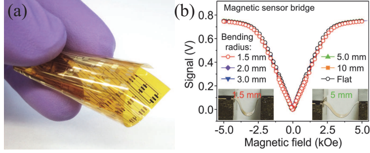
Figure 0.0.2 – a) Array of flexible magnetosensory systems. These are made of Co/Cu multilayers deposited on Kapton foils. These flexible magnetosensitive sensors can be used to monitor displacements or motion and provide feedback as needed. b) Response of the magnetic sensor bridge measured at different bending radii and plotted versus applied magnetic field.
