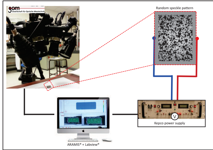
Figure 2.4.3 – Stereo camera experimental set up used during this thesis. The electric field inside the actuator is generated thanks to a voltage applied by using a KEPKO Bipolar power supply. The ARAMIS software is used to analyze the images.
