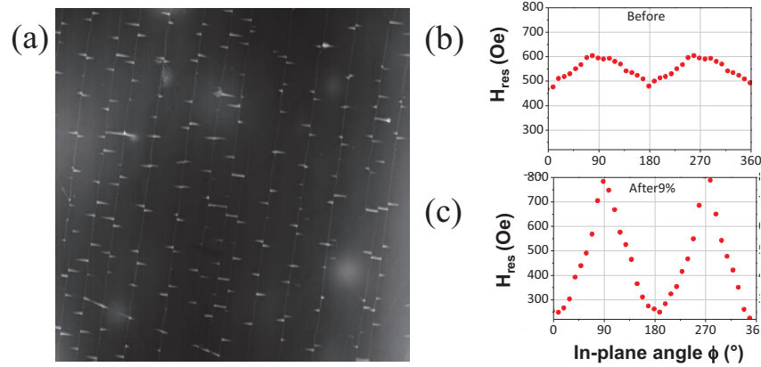
Figure 7.0.3 – (a) 20 \times 20 \mu\text{m}^2 AFM images of a CFB thin film taken at \varepsilon = 9\% . The angular dependance of the resonance field H_{res} has been measured (b) before tensile test (c) after tensile test with maximum strain \varepsilon = 9\% .
