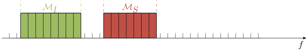
Figure 3.1: Spectral representation of the considered scenario. The incumbent and secondary systems coexist in the same spectral band, and each one is assigned a different subset of subcarriers. Because the systems are not coordinated, the secondary system may misalign its subcarriers with respect to the frequency basis of the incumbent by a frequency offset \delta_f .
