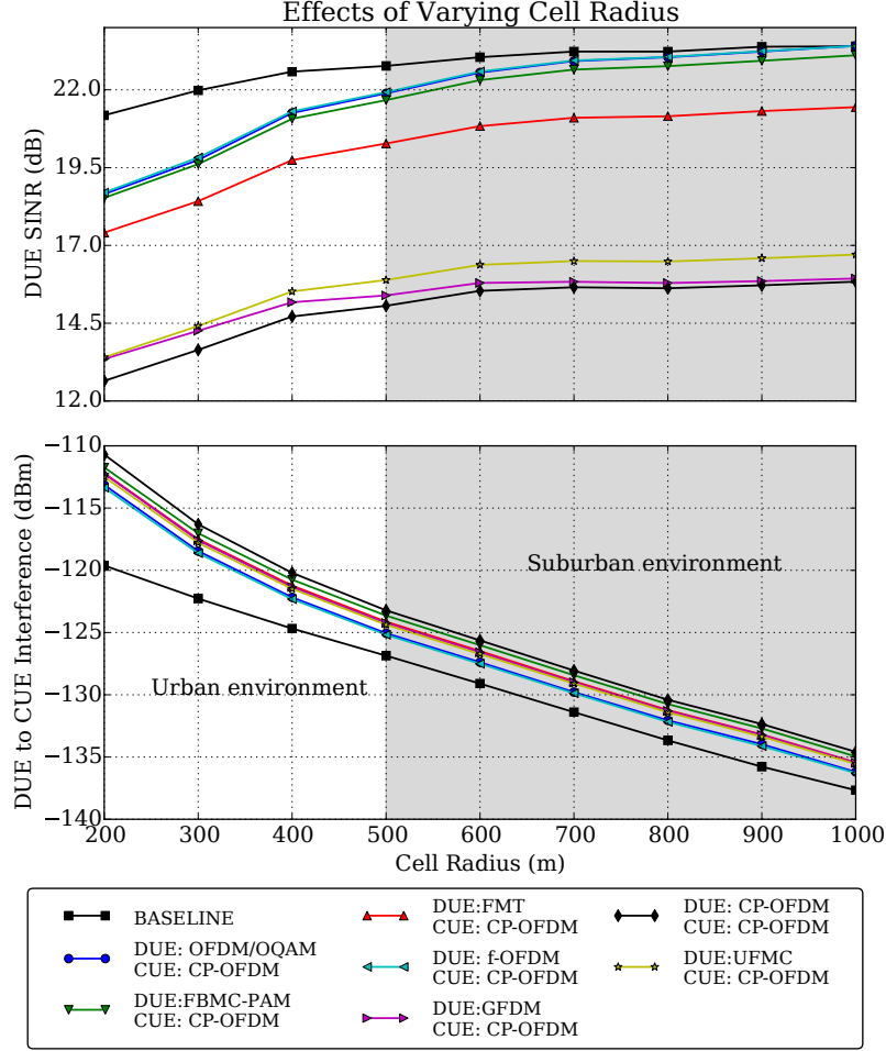
Figure 6.16: As the cell radius increases, DUE SINR increases and reduction in CUE SINR decreases.
