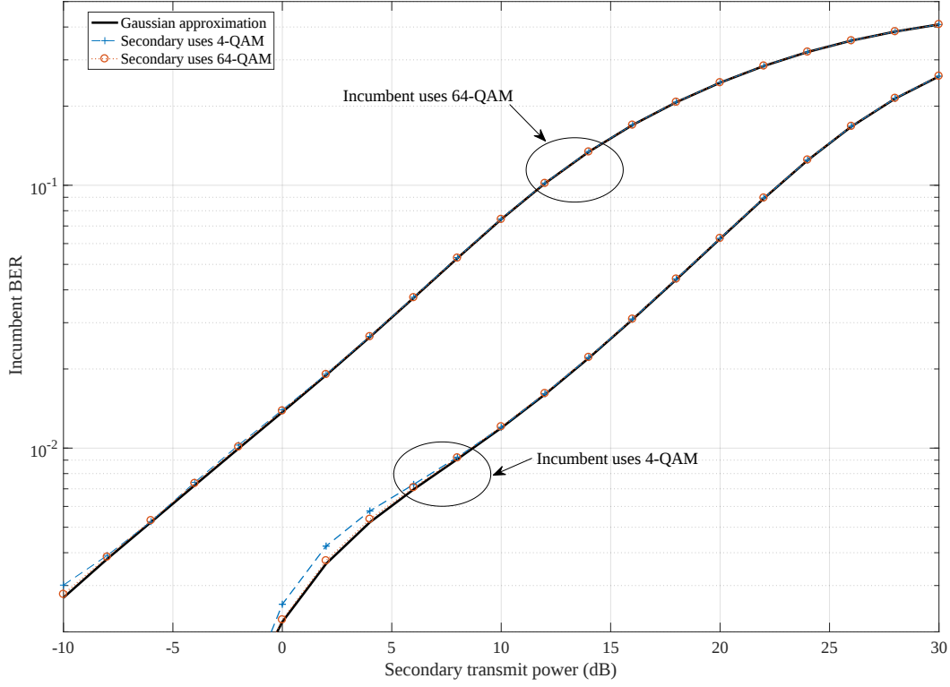
Figure 4.7: BER of the incumbent system for different constellation orders. The higher the constellation order of the secondary is, the more accurate the Gaussian approximation is. Nevertheless, even in the case where the secondary uses 4-QAM, the Gaussian approximation gives good results.
