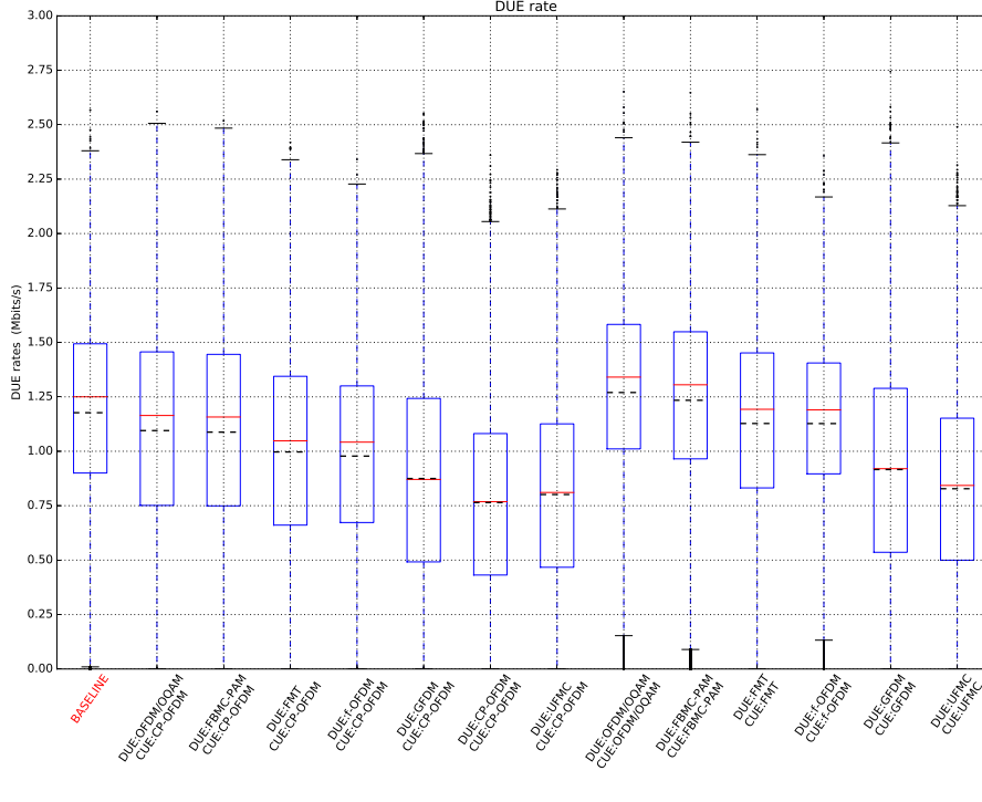
Figure 6.13: Rate performance of DUEs taking into account bandwidth efficiency.
