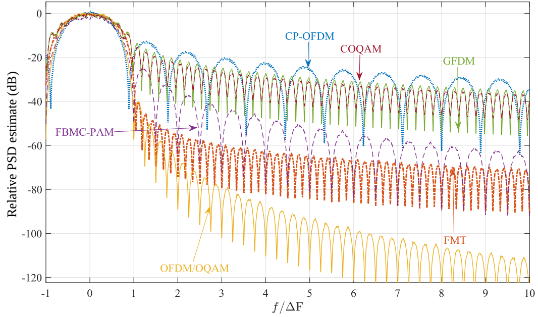
Figure 3.4: Welch estimate of the PSD level of studied waveforms with a Hanning Window of length \frac{100}{\Delta F} and a frequential resolution of 500 points per subcarrier. PSD values are expressed relatively to their maximum.
