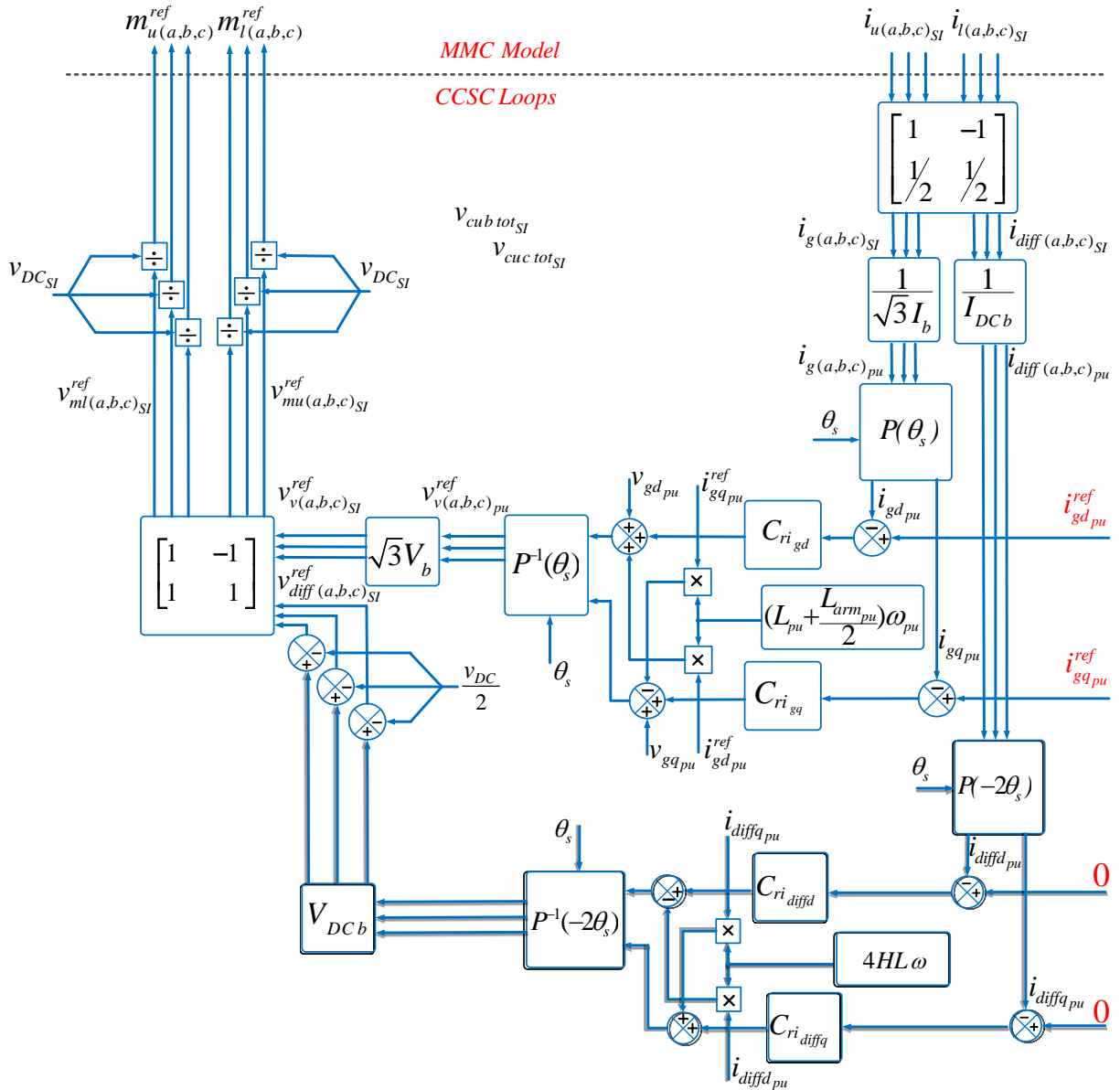
Figure 2-7: Structure of circulating current suppression controller in dq frame (CCSC)
