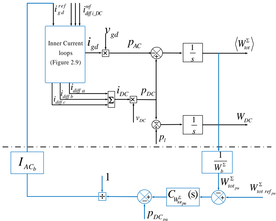
Figure 4-6: MMC connected to a variable DC link when the energy is controlled by the AC power
