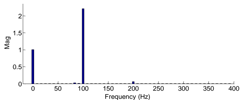
Figure 2-6: Spectrum of differential current with AC current control
