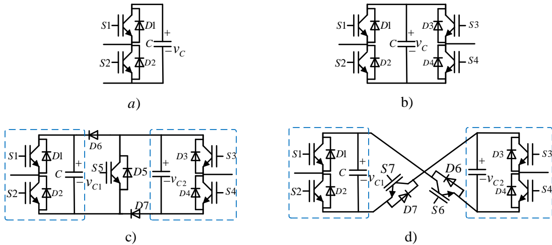
Figure 1-5: The MMC main sub-module topologies
