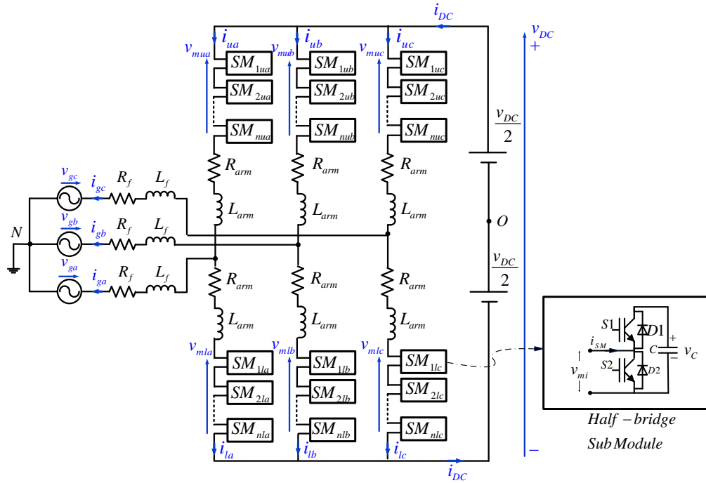
Figure 1-9: The MMC based on half bridge SM
