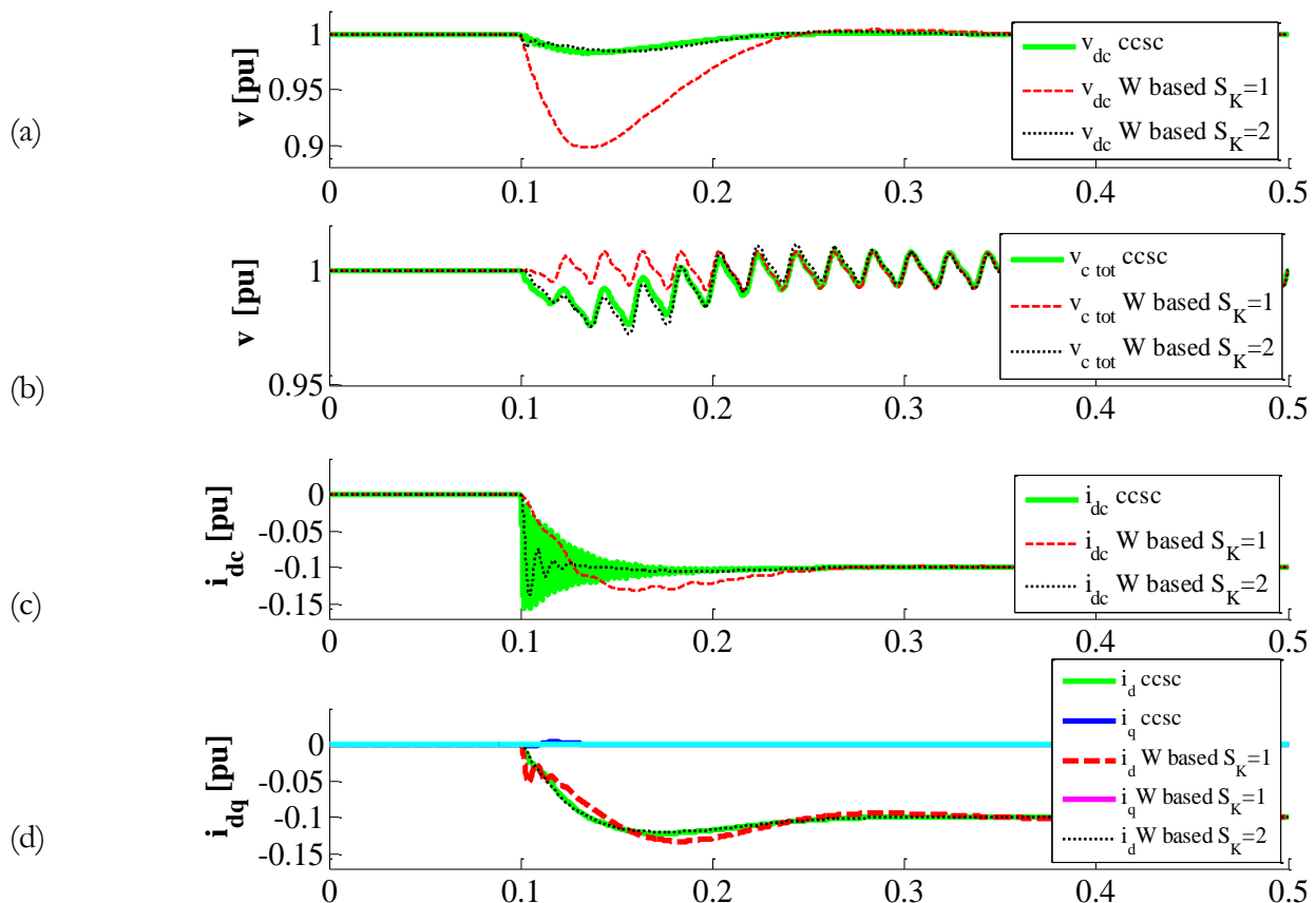
Figure 4-9: Comparison results between CCSC and energy-based control with variable DC bus voltage in two cases if DC voltage controlled by AC power
