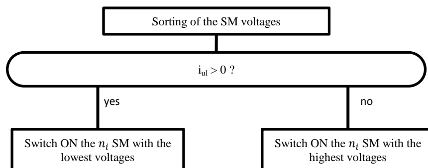
Figure 1-13: Basic BCA flowchart
