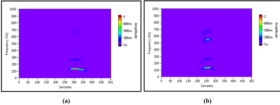
Figure 4.8: Spectrograms after Normalization and Noise Removal using a Hamming Window of Size 256
