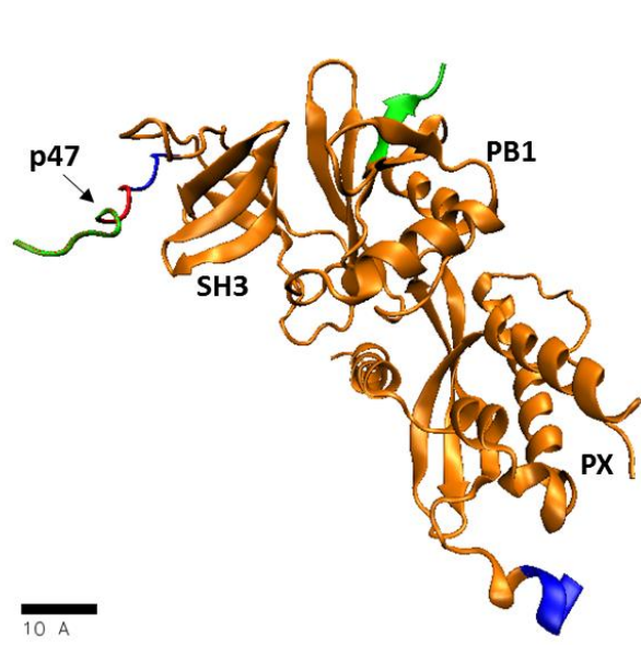
Figure 62 Alignment of the full-length crystal structure of p40 phox with the one of the interaction to p47 phox
