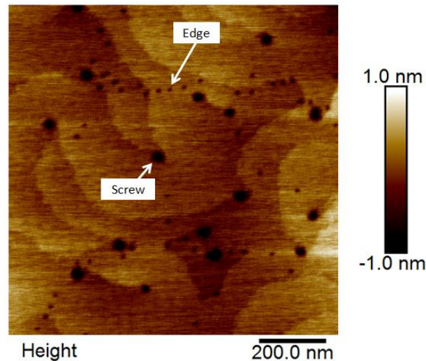
Fig. 1.16 – 1 \times 1 \mu\text{m}^2 AFM picture of GaN surface grown at 930^\circ\text{C} .
