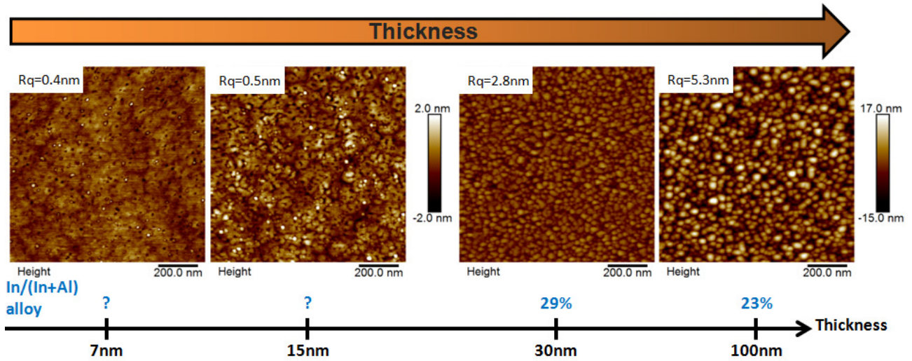
Fig. 4.27 – Effect of thickness : on topology on 1 \times 1 \mu\text{m}^2 AFM pictures, and alloy composition by XPS. T=730^\circ\text{C} , V_g=3\text{nm}/\text{min} , gas mixture : 41% of indium precursors in the gas phase, carrier gas : \text{N}_2 .
