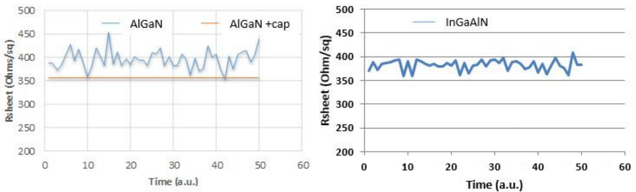
Fig. 6.6 – Comparison between Rsheet measurements on AlGaIn barrier layers with and without an SiN cap, and on an InGaAlN barrier with a SiN cap grown at 830^\circ\text{C} during 320s.
