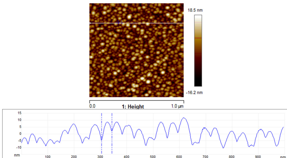
Fig. 5.6 – 1 \times 1 \mu m^2 AFM picture showing the surface morphology of a 100nm thick InAlN sample (sample1). Below, a section showing the profile of the topology.
