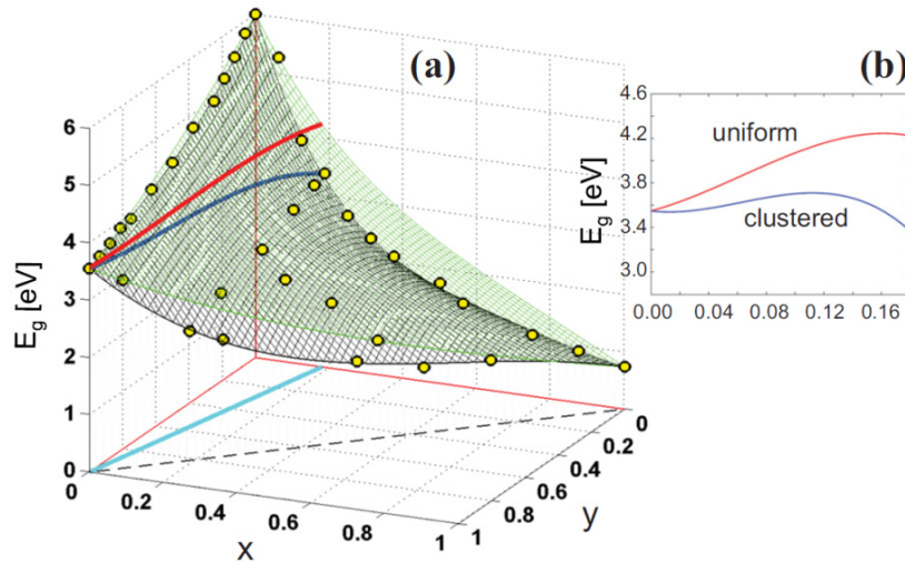
Fig. 1.7 – (a) Theoretical illustration InGaAlN quaternary band gap. In green color, uniform material. In black color, material with indium-rich areas. (b) Band gap versus indium ratio for an InGaAlN matched on GaN.[29]
