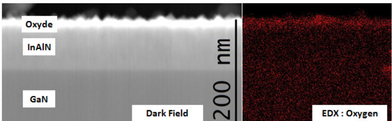
Fig. 4.28 – TEM cross section of 100nm thick InAlN with EDX analysis on oxygen.
