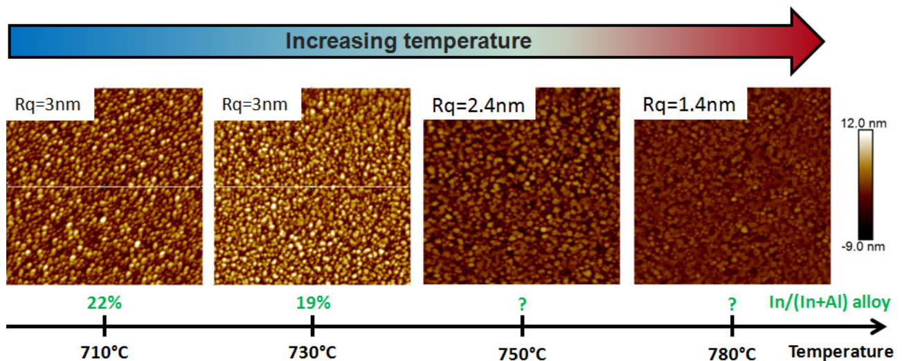
Fig. 4.26 – Effect of growth temperature : on topology on 1 \times 1 \mu m^2 AFM pictures, and alloy composition by XPS. Thickness=30nm, gas mixture : 41% of indium precursors in the gas phase, V_g=3\text{nm}/\text{min} , carrier gas : N_2 .
