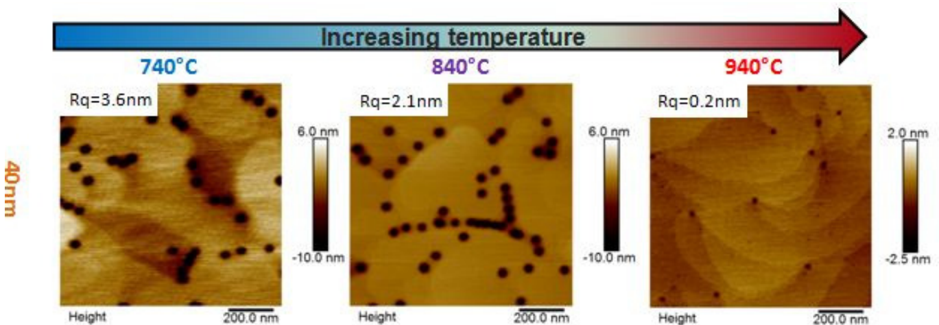
Fig. 3.6 – 1 \times 1 \mu\text{m}^2 AFM images of low temperature GaN grown at three temperatures, using N 2 as carrier gas and TMGa as gallium precursor. Vg=180nm/h for a thickness of 40nm.
