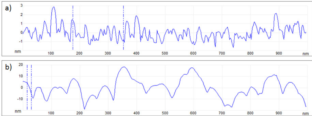
Fig. 4.16 – Cross-sectional view from 1 \times 1 \mu m^2 AFM images on a) 12nm, and b) 200nm thick InGaAlN sample showing the grain structure at the surface.
