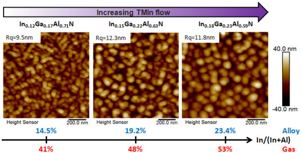
Fig. 4.8 – Effect of TMIn flow at fixed TMAI flow : on topology on 1 \times 1 \mu\text{m}^2 AFM pictures, and gas-alloy composition by XPS. Thickness=200nm, T=730^\circ\text{C} , V_g=3\text{nm}/\text{min} , carrier gas : \text{N}_2 .
