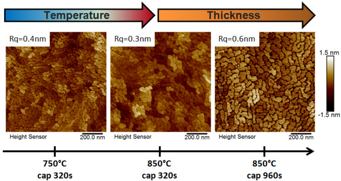
Fig. 6.8 – 1 \times 1 \mu m^2 AFM pictures of 12nm thick In_{0.10}Ga_{0.19}Al_{0.71}N layers having different SiN cap SiN growth temperature grown under hydrogen.
