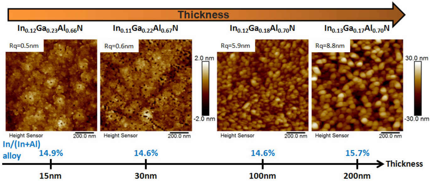
Fig. 4.4 – Effect of thickness on topology on 1 \times 1 \mu m^2 AFM pictures, and alloy composition by XPS. T=730^\circ C , V_g=3nm/min , TMI n/(TMI n + TMAI) : 41% in the gas phase, carrier gas : N_2 .
