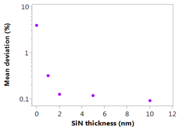
Fig. 6.2 – Comparison of noise in Rsheet measurements on AlGaN barrier layers different thicknesses of SiN cap.
