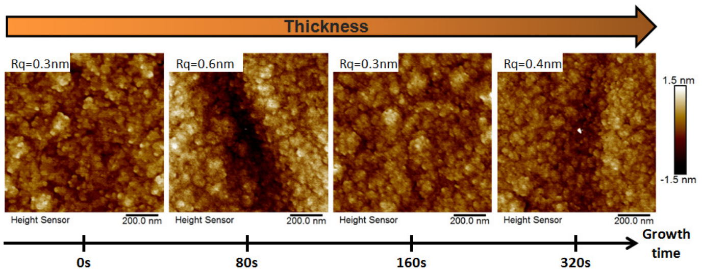
Fig. 6.4 – 1 \times 1 \mu m^2 AFM images of 12nm thick InGaAlN layers having different SiN deposition time grown under nitrogen at 725°C.
