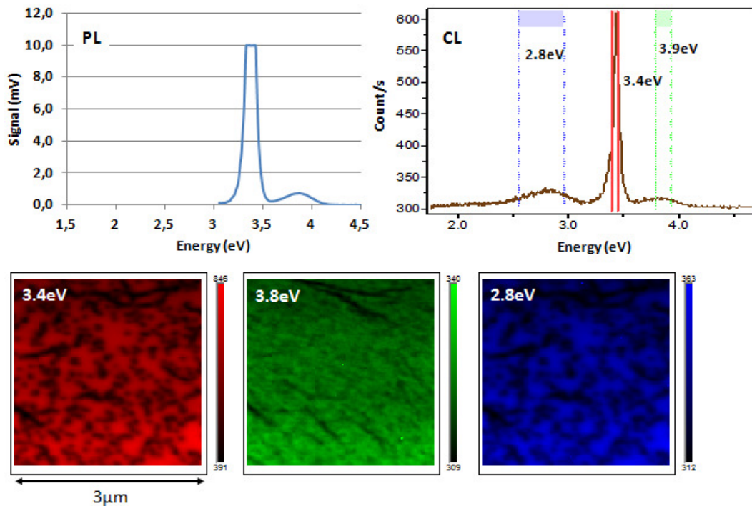
Fig. 4.22 – Spectra of sample 2 : comparison of PL and CL. 3 \times 3 \mu\text{m}^2 pictures showing luminescence at different energy.
