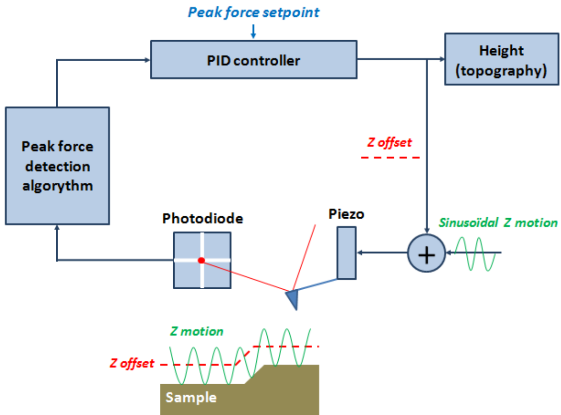
Fig. 2.24 – Peak force mode layout
