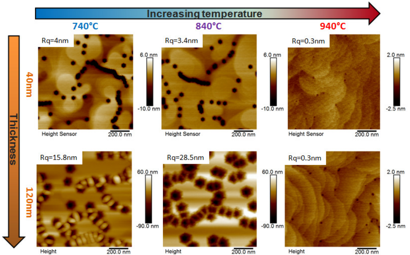
Fig. 3.4 – 1 \times 1 \mu\text{m}^2 AFM images of low temperature GaN grown at three temperatures for two different thicknesses, using \text{N}_2 as carrier gas and TMGa as gallium precursor. V_g=540\text{nm/h} .
