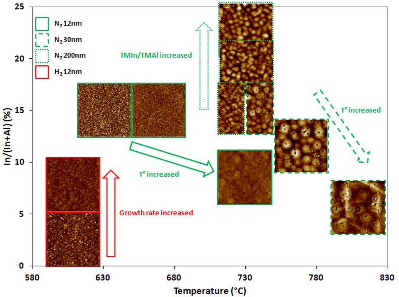
Fig. 5.14 – Surface diagram of InGaAlN samples using 1 \times 1 \mu\text{m}^2 AFM pictures. Correlation of morphology, indium content and temperature.
