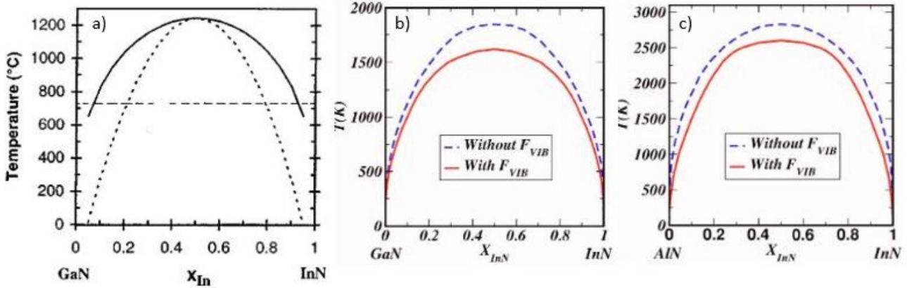
Fig. 2.21 – a) Phase diagram of InGaN ternary by Stringfellow [6], b) phase diagram of InGaN ternary by Burton [7], c) phase diagram of InAlN ternary by Burton [7].
