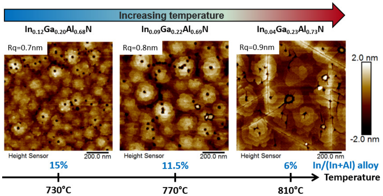
Fig. 4.13 – Effect of growth temperature : 1 \times 1 \mu\text{m}^2 AFM images, and alloy composition by XPS. Thickness=30nm, gas mixture : 41% of indium precursors in the gas phase, V_g=3\text{nm}/\text{min} , carrier gas : \text{N}_2 .
