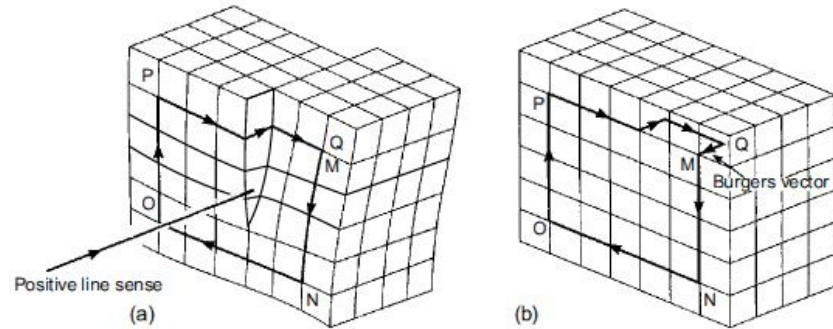
Fig. 1.13 – Burger circuit of cubic crystal with positive edge dislocation, and b) normal cubic crystal. Burger vector represented on b) with a black arrow.[31]
