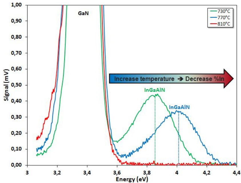
Fig. 4.14 – PL spectra of three 30nm thick samples having a, \text{In}/(\text{In}+\text{Al}) ratio of 6%, 12%, and 15%.
