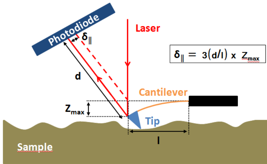
Fig. 2.26 – Interaction laser-tip-photodiode.
