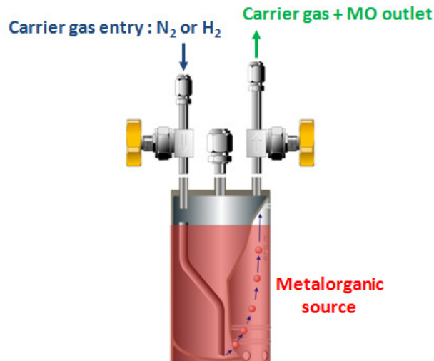
Fig. 2.10 – Bubbler schematic.
