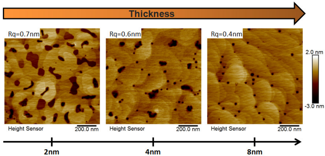
Fig. 6.13 – 1 \times 1 \mu\text{m}^2 AFM pictures of three different thicknesses of GaN caps on 12 nm thick InGaAlN barrier layer. T_{\text{cap}} = 730^\circ\text{C} .
