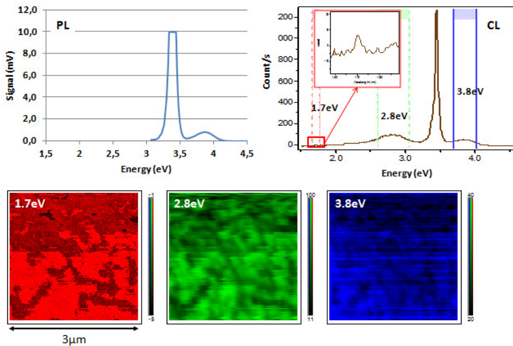
Fig. 4.21 – Spectra of sample 1 : comparison of PL and CL. 3 \times 3 \mu\text{m}^2 pictures showing luminescence at different energy.
