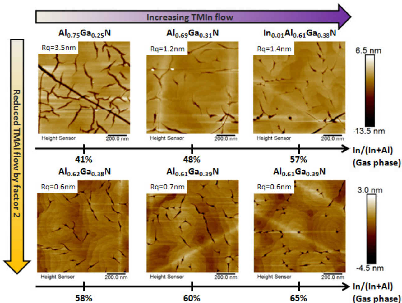
Fig. 4.24 – Effect of TMIIn and TMAI flow : 1 \times 1 \mu\text{m}^2 AFM images. Gas phase composition specified below AFM pictures. Thickness=30nm, T=750°C, Vg=3nm/min, carrier gas : H 2 .
