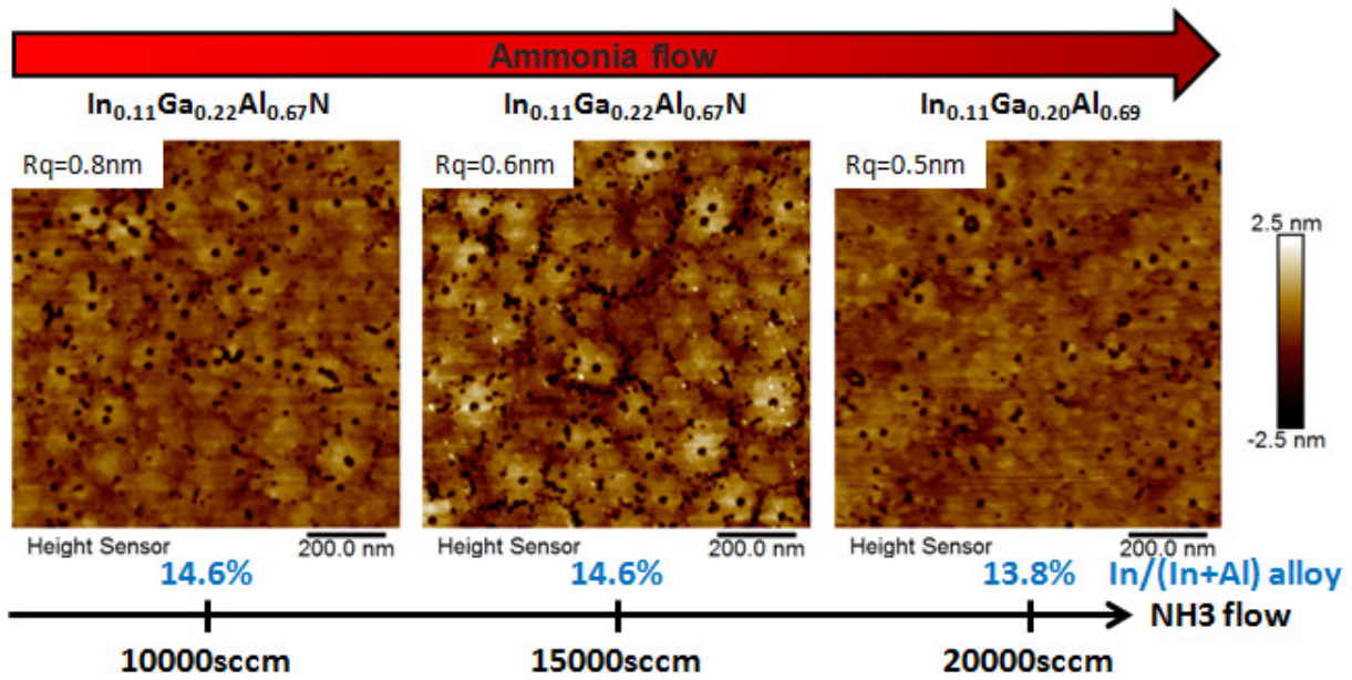
Fig. 4.20 – Effect of ammonia flow : 1 \times 1 \mu\text{m}^2 AFM images, and alloy composition by XPS. Thickness=30nm, gas mixture : 41% of indium precursors in the gas phase, T=730^\circ\text{C} , V_g=3\text{nm}/\text{min} , carrier gas : \text{N}_2 .
