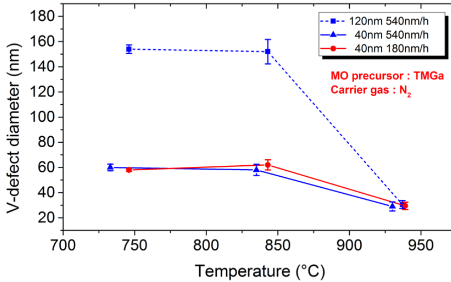
Fig. 3.5 – The figure shows the evolution of V-defect diameter versus growth temperature. Growth rates are fixed at 540 nm/h and 180 nm/h with TMGa precursor and N 2 carrier gas.
