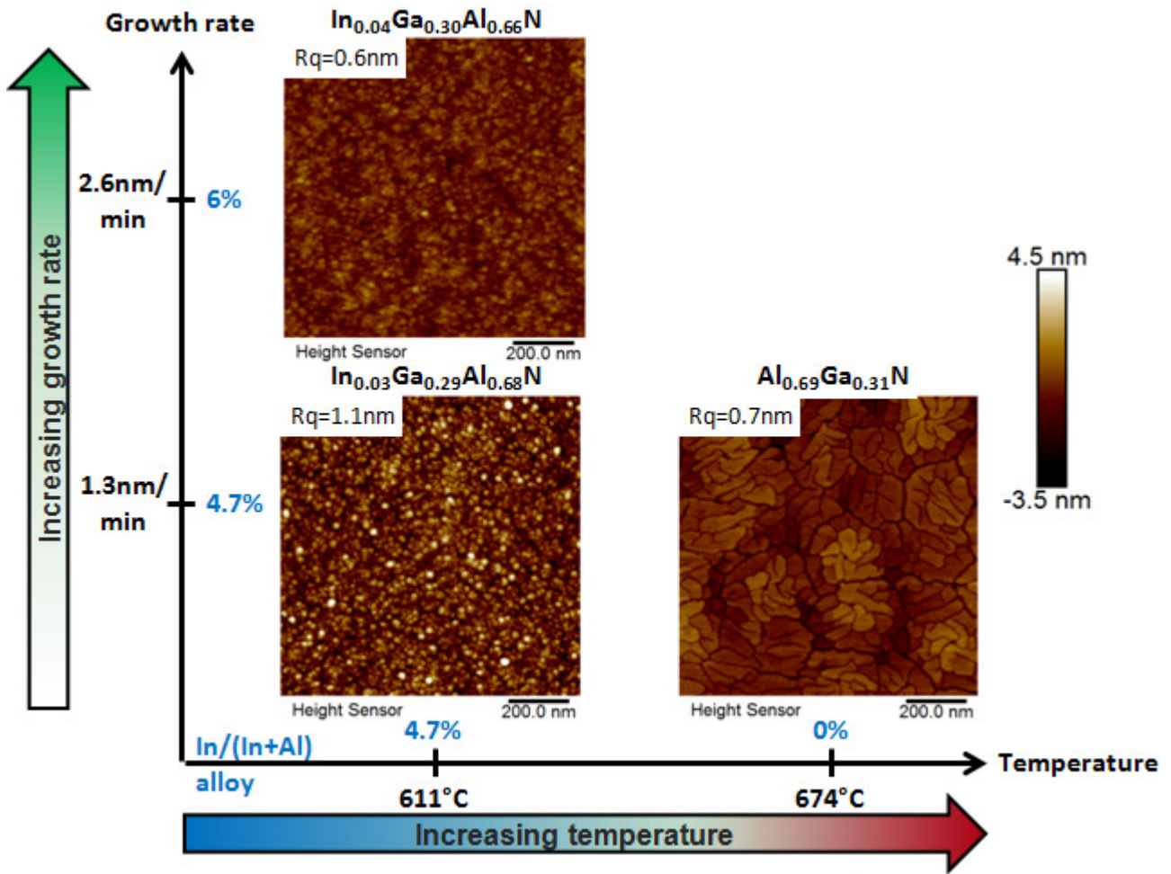
Fig. 4.25 – Effect of T and Vg : 1 \times 1 \mu\text{m}^2 AFM pictures. Gas phase composition specified below AFM images. Thickness=13nm, gas mixture : 41% of indium precursors in the gas phase, carrier gas : H 2 .
