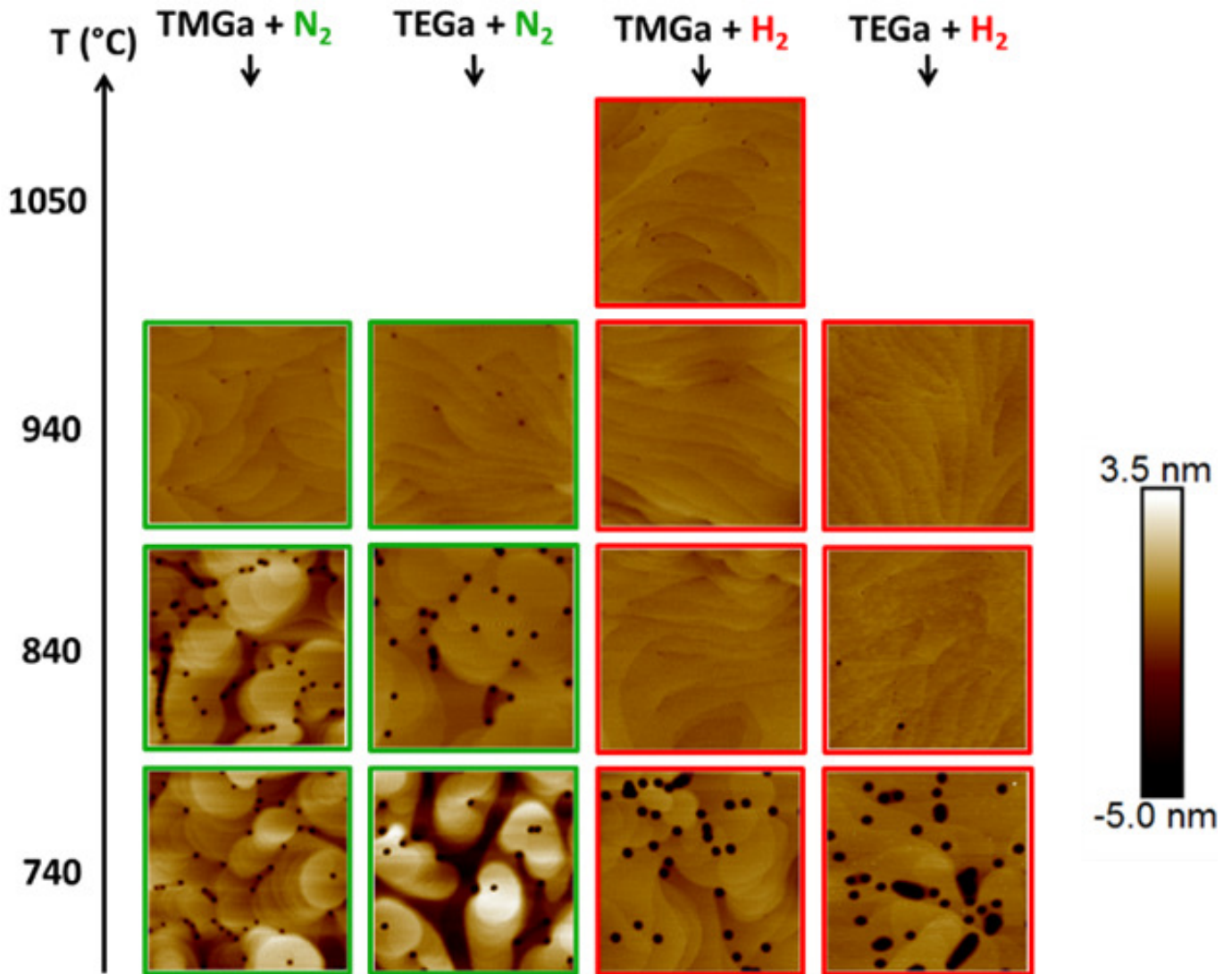
Fig. 3.9 – 1 \times 1 \mu\text{m}^2 AFM images of GaN grown at various temperatures, using H 2 and N 2 as carrier gas and TMGa and TEGa as gallium precursors.
