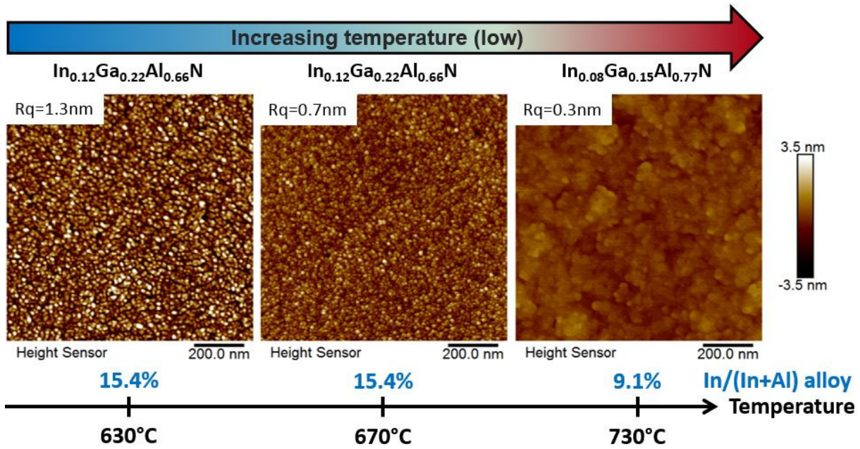
Fig. 4.15 – Effect of growth temperature : 1 \times 1 \mu\text{m}^2 AFM images, and alloy composition by XPS. Thickness=12nm, gas mixture : 41% of indium precursors in the gas phase, V_g=3\text{nm}/\text{min} , carrier gas : \text{N}_2 .
