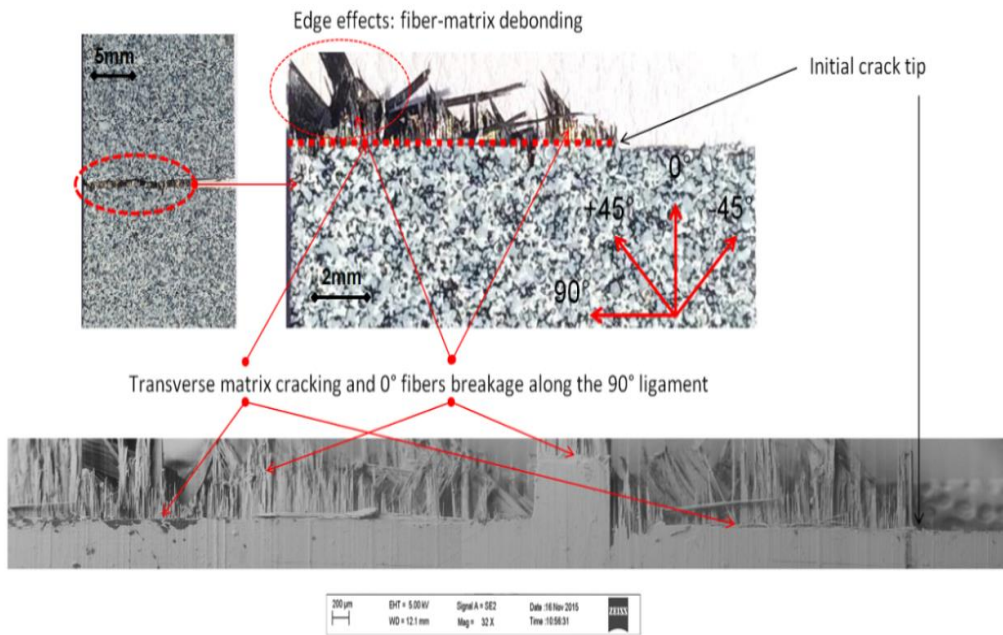
Figure 29. Macroscopic and SEM observations of fracture surface in QI SEN C/PPS specimens subjected to tensile loadings at 120°C
