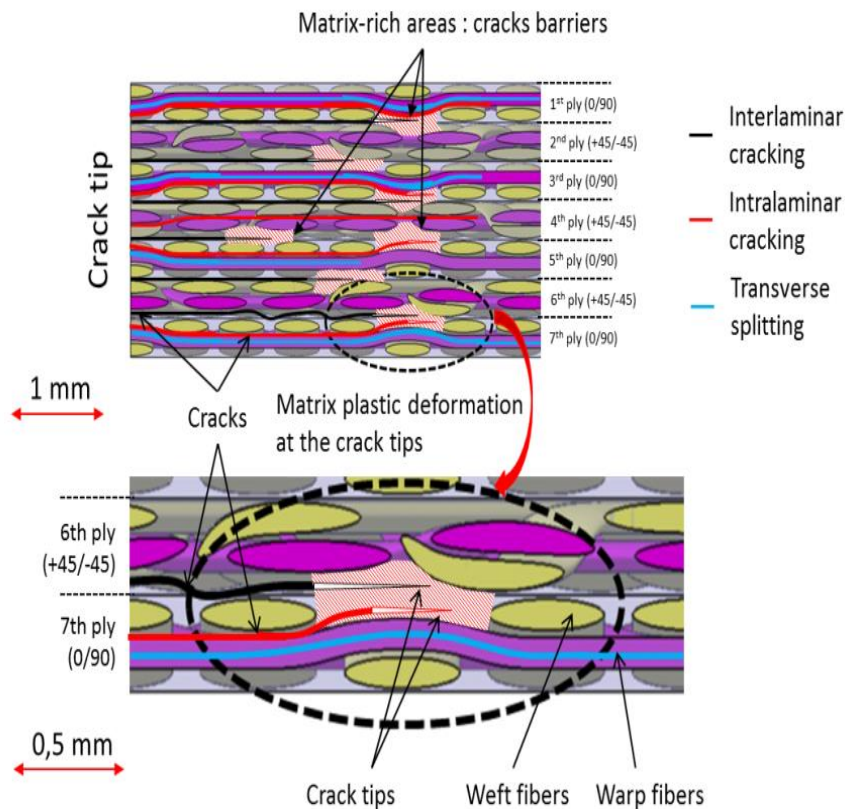
Figure 30. Schematic representation of damage evolution in QI SEN C/PPS specimens subjected to tensile loadings at 120°C
