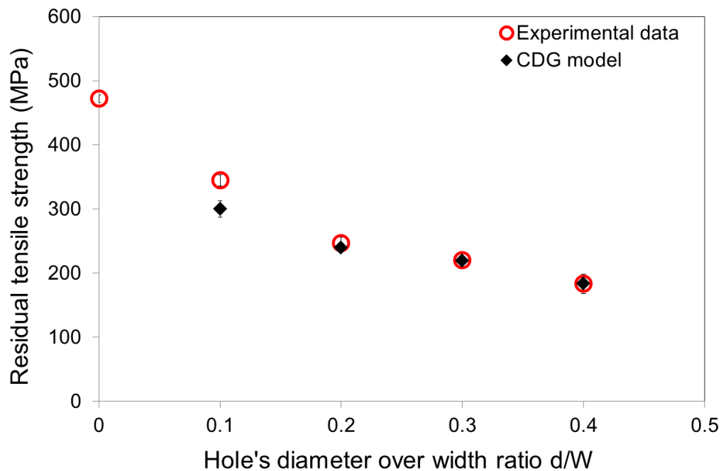
Figure 102. Prediction of the residual tensile strength as a function of the ratio d/w of the hole diameter over the specimen width for CCH quasi-isotropic C/PPS specimens at 120°C
