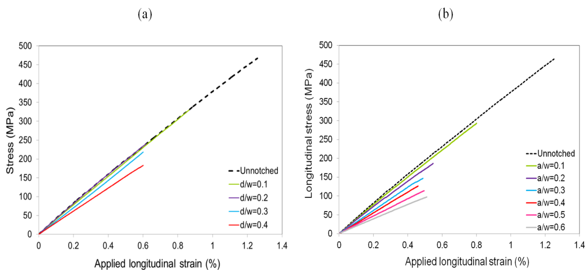
Figure 98. Influence of the ratio of the initial notch length over the specimen width ( d/w and a/W ) on the tensile responses of quasi-isotropic C/PPS specimens at 120°C: (a) Central Circular Hole – (b) Single-Edge Notch
