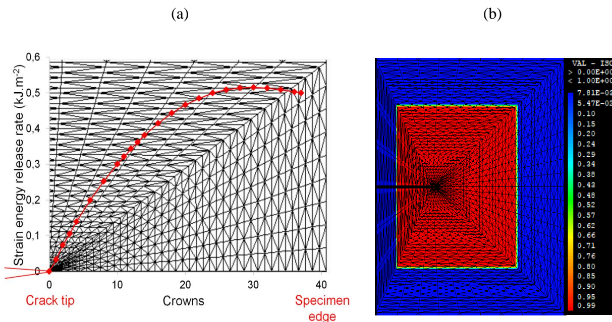
Figure 89. Path independence domain for a/W=0.3 in notched QI laminates: (a) Evolution of the strain energy release rate according to each crown and (b) \theta field in the 26th crown.
