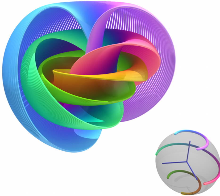
Figure II.2: A pictural representation 5 of the simplest Hopf fibration: the three-sphere S^3 is thought as a three-ball where all the points on the boundary are identified (i.e this is essentially a variant of the stereographic projection). It is fibred by circles of different colours. The two-sphere in the bottom-right corner represents the base space.
