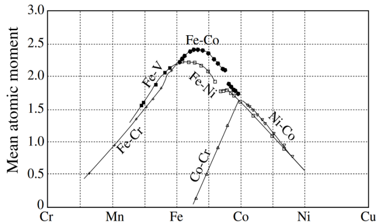
Figure 2.4: Slater-Pauling curve which is a plot of magnetic moment measurements of several TM alloys, where the maximum saturation magnetisation was found for \text{Fe}_{65-70}\text{Co}_{35-30} alloys with \mu_0 M_s = 2.45 \text{ T} ( M_s \sim 2.45 \times \frac{10^4}{4\pi} = 1950 \text{ emu/cm}^3 ) – the Slater-Pauling limit. From Sourmail, 2005
