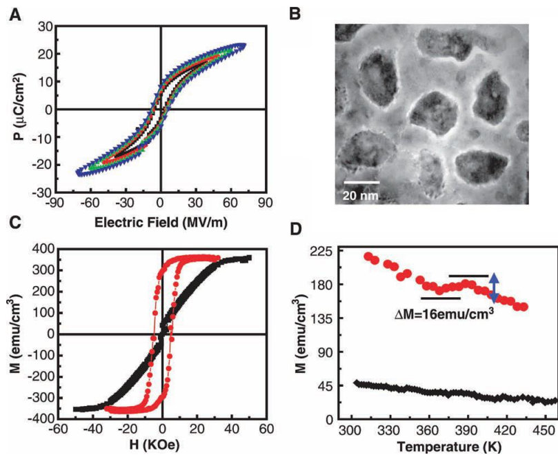
Figure 2.10: Multiferric BaTiO 3 -CoFe 2 O 4 nanocomposite: A,C: classical ferroic behavior showing the coexistence of ferroelectric and magnetic order. B: Planar transmission electron micrograph of the sample structure, showing the CoFe 2 O 4 nanopillars embedded in the BaTiO 3 matrix. D: Magnetization vs. temperature response of the system, showing a change in the magnetic response of the system with the onset of ferroelectric order (red symbols) compared with the signal from a simple multilayered structure showing negligible change in magnetism. From Zheng et al., 2004
