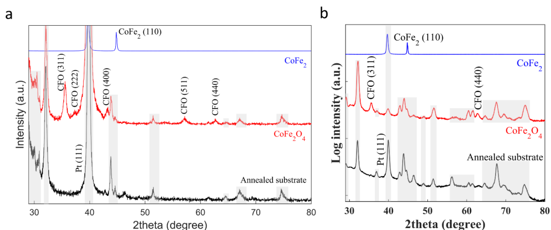
Figure 5.20: Out-of-plane powder XRD (a) and in-plane GIXRD (b) patterns of the vertically aligned \text{CoFe}_2 nanopillar arrays (blue), the \text{CoFe}_2\text{O}_4 nanopillar arrays (red), and the Pt/Ti/Si substrate annealed at \sim 600^\circ\text{C} (black)
