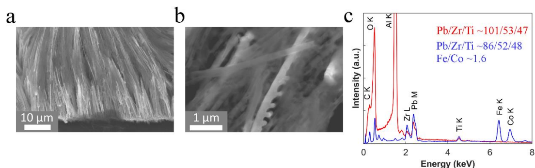
Figure 4.5: (a) Tilted top view SEM image of the PZT 500 -CoFe 2 nanocables after partial dissolution of the alumina ( D_{\text{pore}} \sim 150 nm, P_{\text{AAO}} \sim 35\% ). (b) Top view SEM images of the PZT 500 -CoFe 2 C arrays after full AAO dissolution, top segment of the PZT 500 nanotubes (unfilled with CoFe 2 ) can be distinguished by their transparent look and the PZT 500 -CoFe 2 nanocables can be found by their bright colour. (c) EDX spectra of the crystallized PZT 500 NTs inside AAO (red) and PZT-CoFe 2 nanocables after AAO dissolution (blue)
