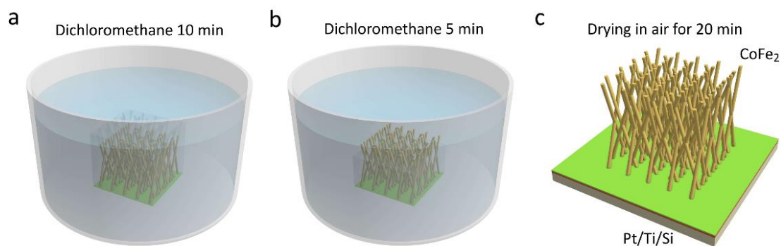
Figure 3.32: Flow chart of the polymer membrane chemical dissolution process. (a) Immersing of the polymer membrane hosting \text{CoFe}_2 3D interconnected nanowire network into a vessel containing dichloromethane solution for 10 min, (b) Immersing in the 2 nd dichloromethane solution for 5 min, (c) Drying of the \text{CoFe}_2 interconnected nanowire network in air for 20 min
