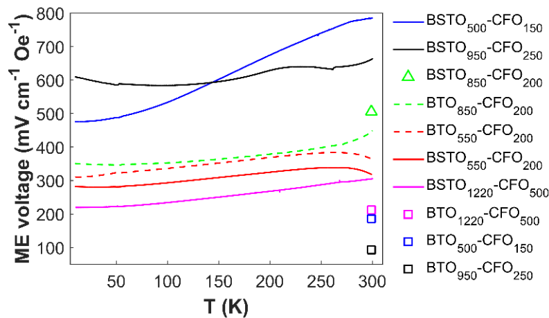
Figure 5.16: Temperature dependence of ME voltage coefficients for the BSTO-CFO and BTO-CFO nanocomposites, where the total thickness of the BSTO and BTO structure, t_{total} , varies between \sim 500 and 1220 nm, and the height of \text{CoFe}_2 nanopillars, h_{pillar} , is in the range \sim 150 - 500 nm. Solid lines and a triangle corresponds to the results for BSTO-CFO nanocomposites, while broken lines and squares correspond to the results obtained for BTO-CFO nanocomposites. Same colours correspond to the same ratio t_{total}/h_{pillar} .
