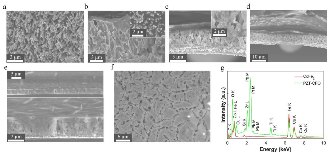
Figure 6.7: Tilted view SEM images on (a) 3D interconnected CoFe_2 nanowire network with D_{NW} \sim 230 nm and \alpha_{tilt} \sim 25^\circ , (b) corresponding PZT- CoFe_2 3D nanostructure after sol-gel dip-coating deposition and dehydration of PZT sol, (c,d) PZT-CFO nanostructure after simultaneous PZT crystallization and in situ oxidation of CoFe_2 3D NW network at 650 °C for 30 min at 5 °C/min heating rate, (e) PZT-CFO nanostructure after post-annealing at 600 °C for 12 hours at 2 °C/min heating rate. (f) Top view SEM micrograph on the corresponding post-annealed at 600 °C for 12 hours at 2 °C/min PZT-CFO 3D nanostructure shown in (e). (g) EDX analysis spectra for the CoFe_2 3D NW network (red) and the PZT-CFO 3D nanostructure (green)
