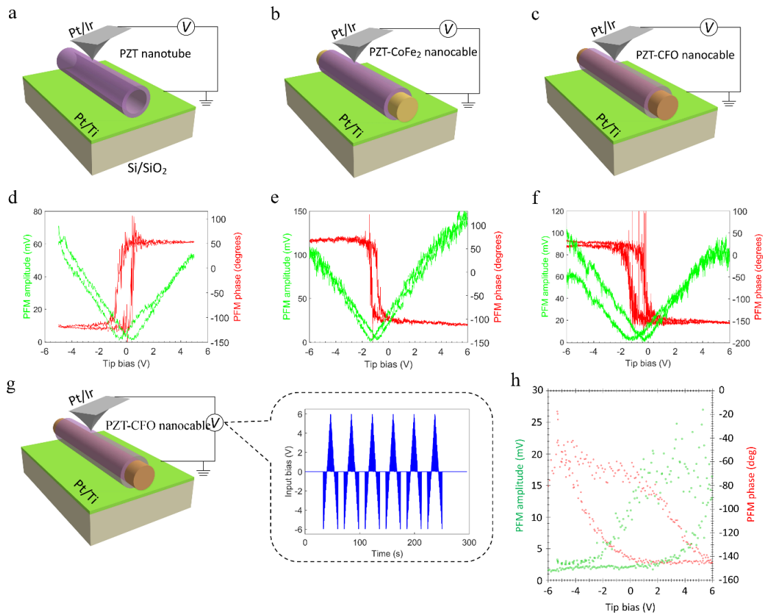
Figure 4.13: Schematic of localized ferroelectric characterization and domain switching shown by in-field phase (red line) and amplitude (green line) hysteresis loops for (a,d) the three-layer PZT 500 nanotube; (b,e) the PZT 500 -CoFe 2 nanocable; (c,f) the PZT 500 -CFO 600 nanocable. (g) Switching spectroscopy PFM (SS-PFM) mode with application of triangular-shaped voltage pulses; (h) SS-PFM measured amplitude (green dots) and phase (red dots) hysteresis loops for the PZT 500 -CFO 600 nanocable domains located at the top margin of the PZT 500 -CoFe 2 nanocables are mostly polarized downwards, indicated by the darker colour than that in the central area of nanocables.
