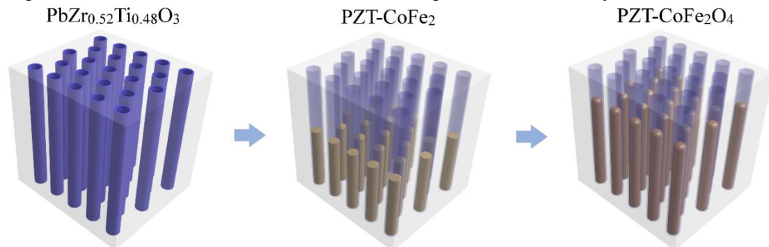
Figure 4.1: Schematic illustration of fabrication process of the core-shell \text{PbZr}_{0.52}\text{Ti}_{0.48}\text{O}_3 - \text{CoFe}_2\text{O}_4 nanocable arrays by sol-gel dip-impregnation of PZT nanotubes into a commercial AAO membrane, pulsed electrodeposition of \text{CoFe}_2 nanowires arrays into PZT nanotubes, and their thermal oxidation into \text{CoFe}_2\text{O}_4 phase nanowires
