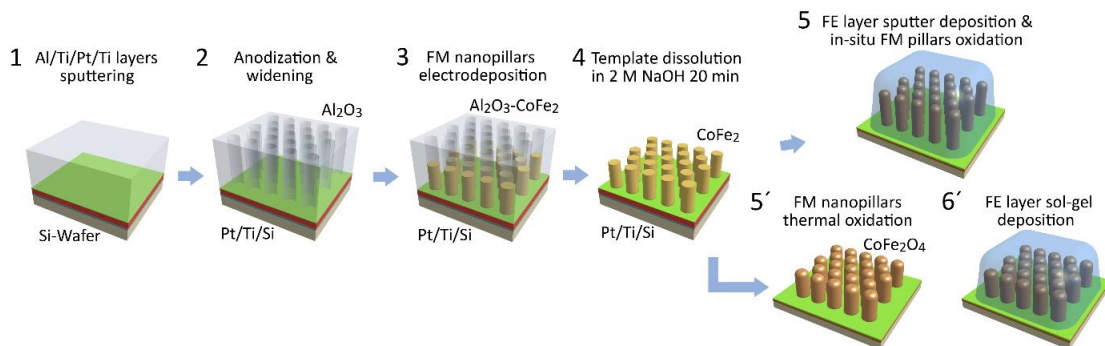
Figure 3.14: Schematic fabrication of the vertically aligned magnetolectric nanocomposites based of ferromagnetic \text{CoFe}_2\text{O}_4 nanopillars. (1) Sputter deposition of the Al/Ti/Pt/Ti multilayer ( \sim 1 \mu\text{m}/5\text{nm}/50\text{nm}/5\text{nm} ) on the \text{SiO}_2/\text{Si} wafer; (2) Top Al/Ti bilayer anodization & widening process to form porous AAO template on the Pt/Ti/ \text{SiO}_2/\text{Si} substrate; (3) Pulsed electrodeposition growth of \text{CoFe}_2 nanopillar array; (4) Chemical dissolution of the hosting AAO template; (5) RF magnetron sputtering of the \text{Ba}_{0.7}\text{Sr}_{0.3}\text{TiO}_3 or the \text{BaTiO}_3 matrix layer on the \text{CoFe}_2 nanopillar arrays, which are simultaneously in situ oxidized into \text{CoFe}_2\text{O}_4 phase; (5') Thermal oxidation of the free-standing \text{CoFe}_2 nanopillar array in a furnace; (6') Sol-gel dip coating deposition of the \text{PbZr}_{0.52}\text{Ti}_{0.48}\text{O}_3 matrix layer on the \text{CoFe}_2\text{O}_4 nanopillar array
