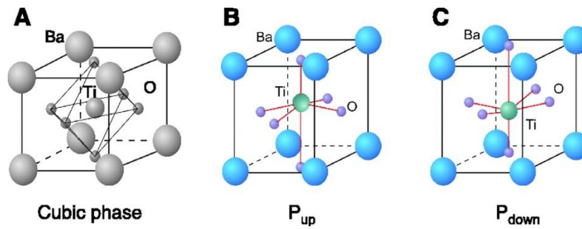
Figure 2.18: Crystal structure of the perovskite ferroelectric \text{BaTiO}_3 . (A) High temperature, paraelectric, cubic phase. (B and C) Room temperature, ferroelectric, tetragonal phases, showing up and down polarization variants. The atomic displacements are scaled to be clearly visible. From Ahn et al., 2004
