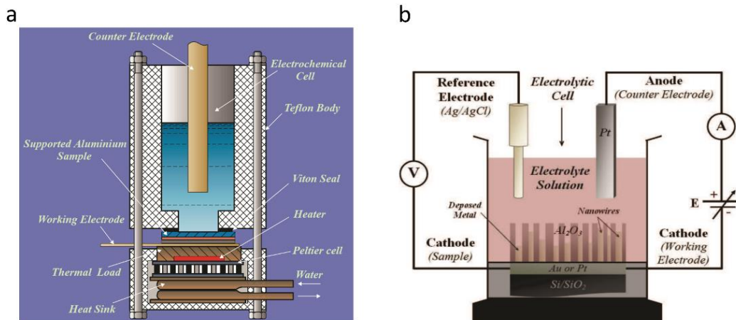
Figure 3.9: (a) The construction diagram of a typical electrolytic cell with temperature controlling features (from Mátefi-Tempfli, 2008) (b) Schematic of the “3-electrodes” potentiostatic electrochemical deposition setup (from Antohe, 2012)
