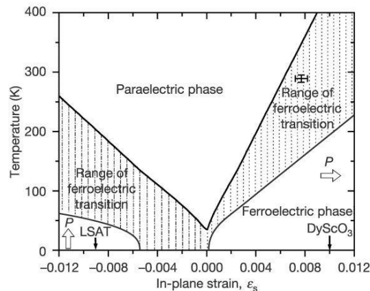
Figure 2.19: Expected T_c of (001) \text{BaTiO}_3 under biaxial in-plane strain \sigma , based on thermodynamic analysis. The arrows indicate the predicted direction of the polarization for strained \text{SrTiO}_3 : in-plane for biaxial tensile strain and out-of-plane for biaxial compressive strain. The \epsilon_s values for \text{SrTiO}_3 fully constrained (commensurate) to the lattice constants of LSAT and (110) \text{DyScO}_3 substrates are indicated by the positions of the corresponding arrows. The cross shows the observed T_c shift of a 500-Å-thick \text{SrTiO}_3 film epitaxially grown on (110) \text{DyScO}_3 . From Haeni et al., 2004
