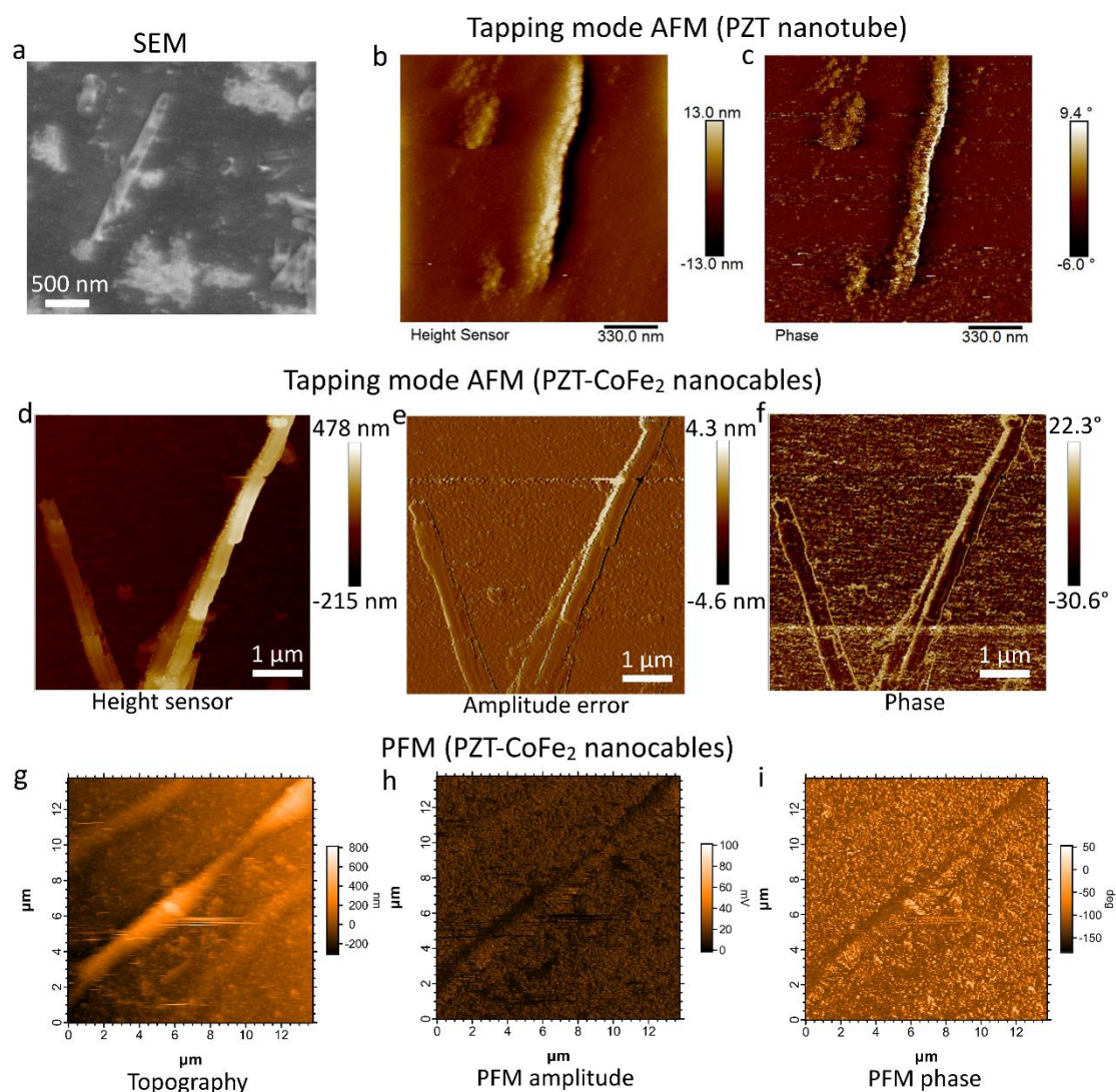
Figure 4.12: (a) HRSEM images of the three-layer PZT 500 nanotube collected on the platinized Si substrate after AAO membrane dissolution. Tapping mode AFM topography (b) and phase (c) images corresponding to the PZT 500 nanotube. Tapping mode AFM topography (d), amplitude error (e), and phase (f) of the PZT 500 -CoFe 2 nanocables. PFM topography (g), amplitude (h), and phase (i) of the PZT 500 -CoFe 2 nanocables.
