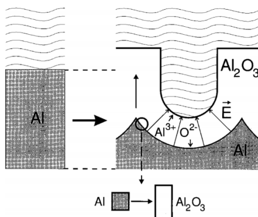
Figure 3.17: Expansion of the alumina during anodic oxidation. On the left the level of the unoxidized metal surface is depicted, reproduced (from Jessensky et al., 1998 )
