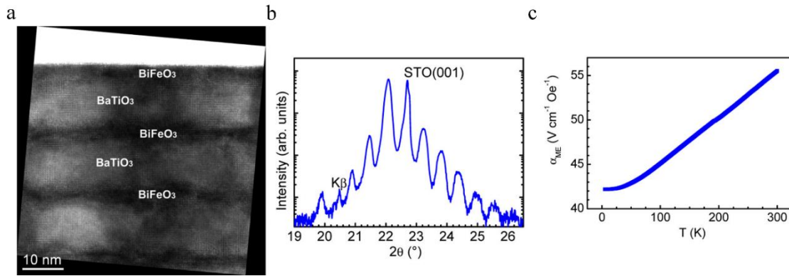
Figure 2.15: (a) HR-TEM image from a cross section of BTO-BFO \times 15 superlattices near a surface; (b) XRD 2\theta - \omega scan with superlattice fringes. (c) Temperature-dependent magnetoelectric coefficient of superlattice BTO-CFO \times 15. From Lorenz et al., 2017
