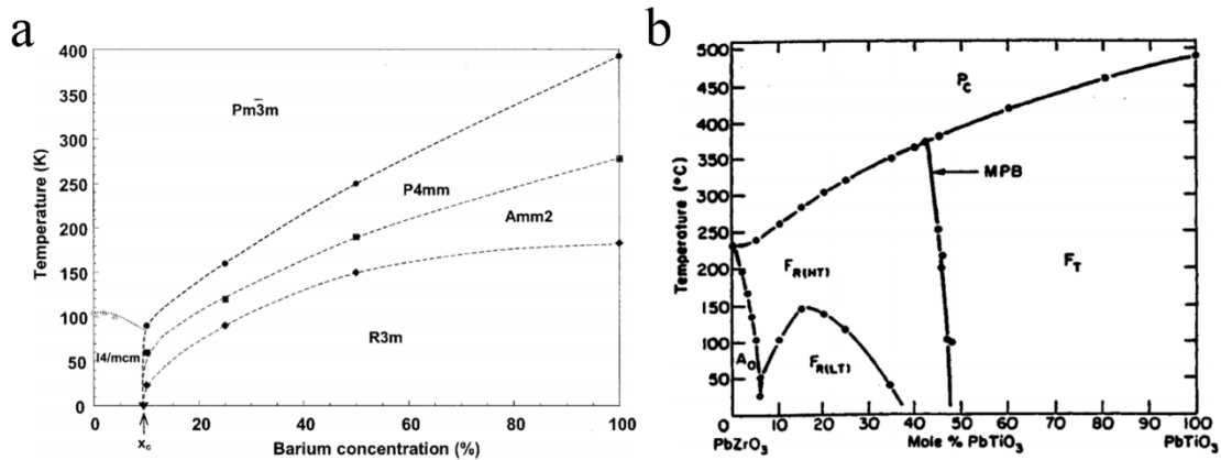
Figure 2.20: (a) Critical temperature vs concentration phase diagram of \text{Sr}_{1-x}\text{Ba}_x\text{TiO}_3 , deduced from x-ray and neutron-diffraction studies (from Menoret et al., 2002 ). (b) PZT phase diagram. From Noheda et al., 1999 , after Jaffe et al., 1971
