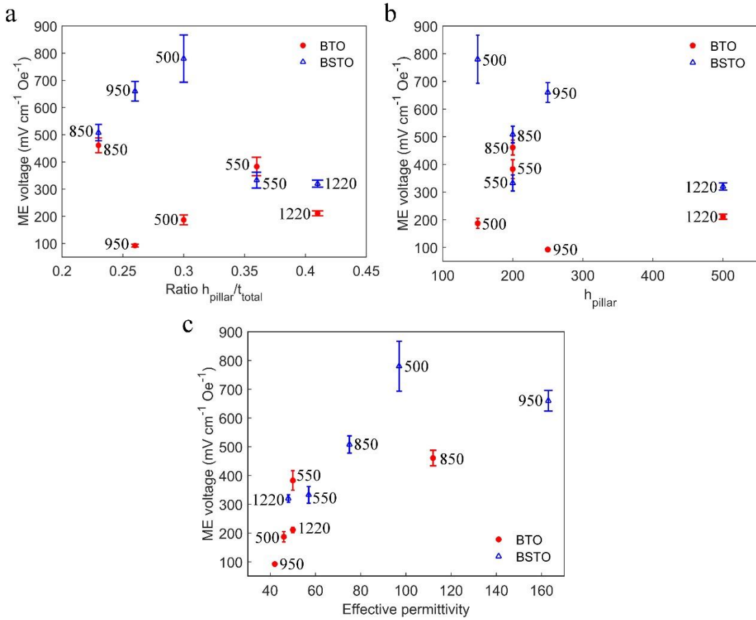
Figure 5.17: Dependence of ME voltage coefficient on (a) ratio between the height of \text{CoFe}_2 nanopillars, h_{\text{pillar}} , and the total thickness of the BSTO and BTO structure, t_{\text{total}} , (b) h_{\text{pillar}} , and (c) effective permittivity of BSTO-CFO and BTO-CFO nanocomposites, estimated from measured capacitance values using Equation (5.2). The numbers indicated next to symbols indicate the total thickness of the BSTO and BTO structure, equivalent to the thickness of BSTO-CFO and BTO-CFO nanocomposites
