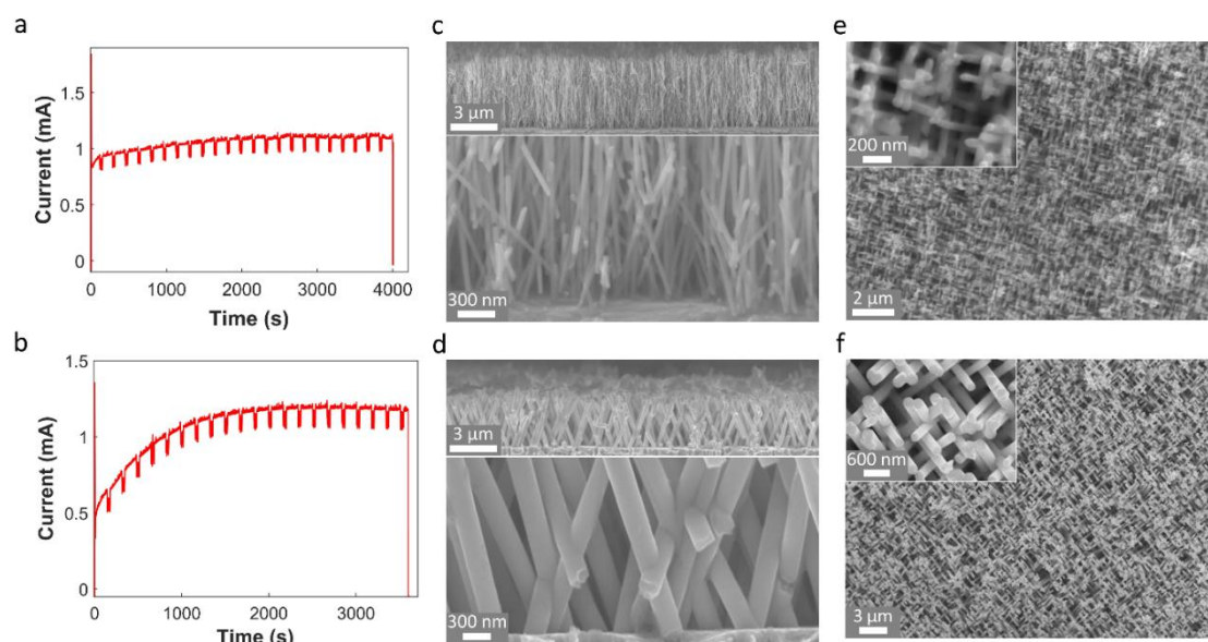
Figure 3.31: (a,b) Cathodic current plots for the electrodeposition of the \text{CoFe}_2 3D nanowire networks with nanowire diameters of \sim 40 and 230 nm, respectively. Tilted cross section view (c,d) and top view (e,f) on the as-deposited 40 nm and 230 nm diameter \text{CoFe}_2 3D NW networks, respectively
