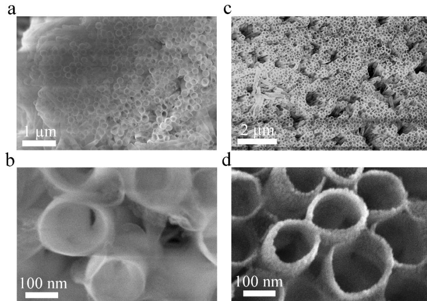
Figure 4.4: HRSEM images of free-standing \text{PZT}^{500} nanotubular structures ( D_{pore} \sim 150 nm, P_{AAO} \sim 35 %) prepared using (a,b) one and (c,d) three consequent sol-gel dip-impregnations in AAO membranes. The PZT nanotubes were collected on the carbon tape after the hosting AAO membrane was dissolved in the concentrated NaOH solution using the AAO dissolution procedure shown in Figure 3.11 , p. 82
