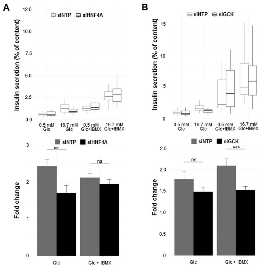
Figure 3: Decreased expression of HNF4A (A) or GCK (B), causing monogenic diabetes, leads to impaired insulin secretion from EndoC- \beta H1 cells. EndoC- \beta H1 cells were transfected with control non-targeting pool siRNA (siNTP) or target gene siRNA and were analyzed 72 h post-transfection. Insulin secretion (percentage of secretion of the total insulin content) was analyzed in response to 60 min incubation with 0.5 mM glucose ( \pm 0.5 mM IBMX), followed by 60 min incubation with 16.7 mM glucose ( \pm 0.5 mM IBMX). Data represent mean values \pm SEM of at least three independent experiments. ** p < 0.01 ; *** p < 0.001 ; ns, not significant. Glc, glucose; IBMX, phosphodiesterase inhibitor 3-isobutyl-1-methylxanthine.
