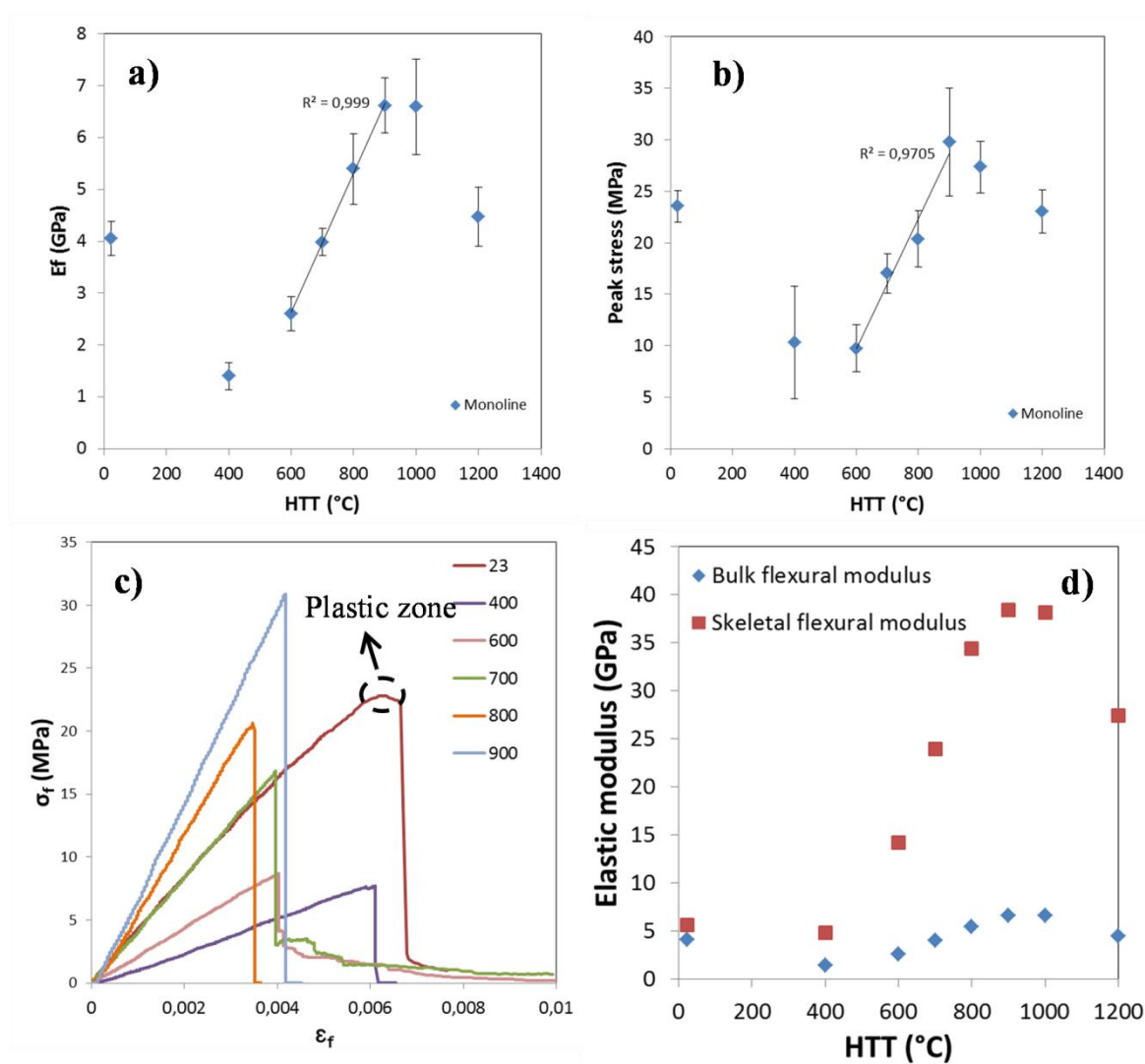
Fig 3.4.9 a) Elastic modulus and b) peak stress of MFC/LS/CP monolines pyrolyzed at different HTTs from 3-point bending tests; c) the flexural stress-strain profile of the samples; d) calculated skeletal elastic modulus with comparison to bulk ones
