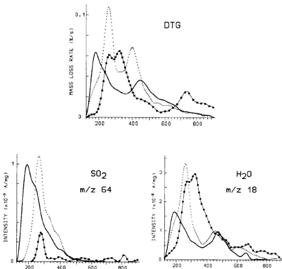
Fig 1.3.3 Comparison of thermal behavior of NaLS \text{---}\blacksquare\text{---} , \text{NH}_4\text{LS} \circ\circ\circ and LS \text{---} : a) DTG curves; b) MS profiles for \text{SO}_2 ; c) MS profiles for \text{H}_2\text{O} (copyright Jakab et al. 1993)
