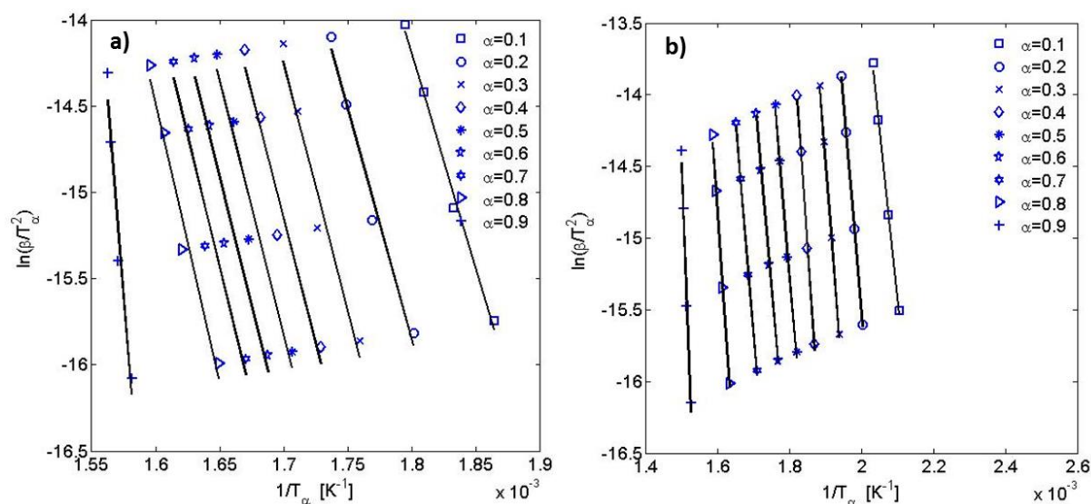
Fig 3.2.7 Arrhenius plot for (a) MFC and (b) LS at conversion levels from 0.1 to 0.9
