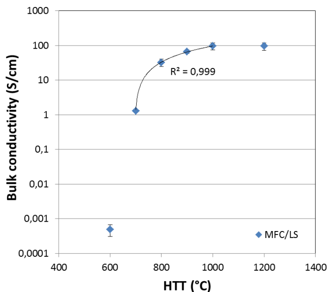
Fig 3.3.4 Evolution of electrical conductivity of chars as a function of HTT
