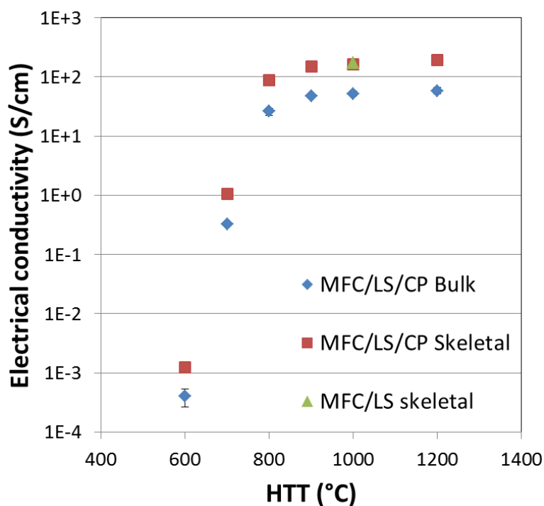
Fig 3.4.8 Bulk and calculated skeletal electrical conductivity of MFC/LS/CP carbons at corresponding HTTs (MFC/LS carbon at 1000°C given for comparison)
