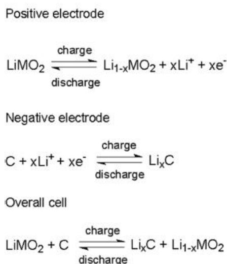
Fig 1.1.13 Reactions in both electrodes and the overall cell during charge-discharge
