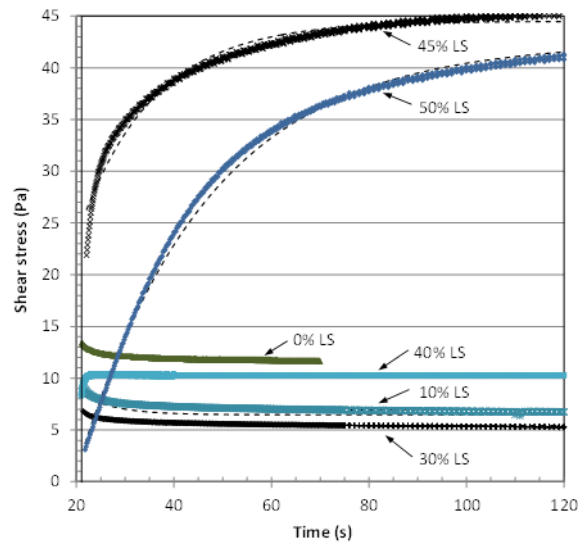
Fig 3.1.6 Shear stress responses to the step-down experiments for the 2% MFC series. The shear rate dropped from 1000 to 0.1 \text{s}^{-1} . Dashed lines represent fits of Eq 3.1.4 to the data.
