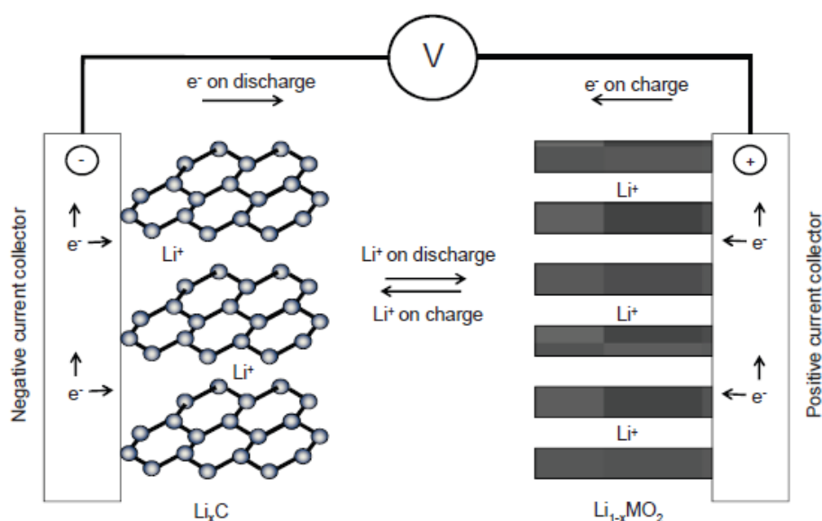
Fig 1.1.12 Charge-discharge process in a LIB cell
