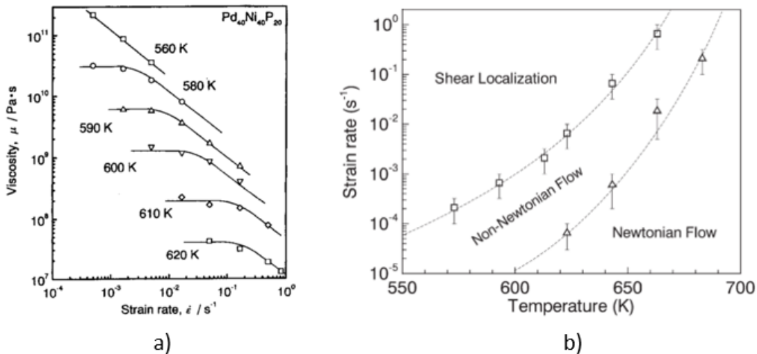
Figure 1.2.2: Viscosity as a function of strain at different temperatures for a Pd 40 Ni 40 P 20 BMG 45 a), Strain modes domains for a Vit1 BMG 43 .
