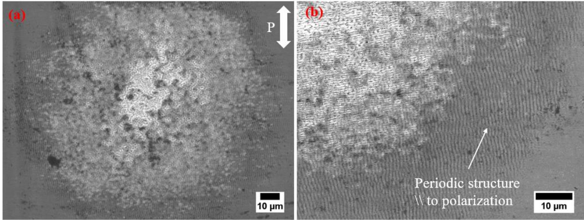
Figure 4.1.10: SEM images of the overall laser spot (a), and zoom on the peripheral part of the spot (b) produced on Zr_{57}Cu_{20}Al_{10}Ni_8Ti_5 BMG at pulse energy E_p = 50\mu J and after N = 200 pulses.
