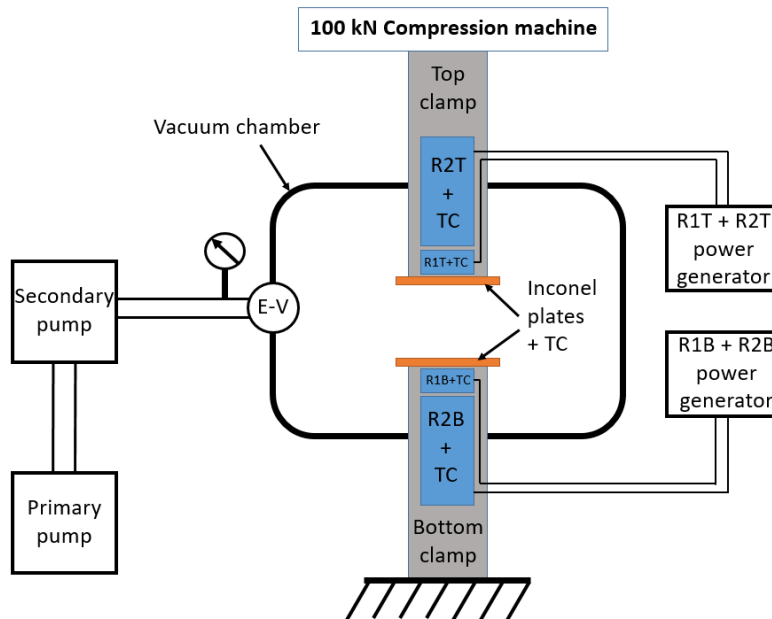
Figure 2.4.4: Comprehensive scheme of the hot compression in-vacuum (HCV) device used to thermoform Zr3 BMG samples.
