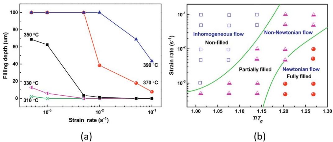
Figure 1.6.2 : Thermomoulding filling depth of metallic glass at various strain rate and temperature in a 50µm width and 100µm depth Si mould (a), flow regimes map of Zr_{35}Ti_{30}Be_{26.75}Cu_{8.25} amorphous alloy with respective filling results (b).
