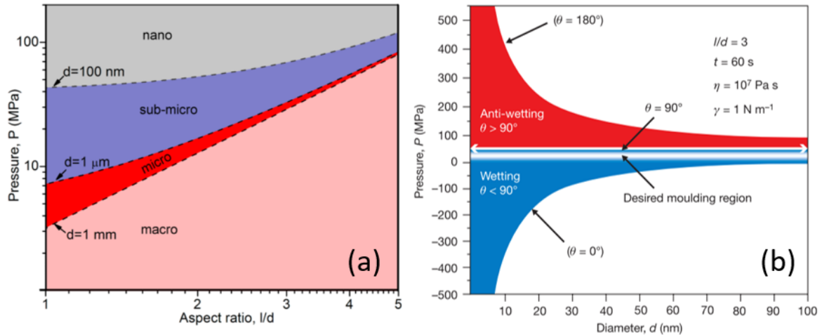
Figure 1.6.1: Required pressure for thermoforming of cylindrical features for different aspect ratios 133 (a), required pressure to fill a channel with a diameter d and an aspect ratio l/d = 3 for both wetting and anti-wetting conditions with a viscous fluid 134 (b).
