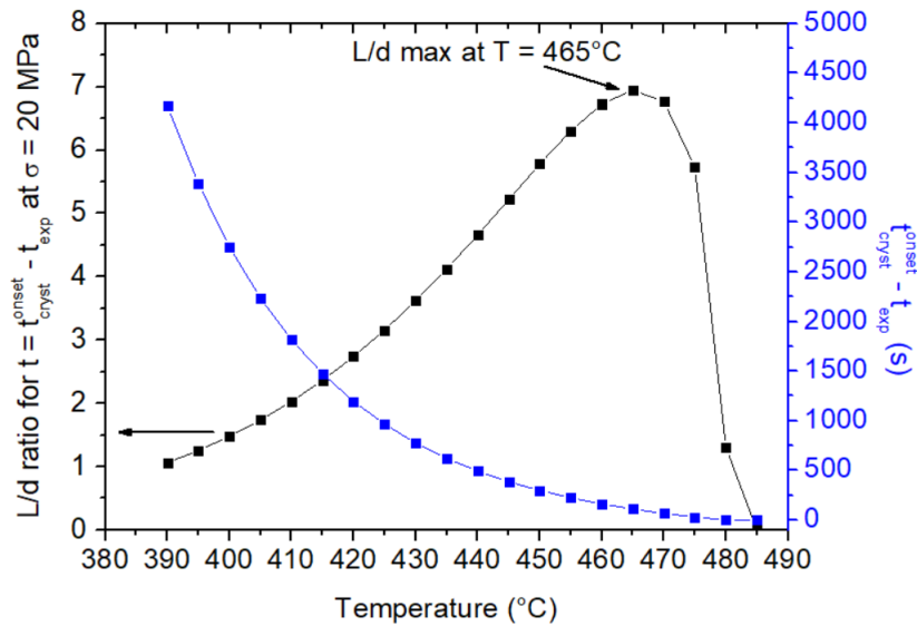
Figure 3.4.7 : Maximum l/d ratios at t = t_{cryst}^{onset} for an applied stress just below the critical stress ( \sigma = 20 MPa) and t_{cryst}^{onset} - t_{exp} as a function of the temperature for Zr3 amorphous alloy.
