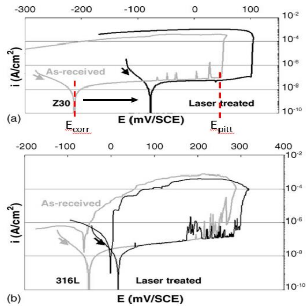
Figure 1.5.19: Cyclic polarization curves for treated and untreated Z30(a) and 316L(b) alloys in Ringer's solution, adapted from 121 .
