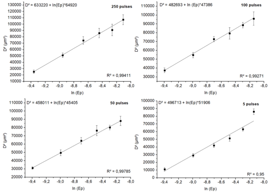
Figure 4.1.3: Plots of D^2 as a function of the pulse energy for 250, 100, 50 and 5 pulses for ZrC alloy. Lines presented are linear fitting of experimental data. R^2 , slopes and intersection values are indicated for every fitting.
