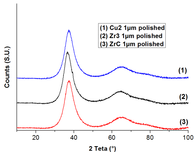
Figure 4.4.1: X-ray diffractograms of untreated Zr3, ZrC and Cu2 1 \mu\text{m} polished metallic glass surfaces.
