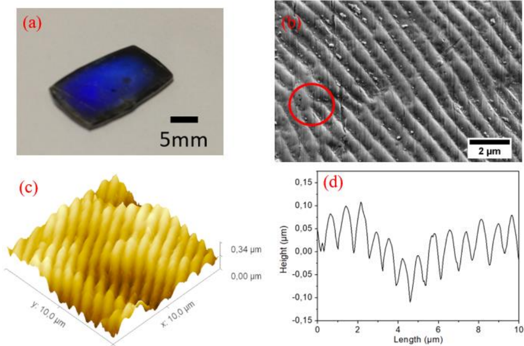
Figure 3.4.11: Picture of a thermoformed Zr3 plate (a), tilted SEM image (b), AFM image of a 100\mu\text{m}^2 surface (c), and 2D roughness profile on the direction perpendicular to LIPSS orientation (d) for a Zr3 BMG thermoformed at \sigma = \sigma_c = 20 \text{ MPa} and T = 400^{\circ}\text{C} .
