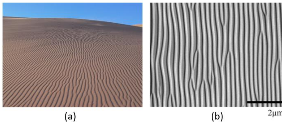
Figure 1.5.13: Ripples formed on sand (a), LIPSS (LSFLs) observed on CaF 2 substrate with Ti:Sapphire source of around 800 nm wavelength 92 .
