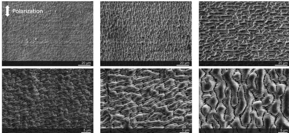
Figure 1.5.21: SEM image of Zr_{62.5}Cu_{22.5}Fe_5Al_{10} (at. %) BMG after fs laser treatment of pulse width \tau = 410 fs and increasing fluence F from 0.103 \text{ J/cm}^2 (upper left) to 0.206 \text{ J/cm}^2 (bottom right), adapted from 17 .
