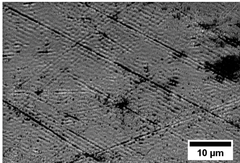
Figure 4.1.9: SEM image of \text{Zr}_{65}\text{Cu}_{15}\text{Al}_{10}\text{Ni}_{10} metallic glass surface irradiated with \phi_a = 0.16 \text{ J/cm}^2 after 1 pulse.
