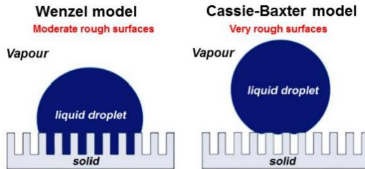
Figure 1.3.1 : Scheme of the Wenzel (left) and Cassie-Baxter (right) models. The different behaviours of a liquid droplet are represented where the liquid completely wets the surface (Wenzel) or the air is trapped within the surface structure (Cassie-Baxter) adapted from 47 .
