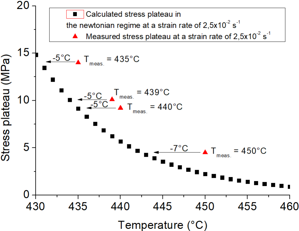
Figure 3.4.1: Graph of the theoretical and measured stress plateau evolution as a function of the temperature at a strain rate of 2.5 \times 10^{-2} \text{ s}^{-1} with Zr3 amorphous alloy.
