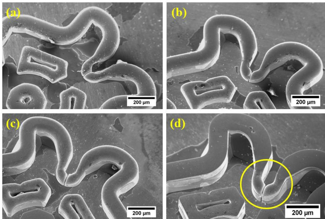
Figure 3.4.3: Tilted SEM images of the reproduced watch micro-piece on BMG after experiments under 420°C and 20 MPa during 30 s (a), 60 s (b), 120 s (c) and 300 s (d) compression time.
