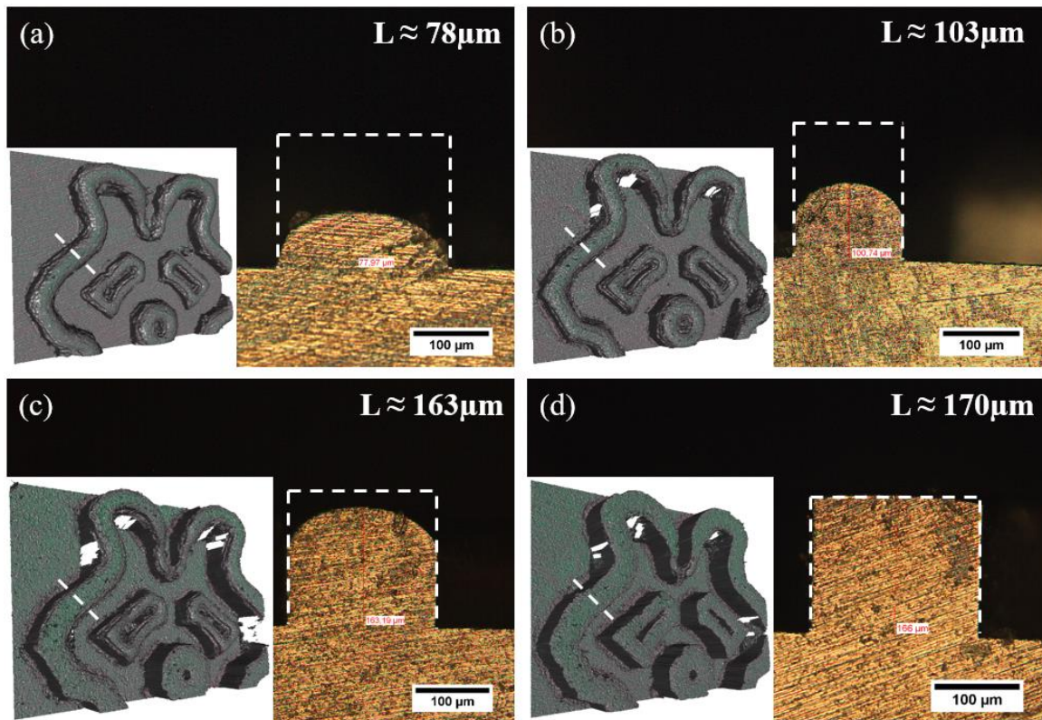
Figure 3.4.2: Microscope images of thermoformed BMG plates cross sections and stereoscopic imprint reconstructions of hot compression tests conducted at 420°C under constant stress of 20 MPa during 30 s (a), 60 s (b), 120 s (c) and 300 s (d) compression time.
