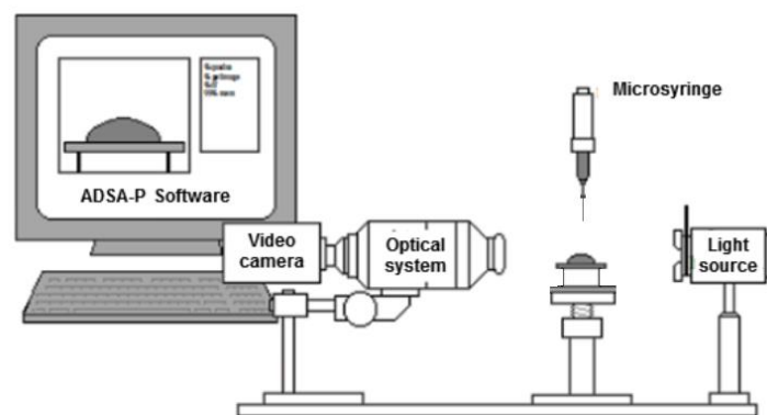
Figure 2.7.1: Scheme of the experimental setup for contact angle measurement, adapted from 47 .
