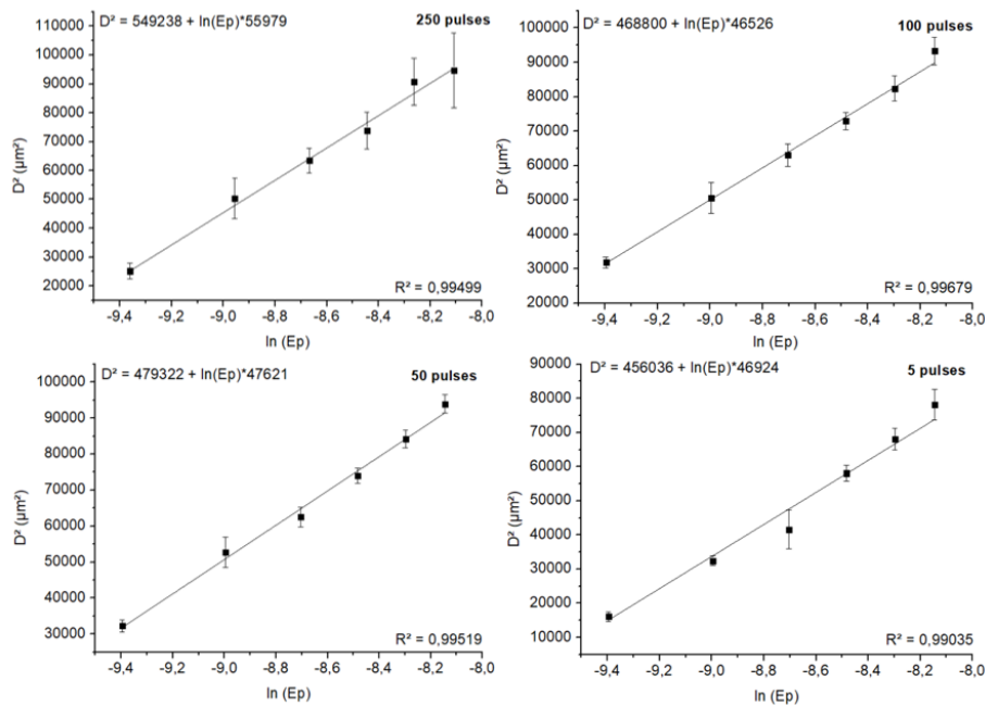
Figure 4.1.2: Plots of D^2 as a function of the pulse energy for 250, 100, 50 and 5 pulses for Zr3 alloy. Lines presented are linear fitting of experimental data. R^2 , slopes and intersection values are indicated for every fitting.
