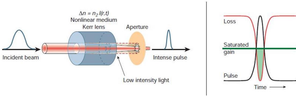
Figure 1.5.5: Kerr lens mode-locking phenomenon. The refractive index of the Kerr lens increases with the laser beam intensity as \Delta n = n_2 I(r, t) , where n_2 is the nonlinear refractive index of the amplifier medium and I(r, t) the radial and time-dependent intensity of a short-pulsed laser beam 64 .
