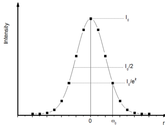
Figure 2.3.4 : Drawing of the Gaussian intensity profile of the laser device used in this thesis work.
