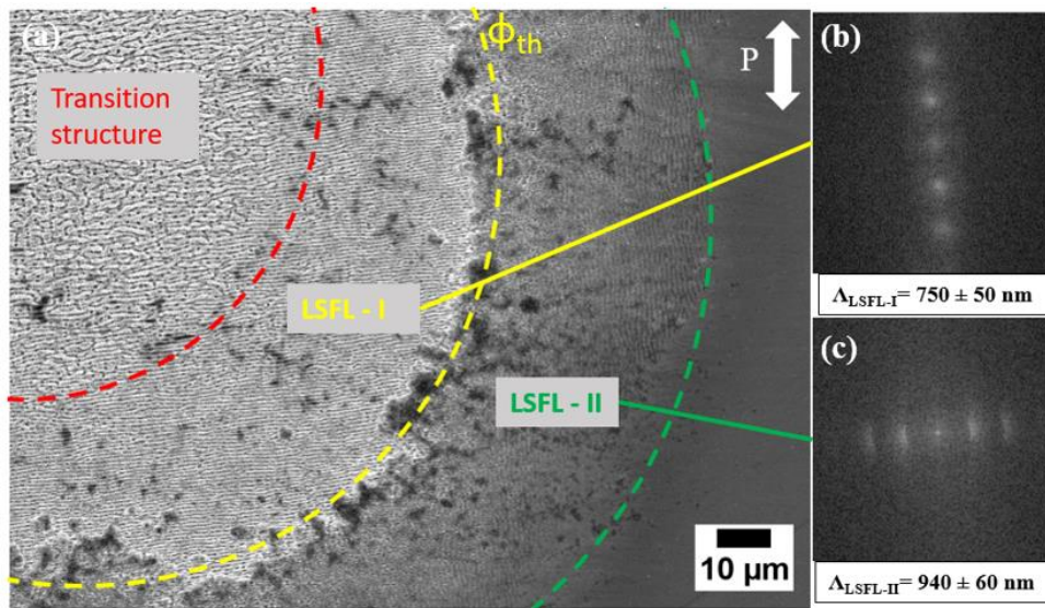
Figure 4.1.12: SEM images of a laser spot produced on a ZrC BMG surface with pulse energy of E_p = 100 \mu\text{J} and N = 150 pulses with the corresponding structures areas and the ablation threshold \phi_{th} zone (a), FFT images of type-I (b) and type-II (c) with corresponded period values.
