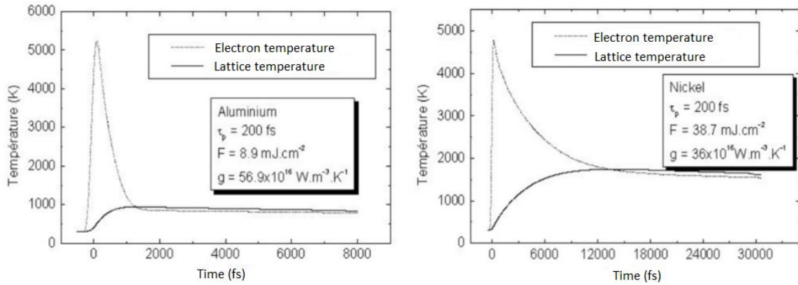
Figure 1.5.10: Two Temperatures Model resolved for a 200 fs laser pulse on aluminium (left) and nickel (right) targets for different fluencies, from Valette thesis 75 .
