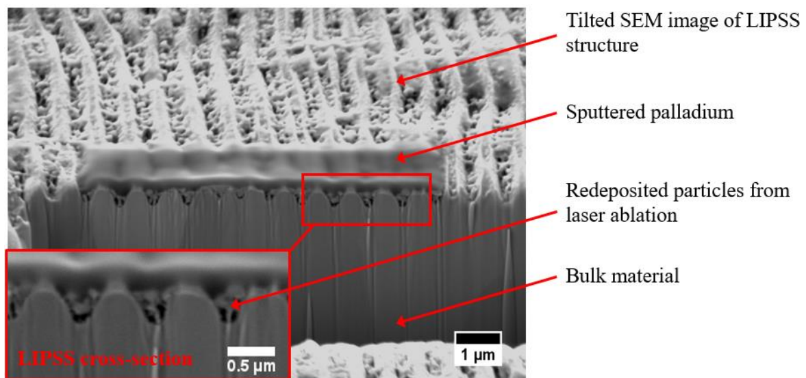
Figure 3.4.13: Tilted SEM image and FIB cross section SEM image of LIPSS structure created on tungsten mould with femtosecond laser at a pulse energy of 800 \mu\text{J} and other experimental parameters presented in Chap II.
