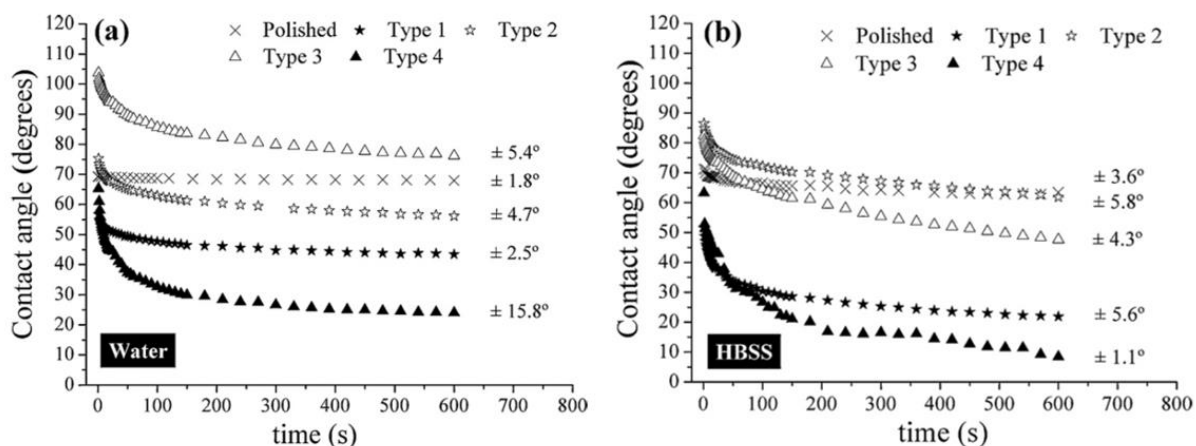
Figure 1.5.17: Contact angle measurements for polished and laser-treated surfaces with water (a) and HBSS solution (b). Type 1 structure corresponding to LIPSS, type 2 to nanopillars, type 3 to columnar structure and type 4 to double scale columnar structure. Adapted from 114 .
