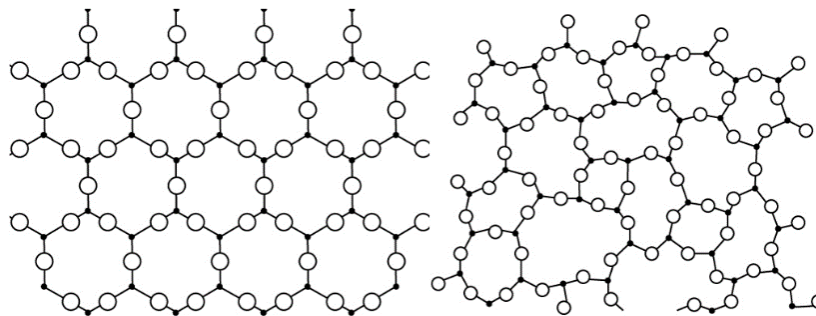
Figure 1.1.1: Silica in crystalline (a) and amorphous (b) state, 2D analogy 23 .
