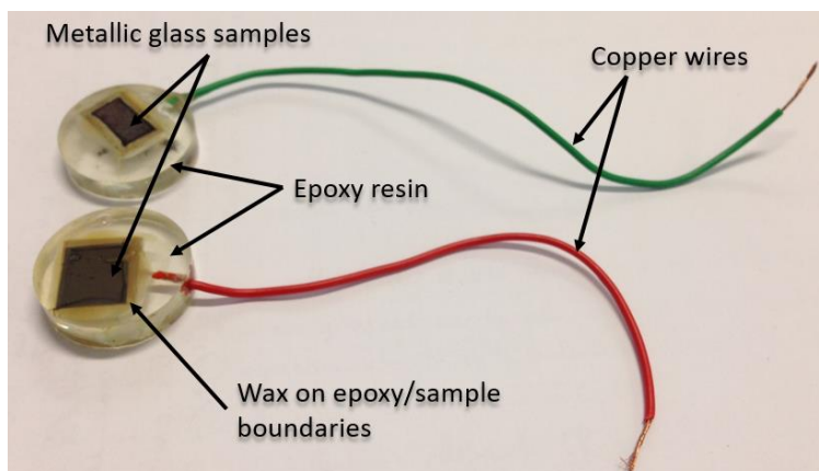
Figure 2.7.2: Picture of prepared metallic glass samples for electrochemical measurements.
