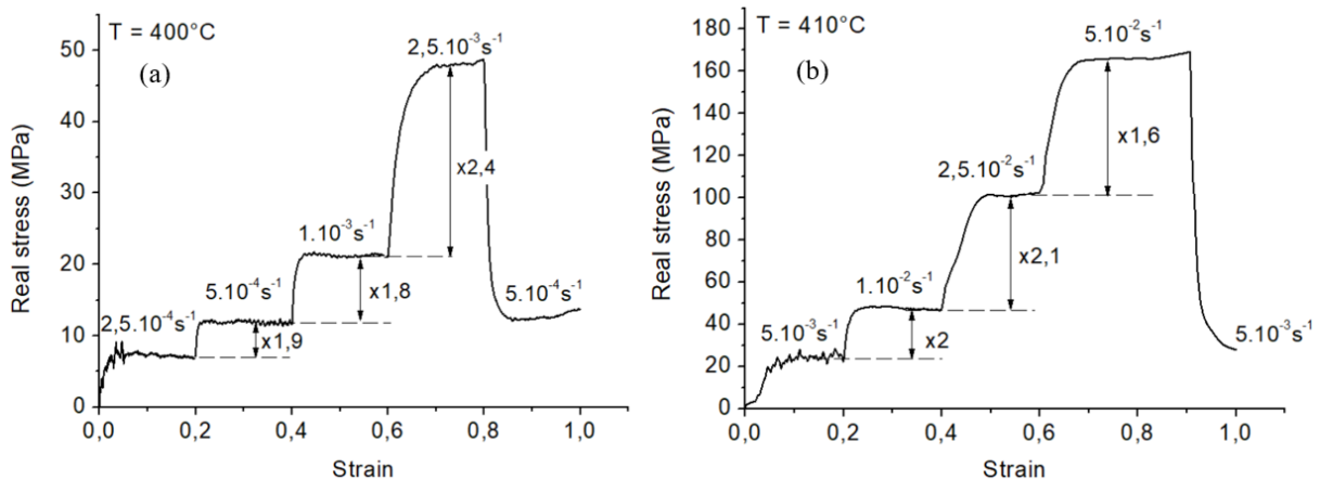
Figure 3.2.4: Curve of strain rate jump test realized at 400^\circ\text{C} on Zr3 rods in the strain range of 2.5 \times 10^{-4} \text{ s}^{-1} to 2.5 \times 10^{-3} \text{ s}^{-1} (a), strain rate jump test curve realized at 410^\circ\text{C} in the strain range of 5 \times 10^{-3} \text{ s}^{-1} to 5 \times 10^{-2} \text{ s}^{-1} (b).
