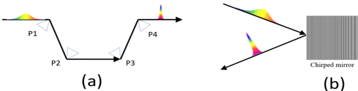
Figure 1.5.6: Dispersion-Compensating Prism Pairs (DCPP) (a), Semiconductor Saturable Absorber Mirror (SESAM) (b).
