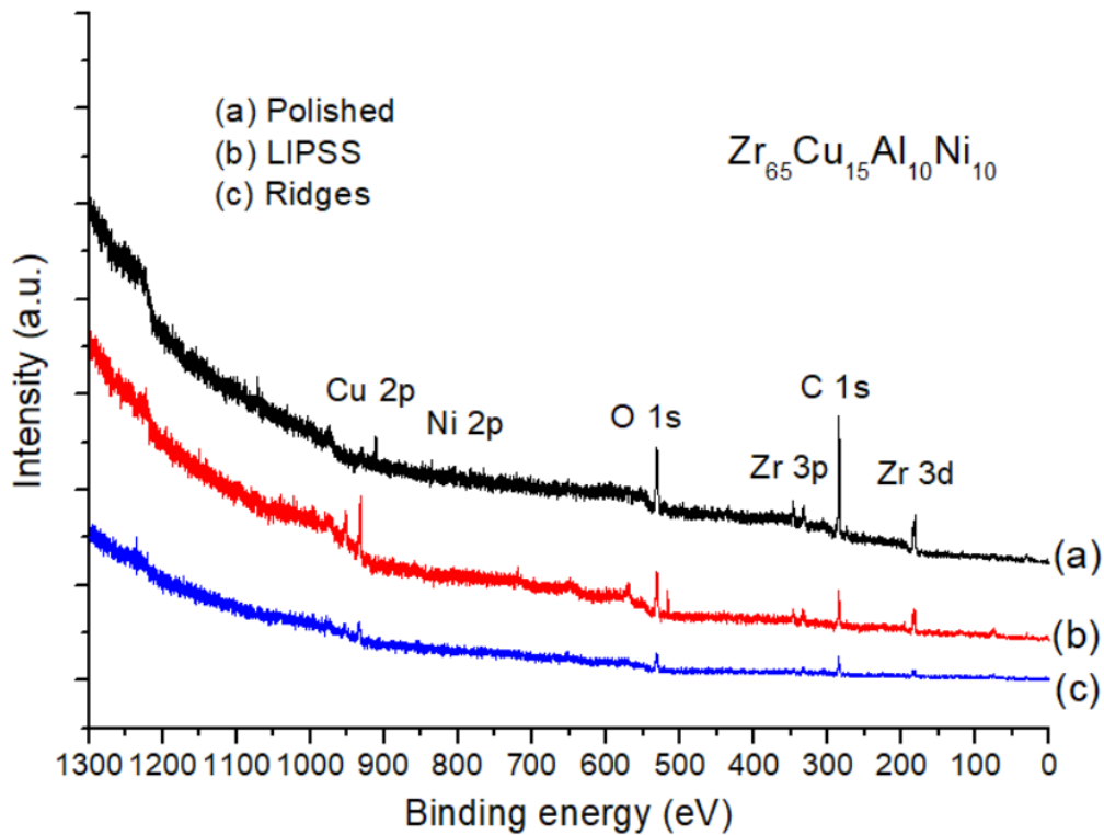
Figure 4.3.1 : XPS survey spectra for 1 \mu\text{m} polished (a), fs-laser treated with LIPSS (b) and ridges (c) textures on Zr 65 Cu 15 Al 10 Ni 10 amorphous alloy surfaces.
