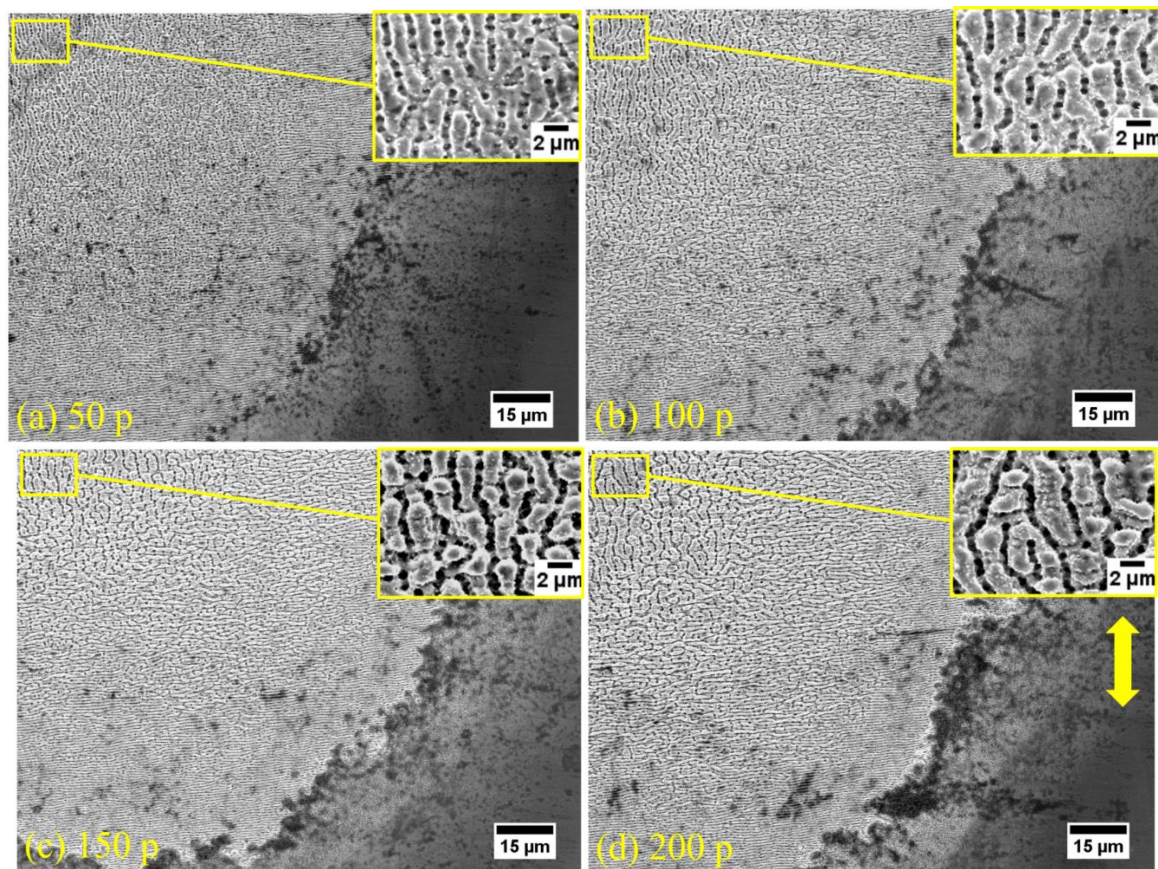
Figure 4.1.7 : Inferior quarters SEM micrographs of different of craters induced by femtosecond laser on a ZrC amorphous alloy with fixed average fluence of 0.18 \text{ J/cm}^2 at a repetition rate of 10 Hz, for 50, 100, 150 and 200 pulses. The yellow arrow indicates the polarization vector of the laser beam. Zoom images were done on the centre of the spot.
