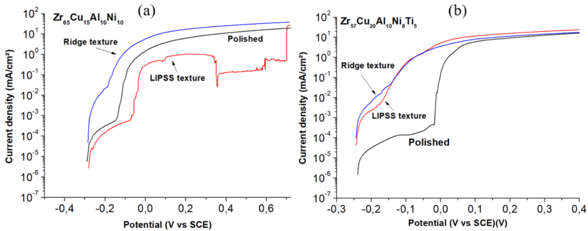
Figure 4.6.3: Anodic polarization measurements on polished, LIPSS texture and RIDGE texture on Zr3 (a) and ZrC (b) amorphous alloy surfaces.
