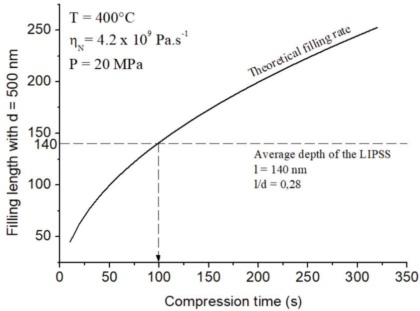
Figure 3.4.10: Theoretical filling length as a function of the time for a temperature of 400°C and an applied pressure of 20 MPa for a d = 500 \text{ nm} width cavity.
