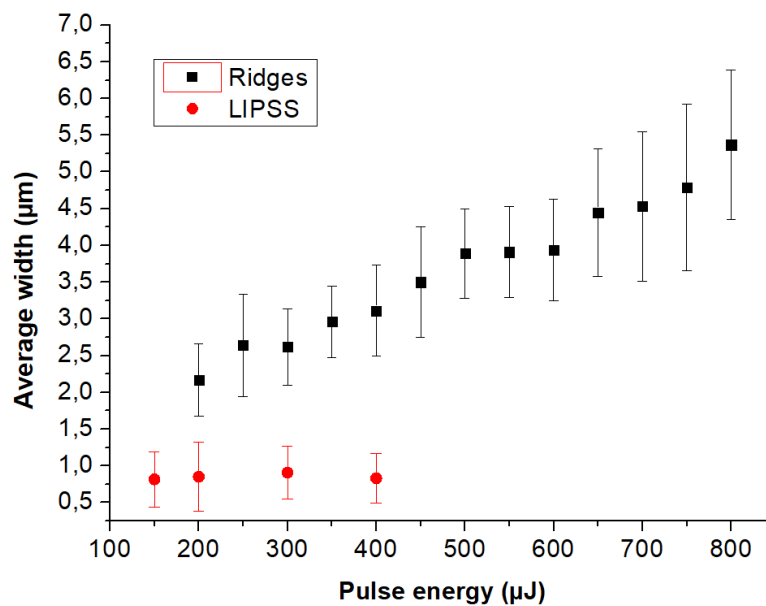
Figure 4.2.5 : Evolution of ridges and LIPSS features width with pulse energy on a Zr3 amorphous alloy surface.
