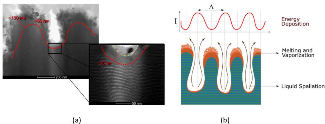
Figure 4.3.3: FIB cross-section of LSFLs on Ti/Ni multilayer substrate irradiated with s-pulse Yb:KYW femtosecond laser of 560 fs pulse duration, wavelength of 1030 nm and pulse energy of 160 \mu J, scheme of the cross section depending on the energy deposition period with ablation mechanisms involved (b) 76 .
