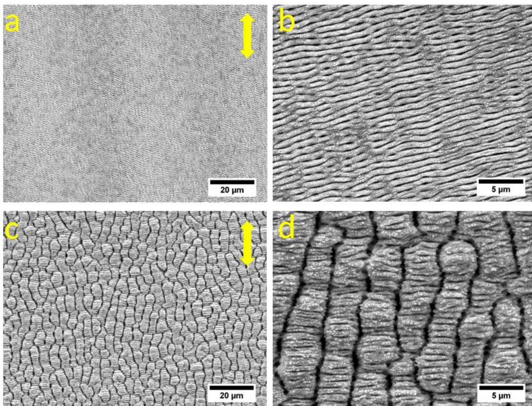
Figure 4.2.2: Low and high magnifications SEM images of LIPSS (a,b) and Ridge (c,d) textures produced on Zr3 amorphous alloy surface. LIPSS (a,b) have been processed with N = 161 and \phi_a = 0.07 J/cm 2 and ridges (c,d) have been processed with N = 538 and 0.4 J/cm 2 . Yellow double arrows represent the laser beam polarization and the scanning orientation.
