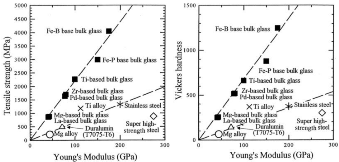
Figure 1.2.1: Relationship between tensile strength ( \sigma_f ), Vickers hardness ( H_v ) and Young's Modulus ( E ) for various bulk amorphous alloys 25 .
