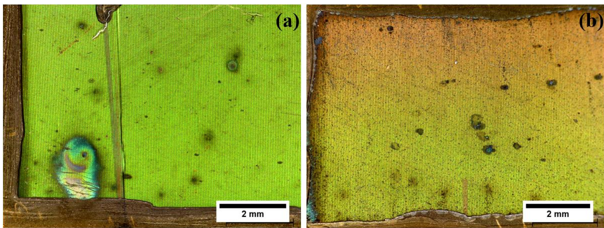
Figure 4.6.4: Optical microscope images of Zr3 (a) and ZrC (b) surfaces textured with LIPSS after anodic polarization measurements.
