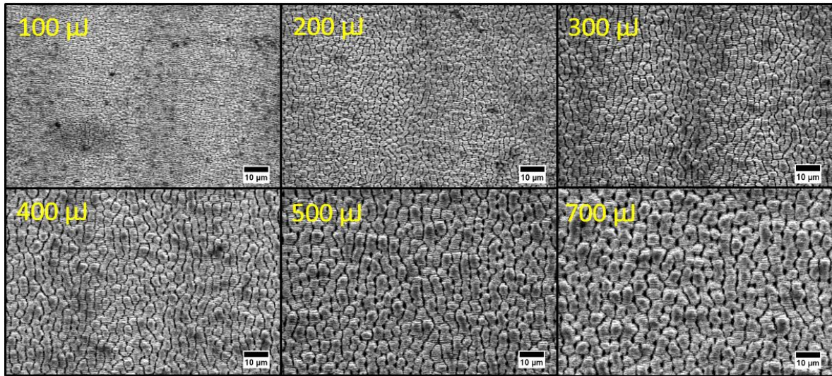
Figure 4.2.4: SEM images of Zr3 alloy textured with ridges processing parameter at 200 Hz with pulse energy of 100, 200, 300, 400, 500 and 700 \mu\text{J} . Scale bar represents 10 \mu\text{m} in length.
