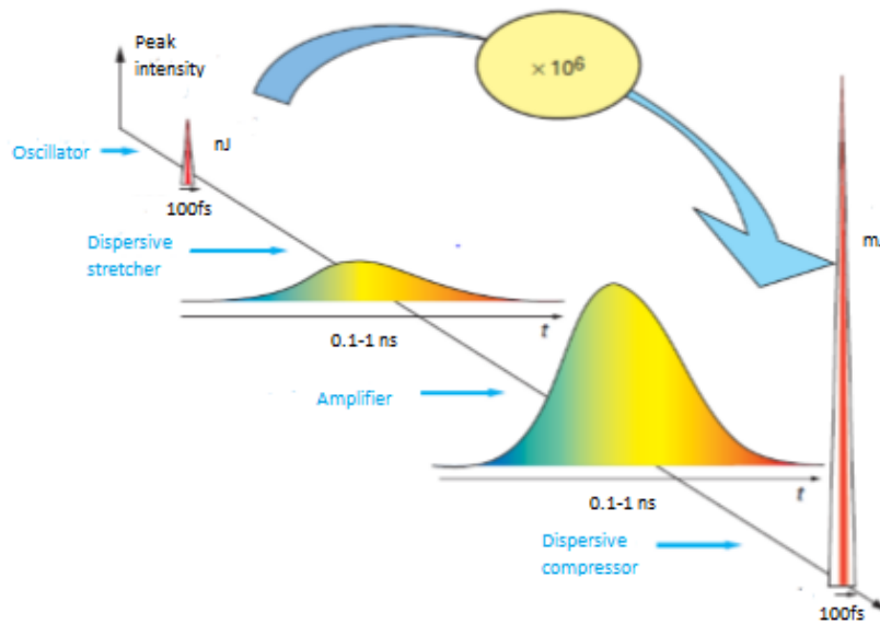
Figure 1.5.8: Scheme of the chirped-pulse amplifier system, adapted from 50 .
