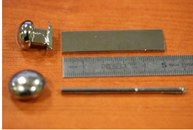
Figure 2.1.2: Zr 65 Cu 15 Al 10 Ni 10 BMG casted in plate and cylindrical shape and the exceeding material removed on the left.
