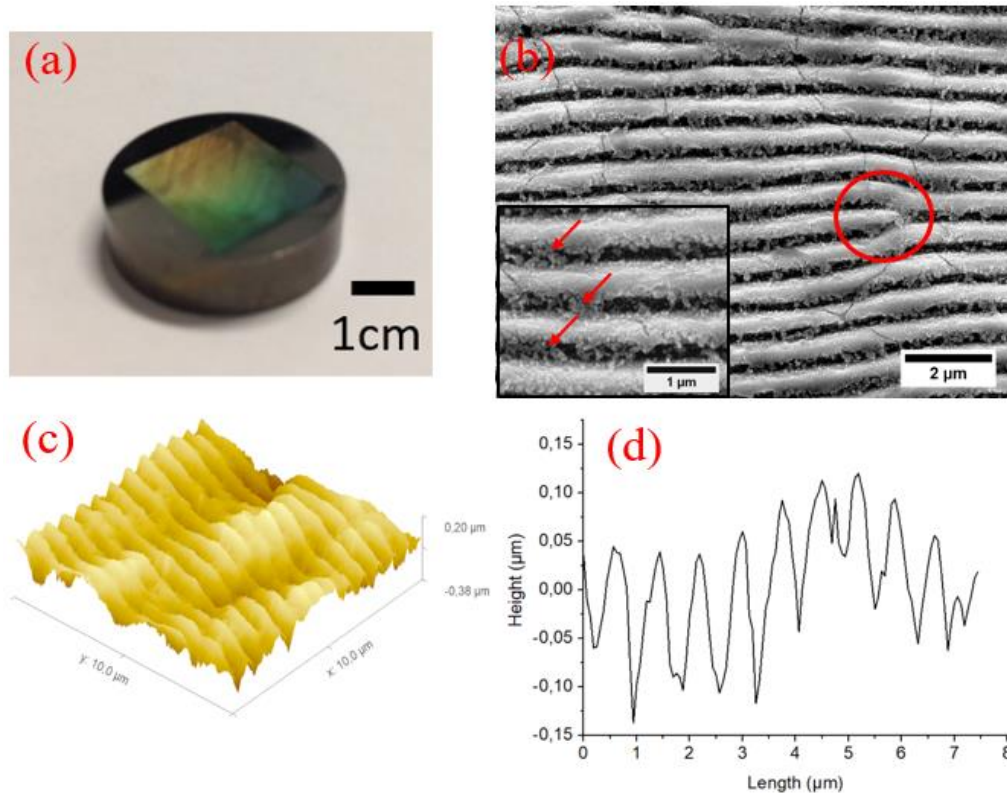
Figure 3.4.9: Picture of a textured tungsten mould with LIPSS (a), SEM image (b), AFM image (c) and 2D roughness profile on the direction perpendicular to the structure orientation (d) of the tungsten cylinder surface textured on a 100mm 2 area with LIPSS produced by femtosecond laser treatment
