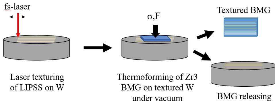
Figure 2.4.8: Scheme of the experimental process for LIPSS replication on Zr3 BMG by thermoforming processing.
