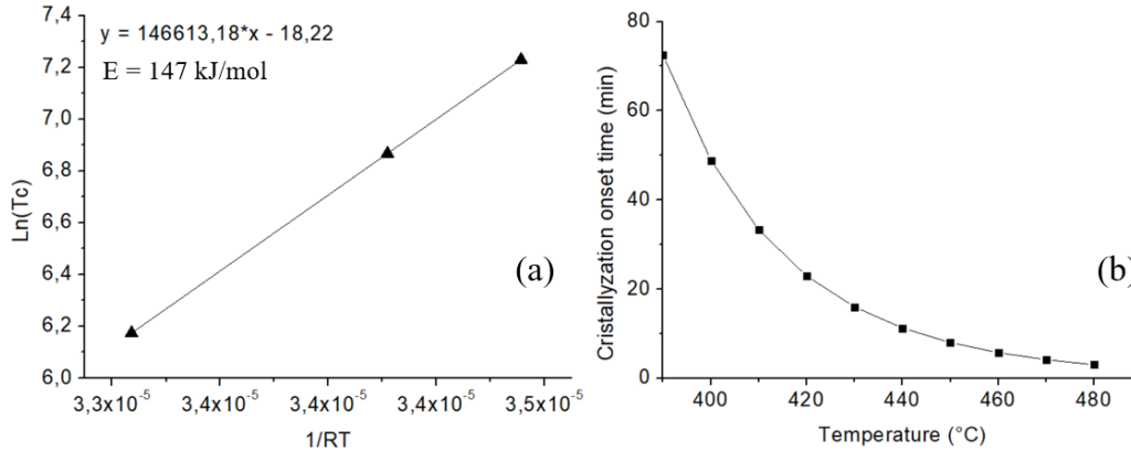
Figure 3.2.3: Plot of \ln(t_c^{onset}) as a function of \frac{1}{RT} in order to determine the crystallization activation energy E of Zr3 (a). Crystallization onset time calculated from the activation energy E for every temperature in the SLR of Zr3 alloy (b).
