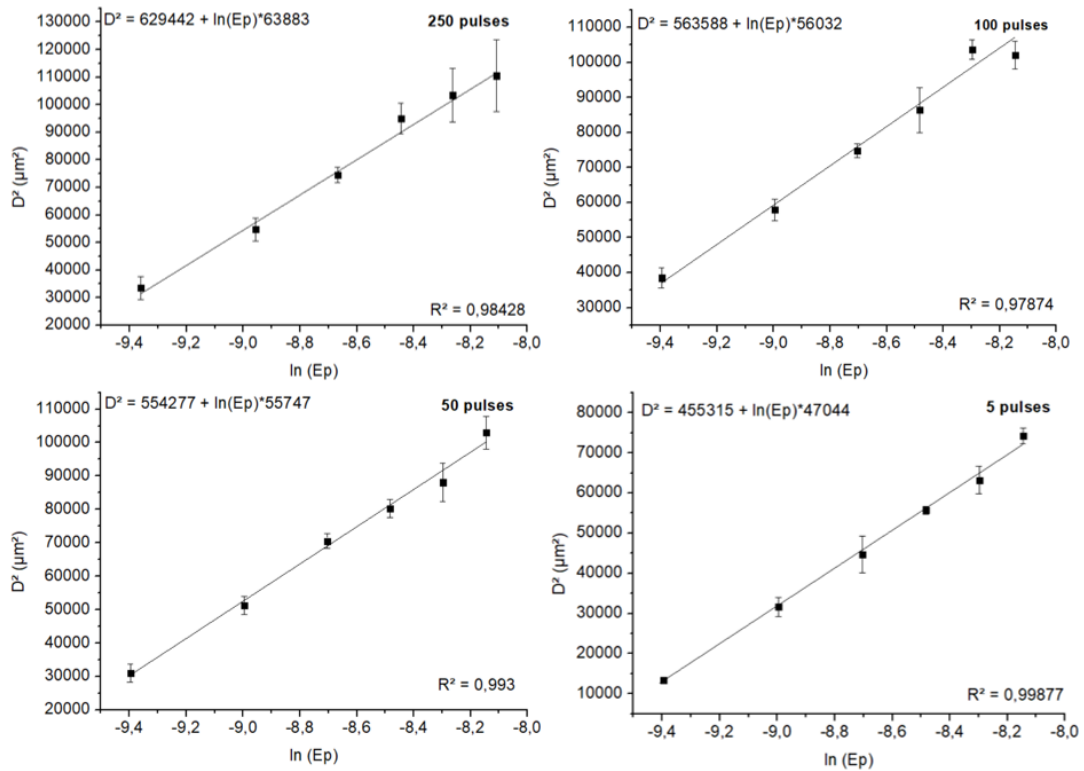
Figure 4.1.4: Plots of D^2 as a function of the pulse energy for 250, 100, 50 and 5 pulses for Cu 2 alloy. Lines presented are linear fitting of experimental data. R^2 , slopes and intersection values are indicated for every fitting.
