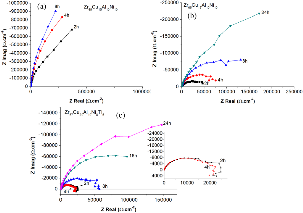
Figure 4.6.5: Nyquist diagrams of LIPSS (a) and Ridge (b) textures on Zr3 alloy and Ridge texture on ZrC alloy (c) made by EIS experiments from 2 h to 24 h of immersion in 0.1 M NaCl.
