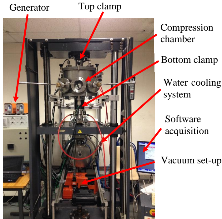
Figure 2.4.3: Picture of the thermoforming device used to pattern Zr_{65}Cu_{15}Al_{10}Ni_{10} alloy.
