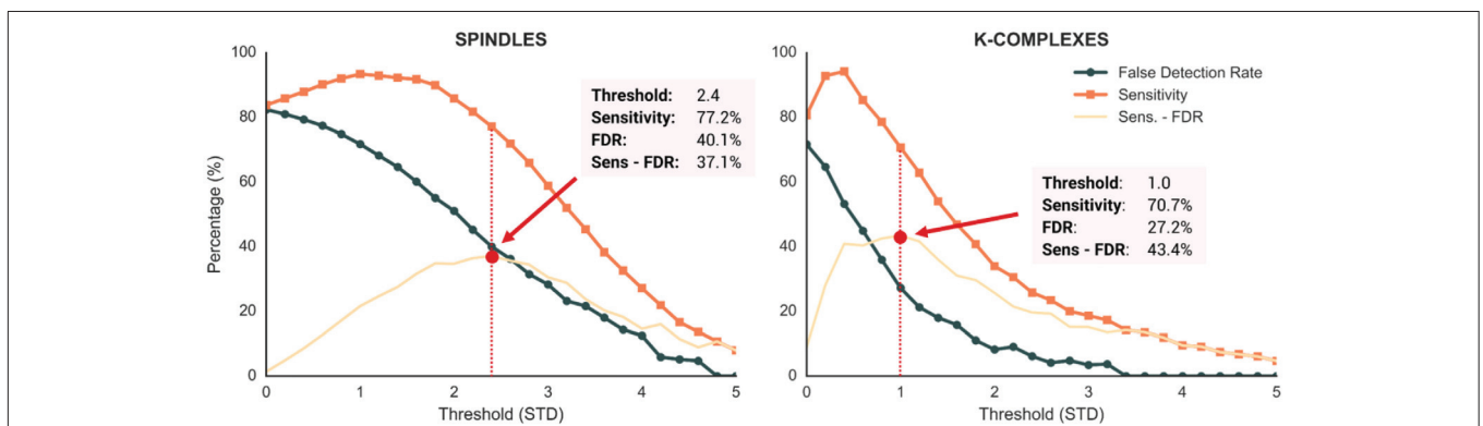
FIGURE 7 | Performance metrics of the Sleep spindle and K-complex detection methods evaluated at 25 different thresholds (range = 0–5, step = 0.2). Dark orange and blue lines depict the sensitivity and false detection rate (FDR), respectively. Light orange lines show the difference between sensitivity and FDR. Red dotted lines depict the threshold values that maximized this difference.
